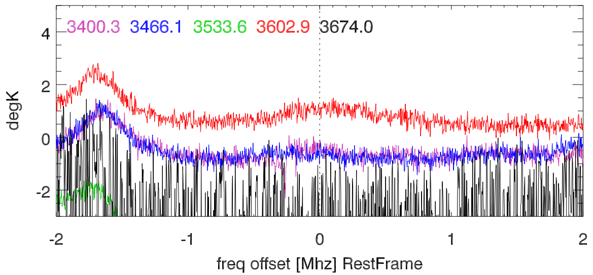
He_beta 3335.7:3689.4 Mhz overplot lineNums
