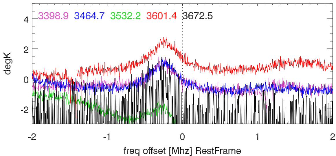
H_beta 3335.7:3689.4 Mhz overplot lineNums
