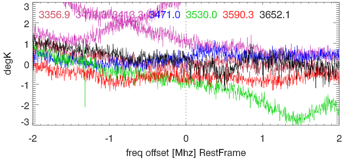
C_gamma 3335.7:3689.4 Mhz overplot lineNums
