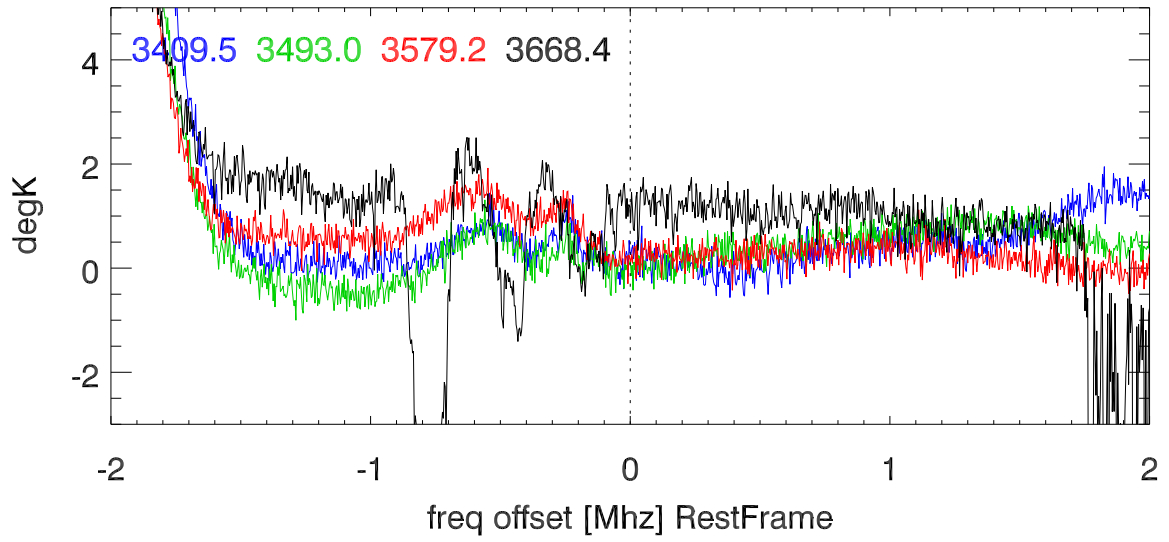
C_alfa 3335.7:3689.4 Mhz overplot lineNums
