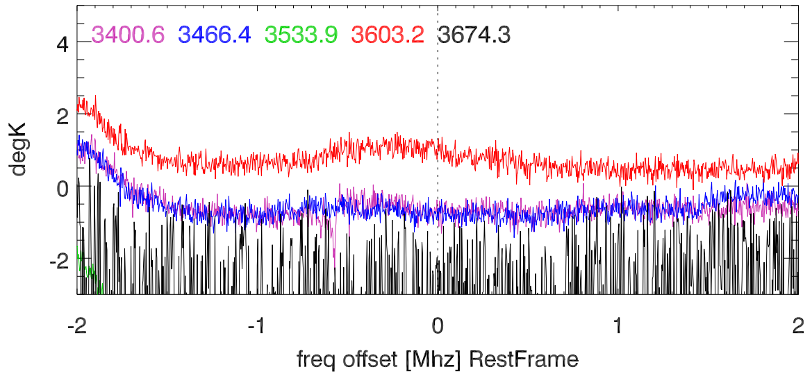
C_beta 3335.7:3689.4 Mhz overplot lineNums
