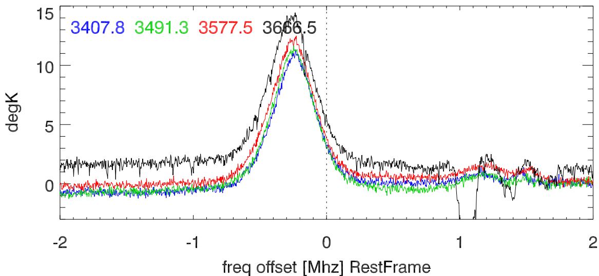
H_alfa 3335.7:3689.4 Mhz overplot lineNums
