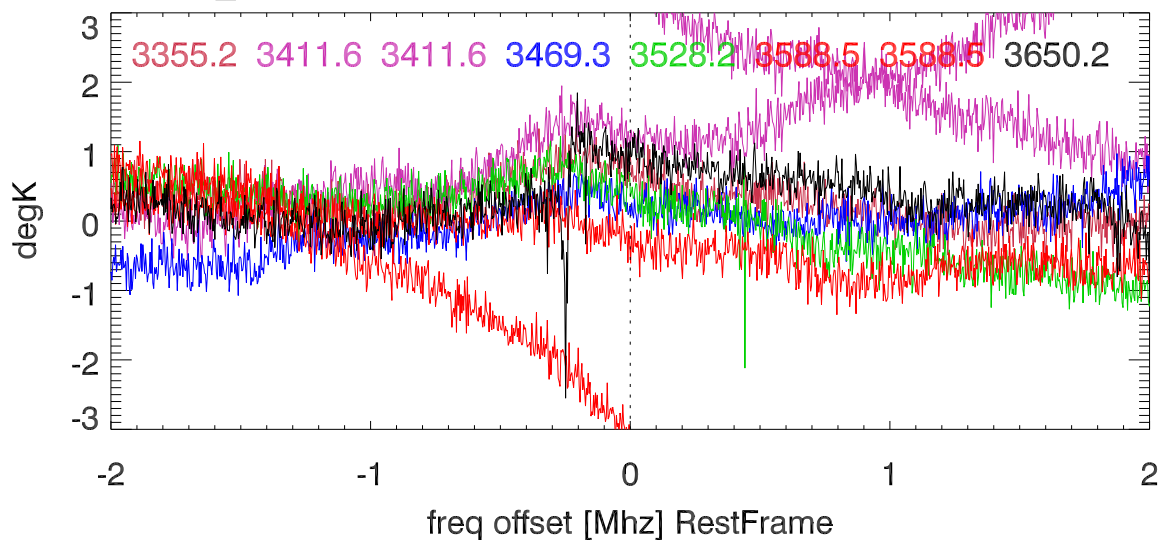
H_gamma 3335.7:3689.4 Mhz overplot lineNums
