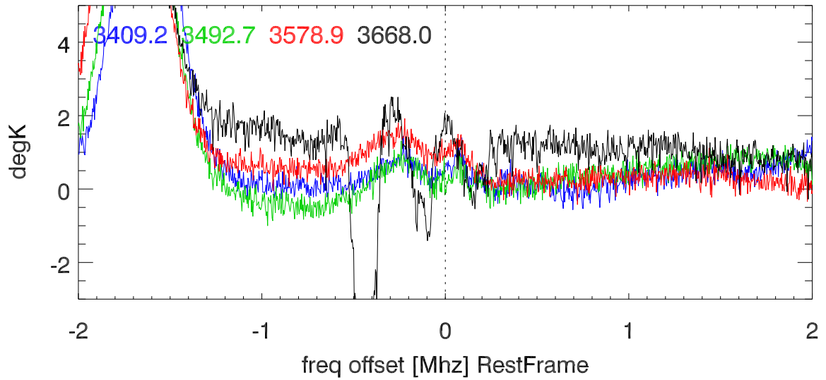
He_alfa 3335.7:3689.4 Mhz overplot lineNums
