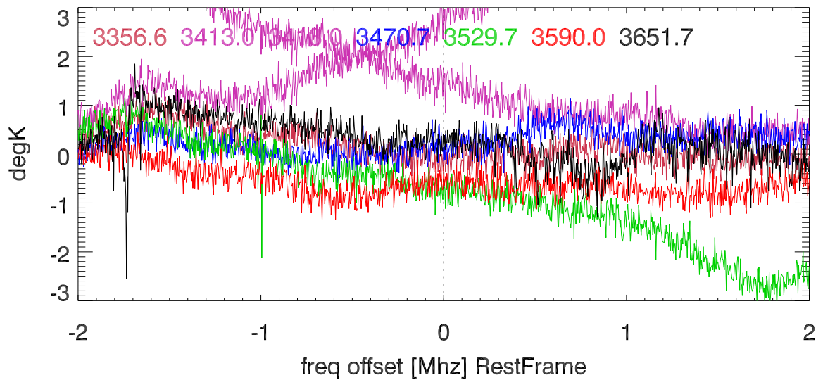
He_gamma 3335.7:3689.4 Mhz overplot lineNums
