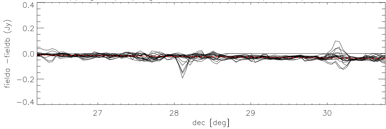
difference overlapping maps (long direction= dec) Cloop:5 Lloop:1 *Field5 - Field14)
