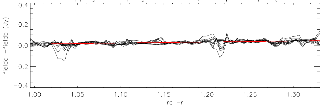
difference overlapping maps (long direction=ra) Cloop:5 Lloop:1 (Field2.05 - Field4.05)
