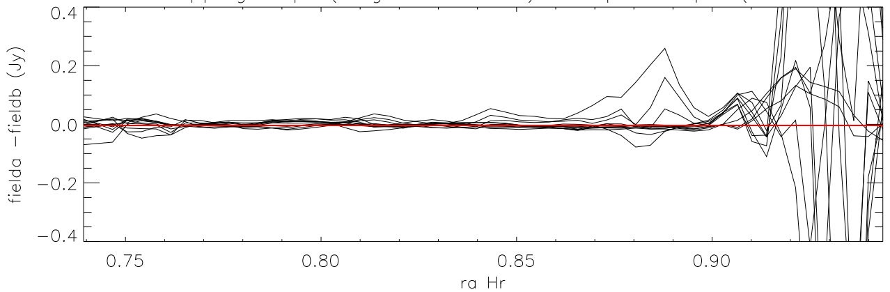
difference overlapping maps (long direction=ra) Cloop:5 Lloop:1 (Field6 - Field1.05)
