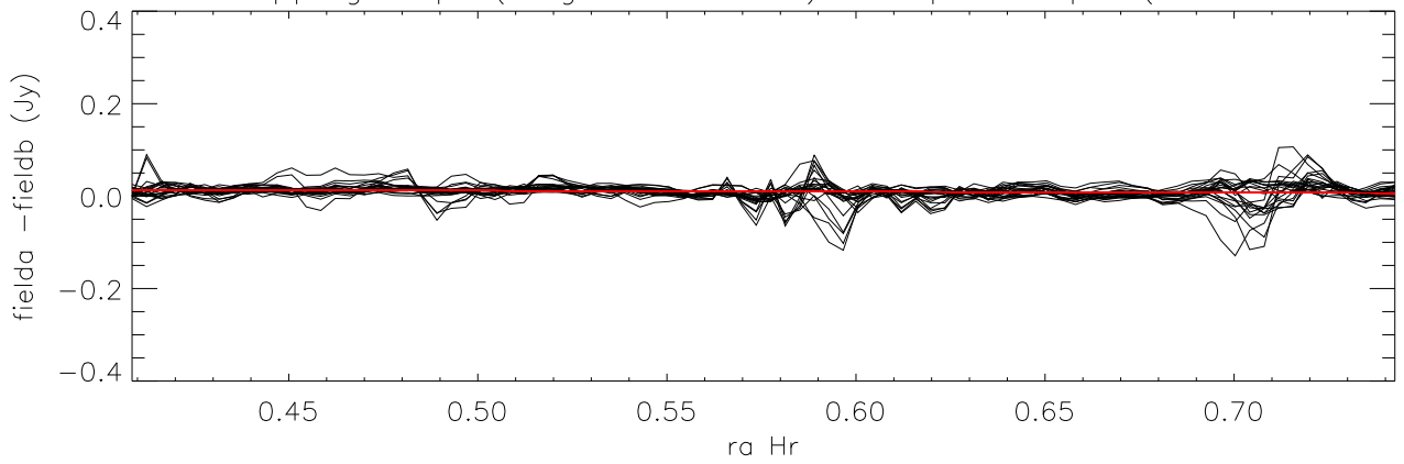
difference overlapping maps (long direction=ra) Cloop:5 Lloop:1 (Field1.05 - Field3.05)
