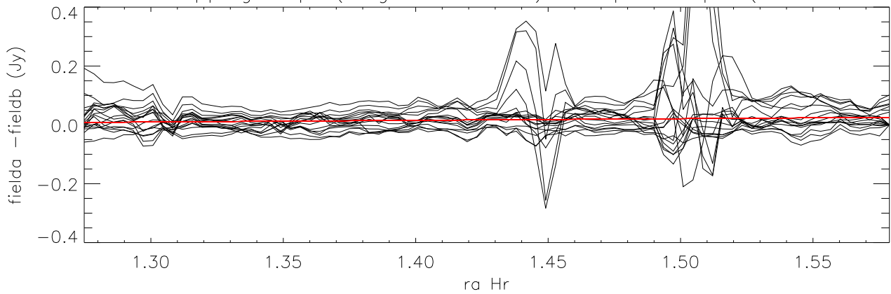
difference overlapping maps (long direction= dec) Cloop:5 Loop:1 *Field1 - Field2)
