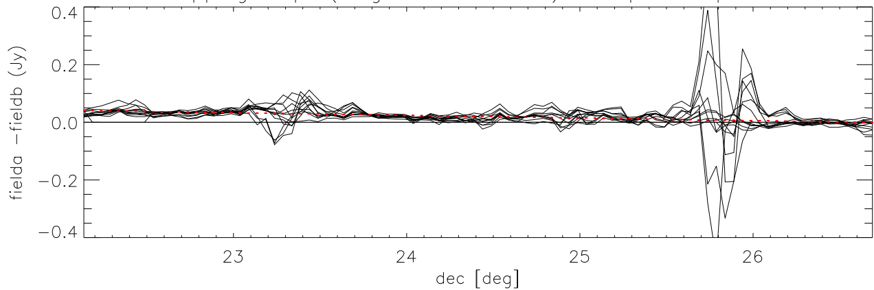
difference overlapping maps (long direction= dec) Cloop:5 Lloop:1 *Field7 - Field6)
