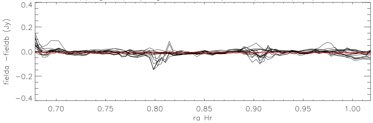
difference overlapping maps (long direction=ra) Cloop:5 Lloop:1 (Field3 - Field2)
