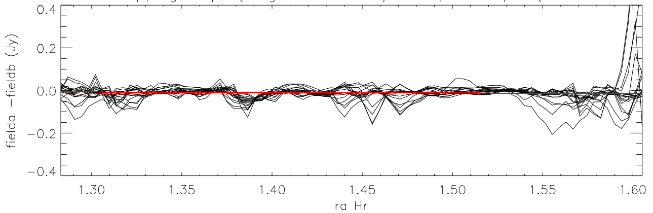
difference overlapping maps (long direction=ra) Cloop:5 Lloop:1 (Field7 - Field2.05)
