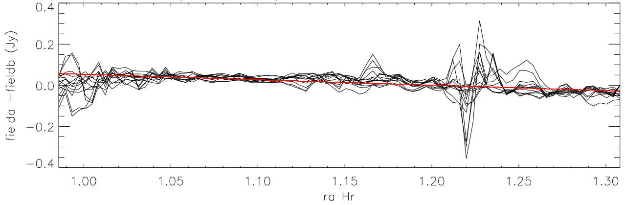
difference overlapping maps (long direction=ra) Cloop:5 Lloop:1 (Field12 - Field11A)
