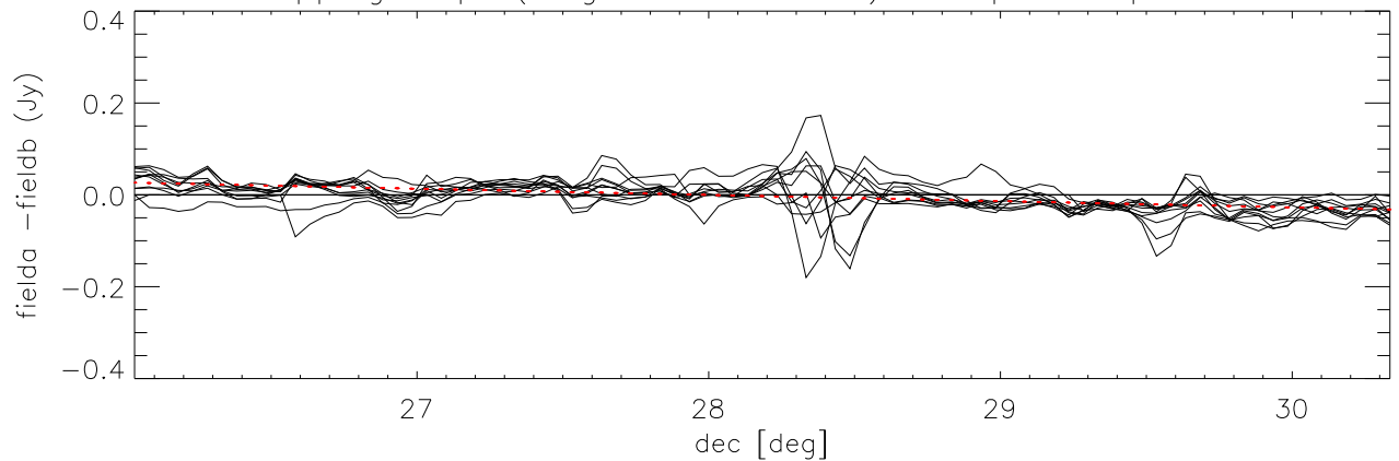
difference overlapping maps (long direction= dec) Cloop:5 Lloop:1 *Field1.05 - Field4)
