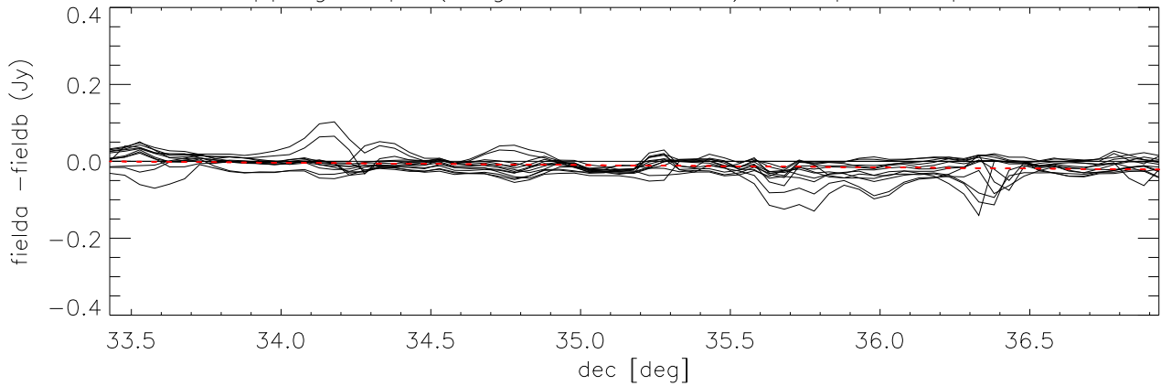
difference overlapping maps (long direction= dec) Cloop:5 Loop:1 *Field3 - Field11A)
