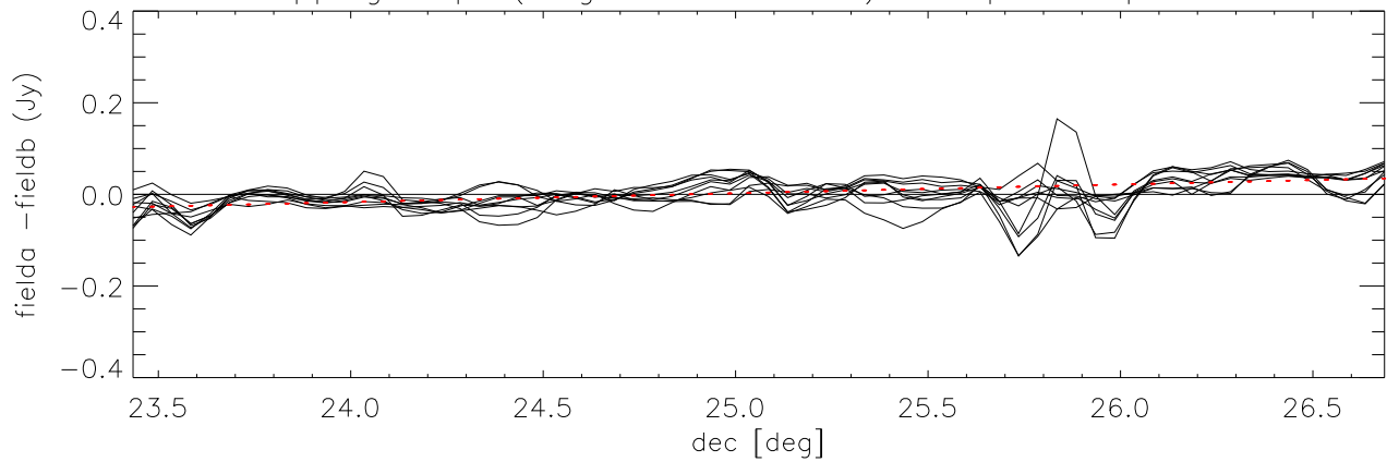
difference overlapping maps (long direction= dec) Cloop:5 Lloop:1 *Field6 - Field5)
