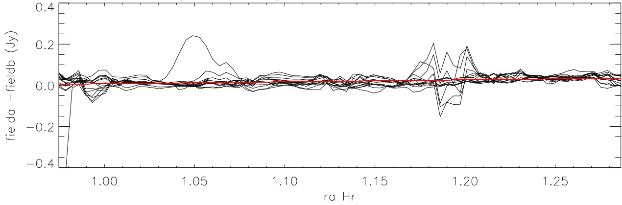
difference overlapping maps (long direction=ra) Cloop:5 Loop:1 (Field14 - Field12)
