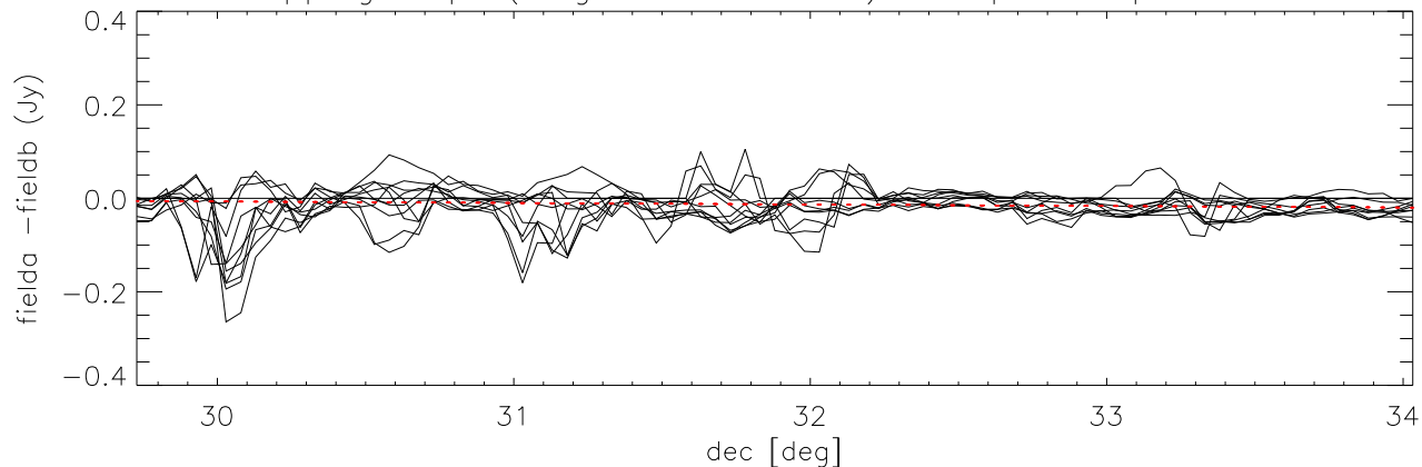
difference overlapping maps (long direction= dec) Cloop:5 Lloop:1 *Field4.05 - Field3.05)
