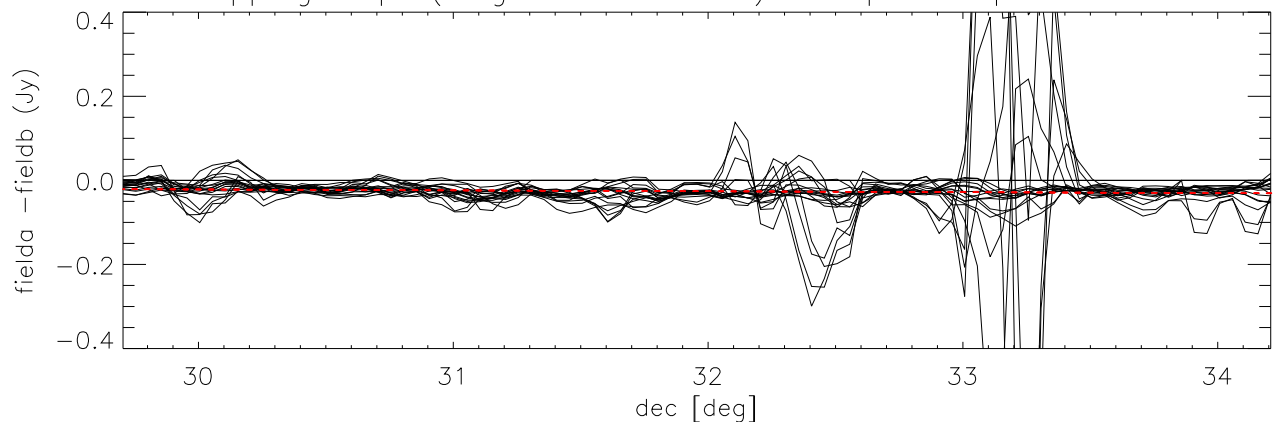
difference overlapping maps (long direction= dec) Cloop:5 Lloop:1 *Field4 - Field12)
