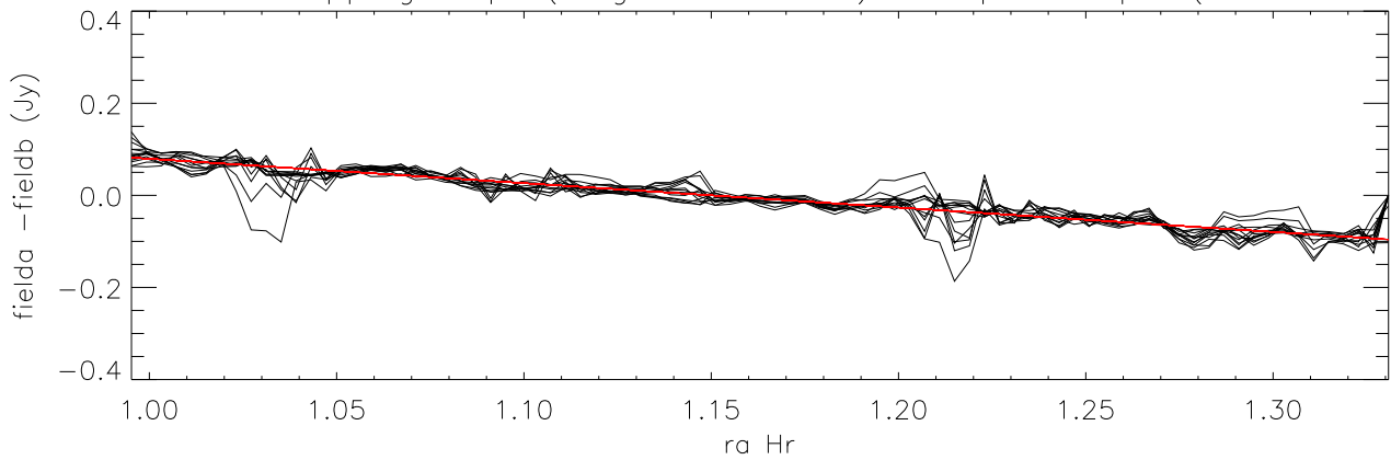
difference overlapping maps (long direction=ra) Cloop:2 Lloop:1 (Field2.05 - Field4.05)
