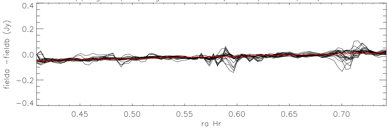
difference overlapping maps (long direction=ra) Cloop:2 Lloop:1 (Field1.05 - Field3.05)
