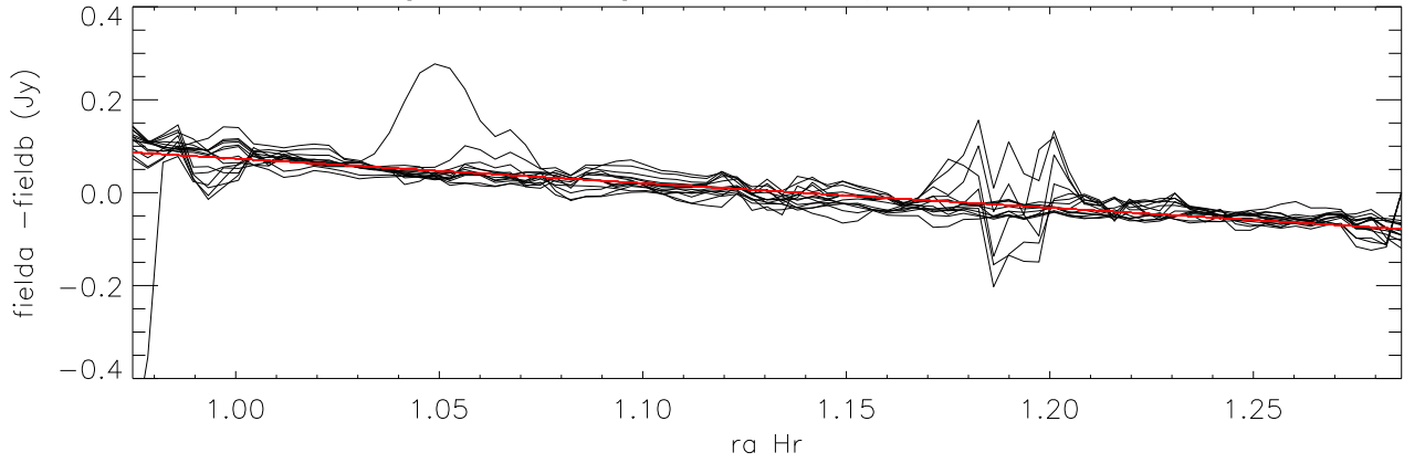
difference overlapping maps (long direction=ra) Cloop:2 Lloop:1 (Field14 - Field12)
