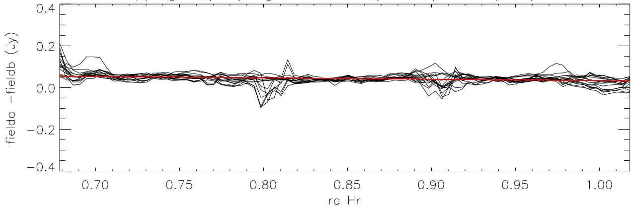
difference overlapping maps (long direction=ra) Cloop:2 Lloop:1 (Field3 - Field2)
