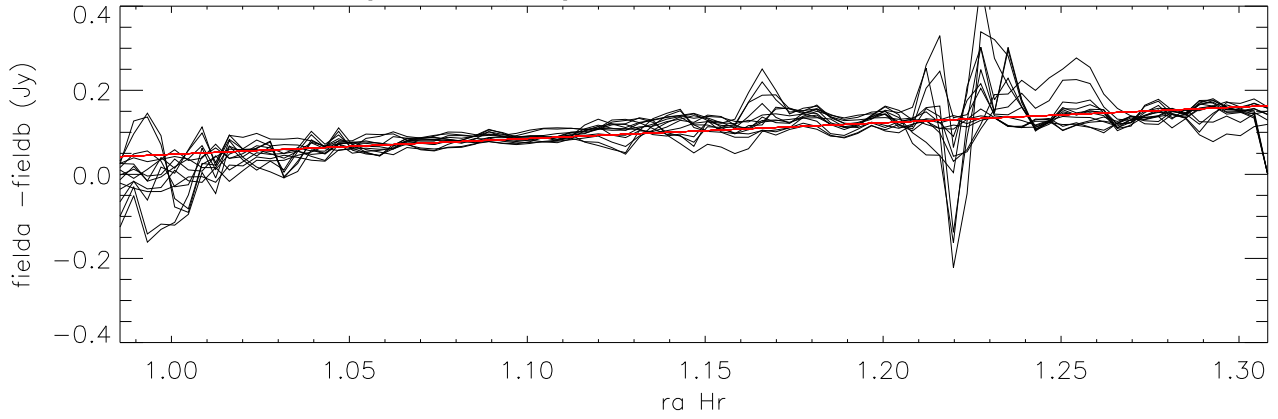
difference overlapping maps (long direction=ra) Cloop:2 Lloop:1 (Field12 - Field11A)
