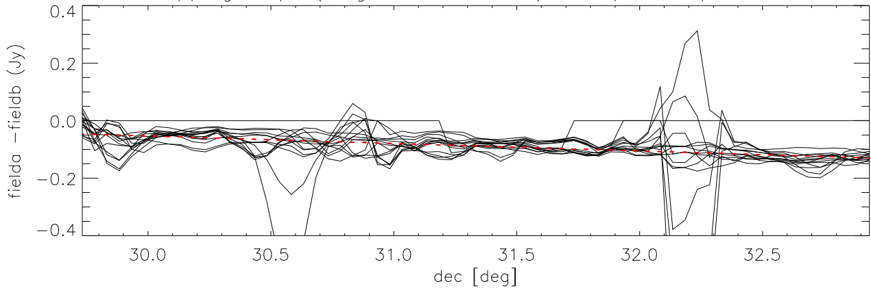
difference overlapping maps (long direction= dec) Cloop:2 Lloop:1 *Field3 - Field11A)
