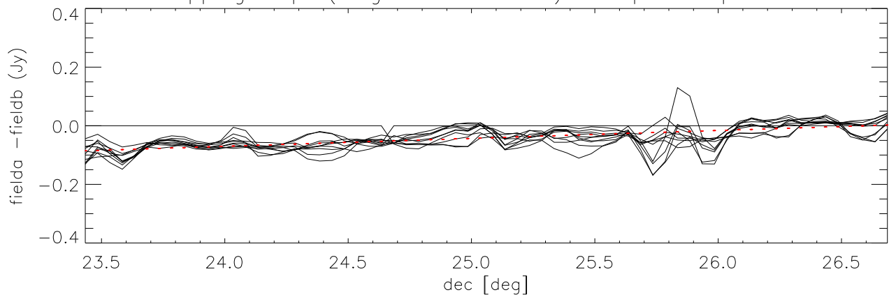
difference overlapping maps (long direction= dec) Cloop:2 Lloop:1 *Field6 - Field5)
