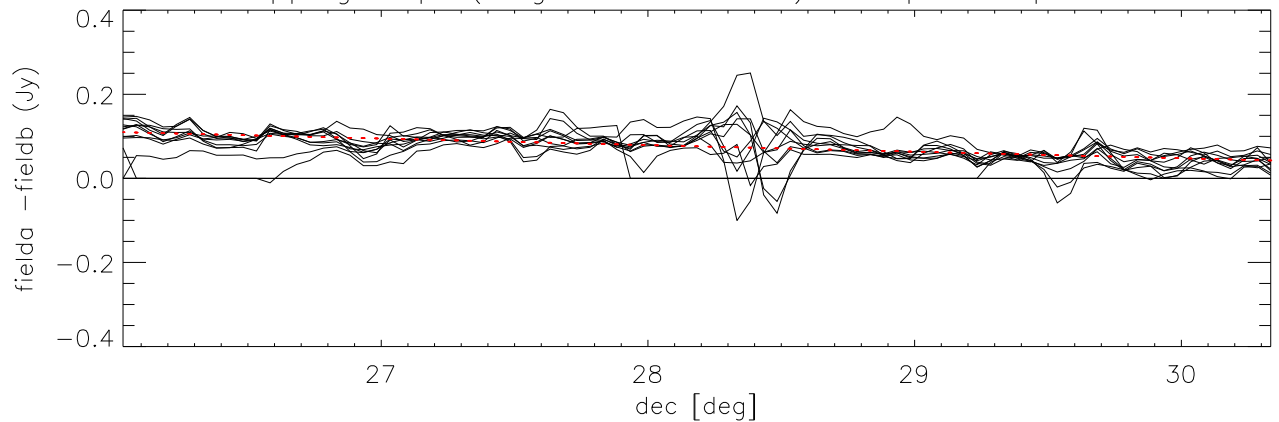
difference overlapping maps (long direction= dec) Cloop:2 Lloop:1 *Field1.05 - Field4)
