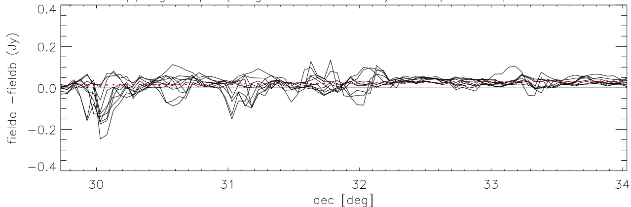
difference overlapping maps (long direction= dec) Cloop:2 Lloop:1 *Field4.05 - Field3.05)
