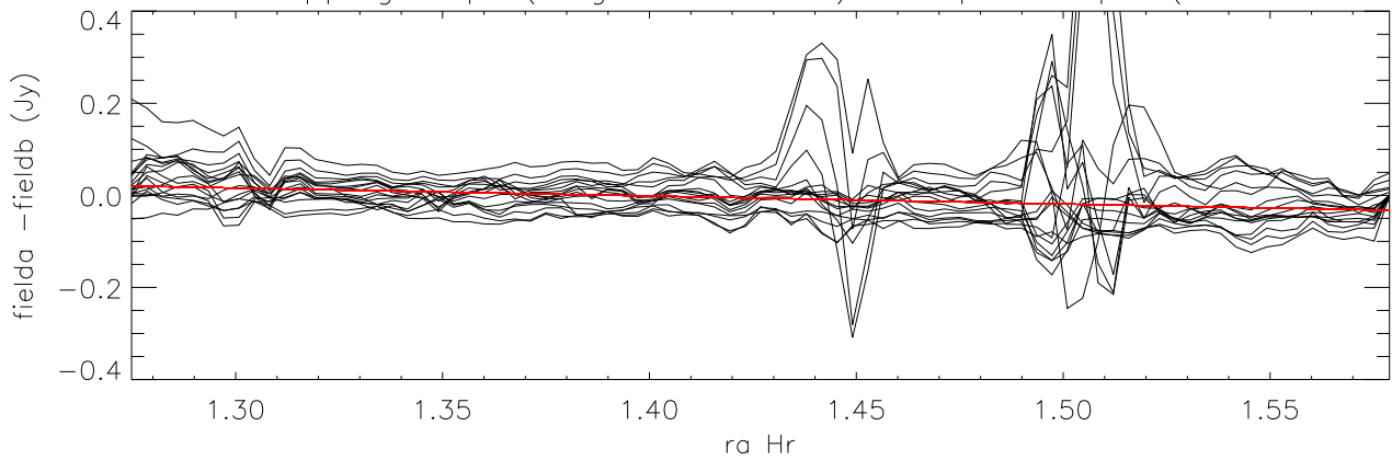
difference overlapping maps (long direction= dec) Cloop:2 Lloop:1 *Field1 - Field2)
