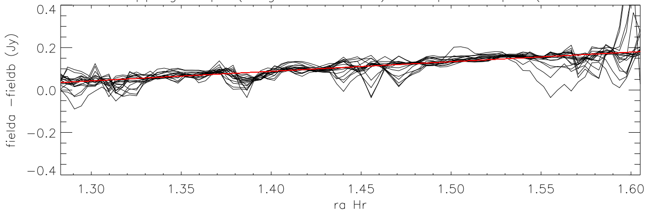
difference overlapping maps (long direction=ra) Cloop:2 Lloop:1 (Field7 - Field2.05)
