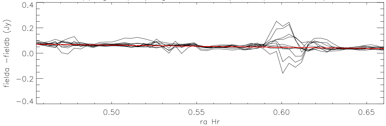
difference overlapping maps (long direction=ra) Cloop:2 Lloop:1 (Field6 - Field1.05)
