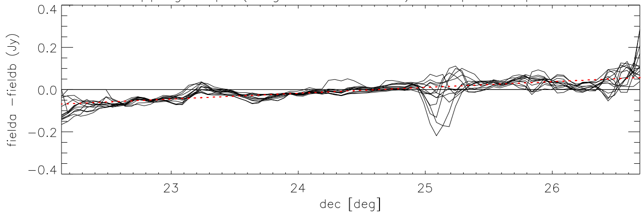
difference overlapping maps (long direction= dec) Cloop:2 Lloop:1 *Field7 - Field6)
