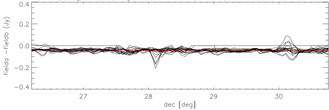
difference overlapping maps (long direction= dec) Cloop:2 Lloop:1 *Field5 - Field14)
