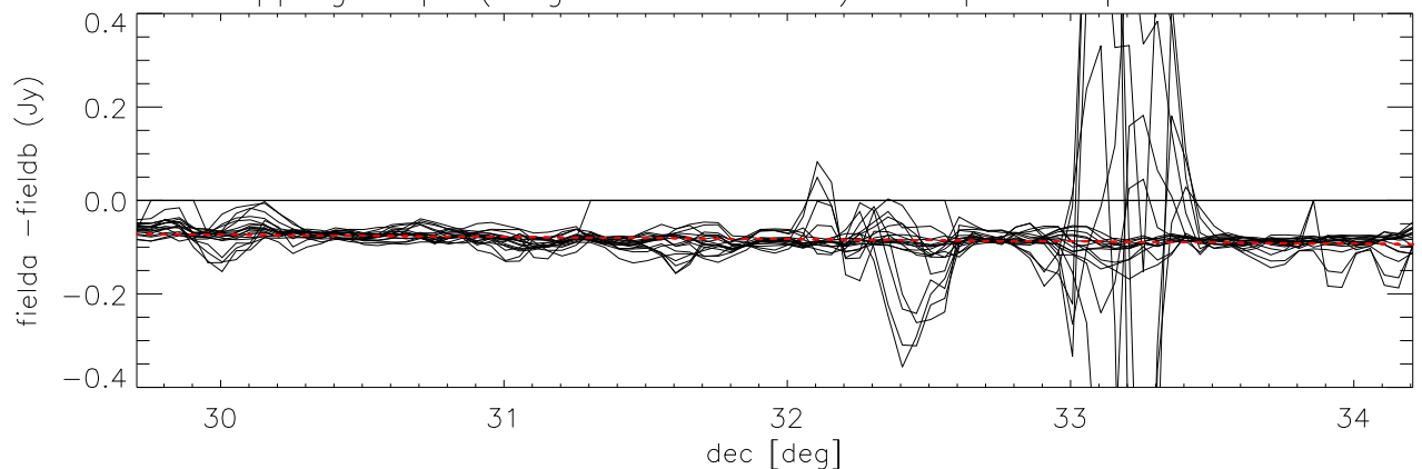
difference overlapping maps (long direction= dec) Cloop:2 Lloop:1 *Field4 - Field12)
