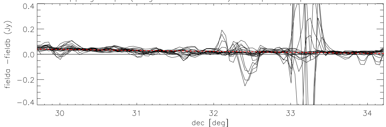
difference overlapping maps (long direction= dec) Cloop:1 Lloop:1 *Field4 - Field12)
