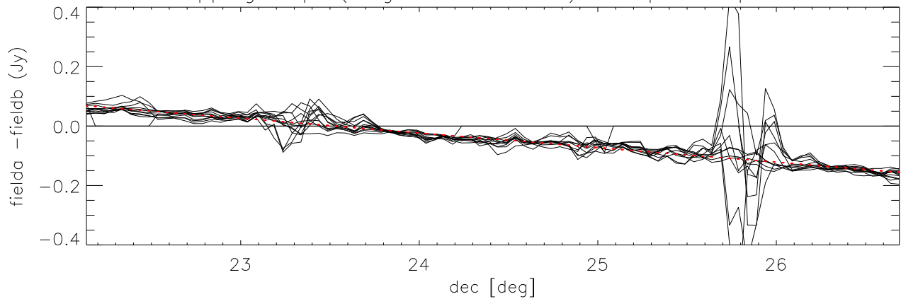
difference overlapping maps (long direction= dec) Cloop:1 Lloop:1 *Field7 - Field6)
