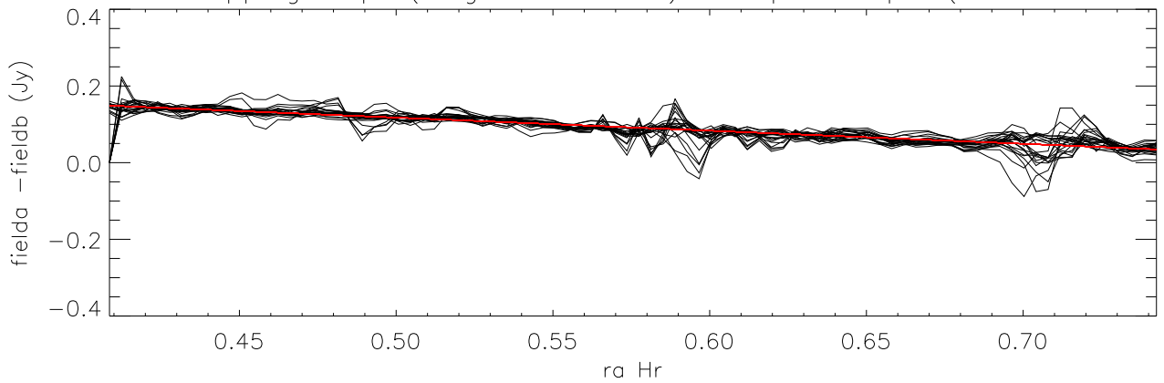
difference overlapping maps (long direction=ra) Cloop:1 Lloop:1 (Field1.05 - Field3.05)
