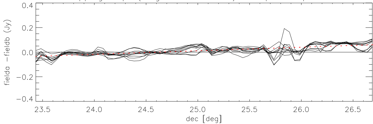
difference overlapping maps (long direction= dec) Cloop:1 Lloop:1 *Field6 - Field5)
