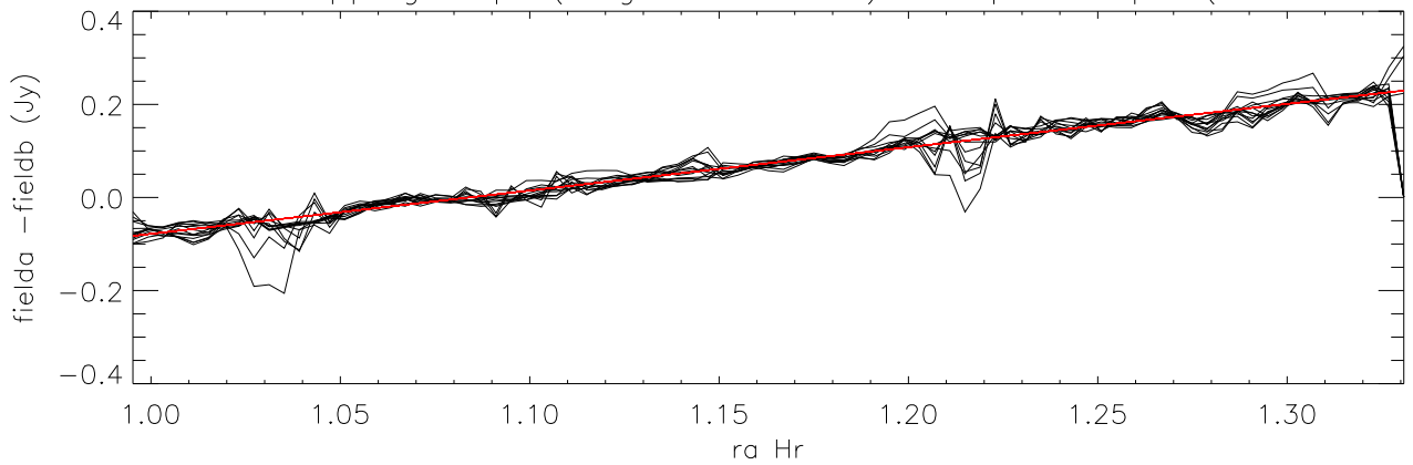
difference overlapping maps (long direction=ra) Cloop:1 Lloop:1 (Field2.05 - Field4.05)
