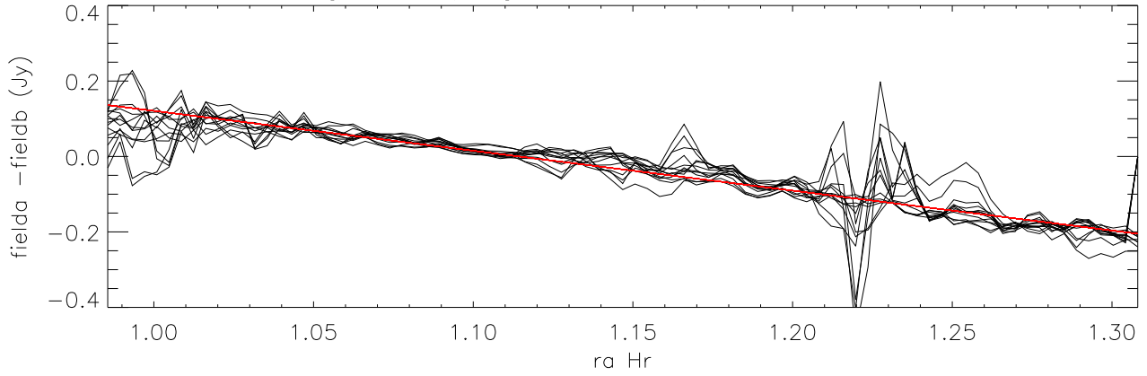
difference overlapping maps (long direction=ra) Cloop:1 Lloop:1 (Field12 - Field11A)
