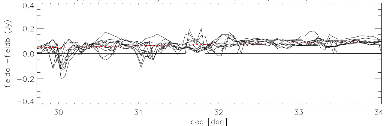
difference overlapping maps (long direction= dec) Cloop:1 Lloop:1 *Field4.05 - Field3.05)
