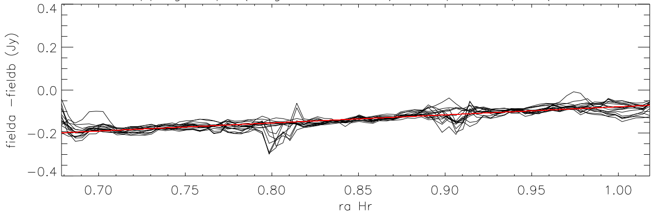
difference overlapping maps (long direction=ra) Cloop:1 Lloop:1 (Field3 - Field2)
