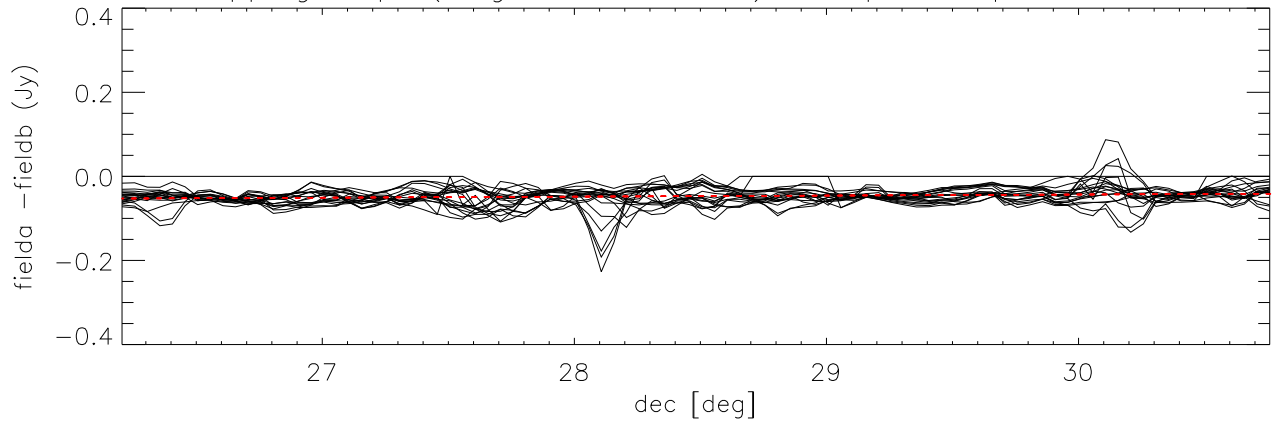
difference overlapping maps (long direction= dec) Cloop:1 Lloop:1 *Field5 - Field14)
