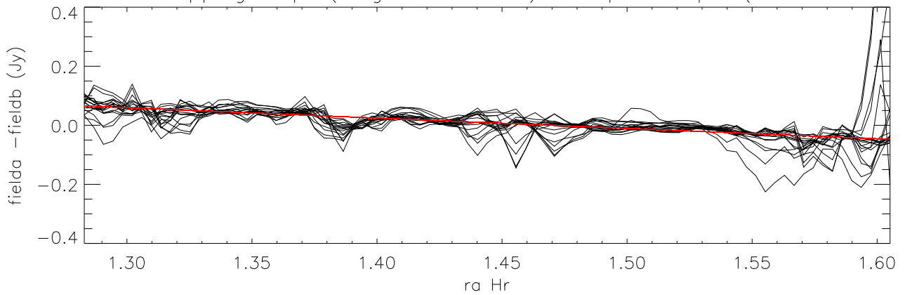
difference overlapping maps (long direction=ra) Cloop:1 Lloop:1 (Field7 - Field2.05)
