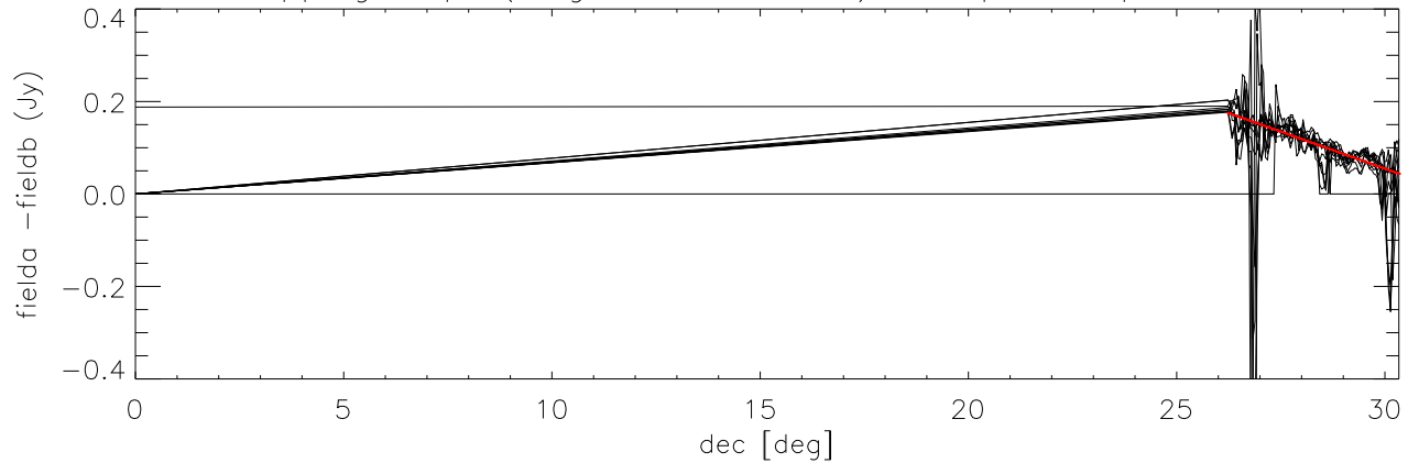
difference overlapping maps (long direction= dec) Cloop:1 Lloop:1 *Field1.05 - Field4)
