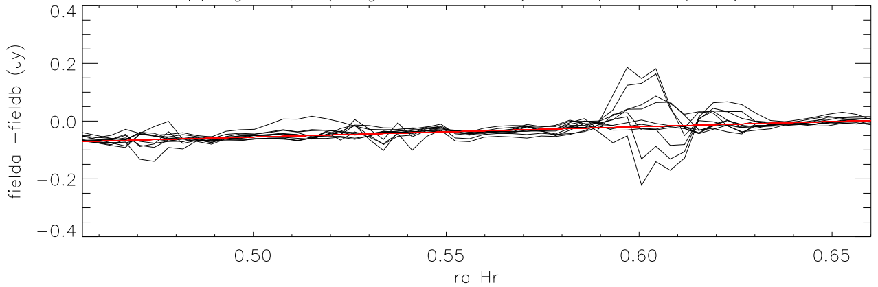
difference overlapping maps (long direction=ra) Cloop:1 Lloop:1 (Field6 - Field1.05)
