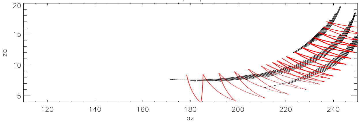
Field9 az,za positions
