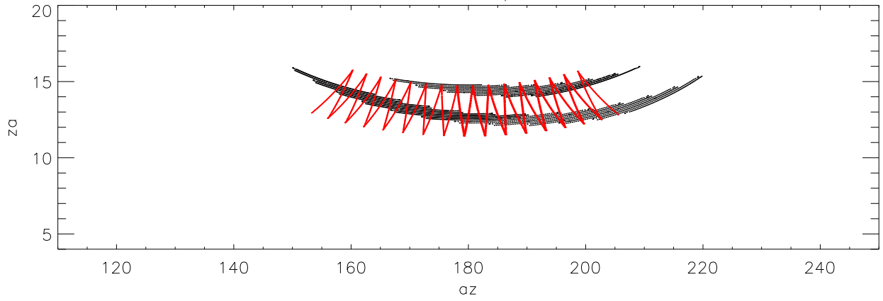
Field12 az,za positions
