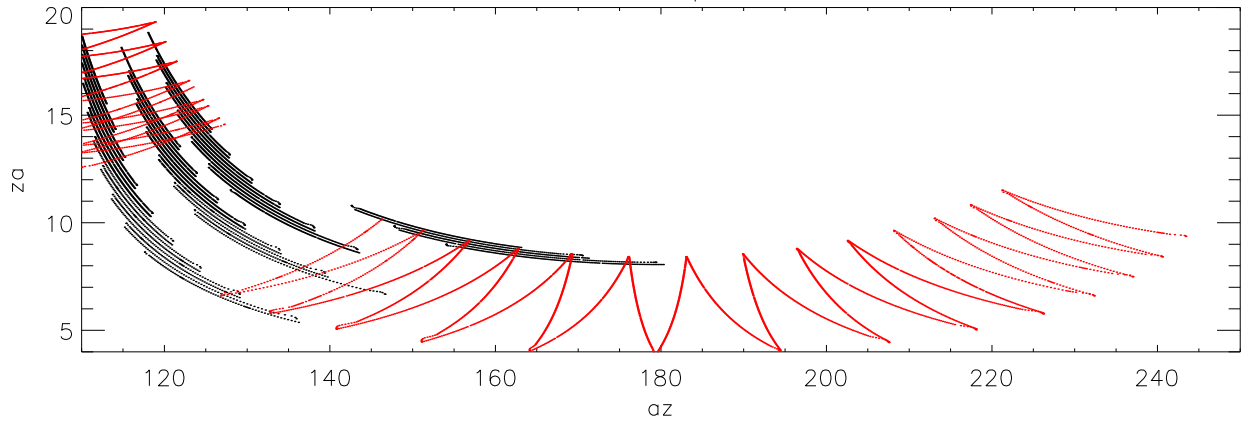
Field6 az,za positions
