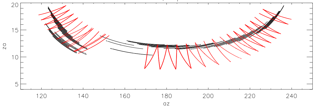
Field14 az,za positions
