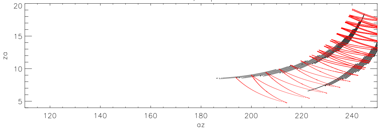
Field7 az,za positions
