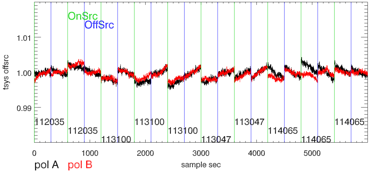
23apr13 a2749 lbw total power vs time. band 1
