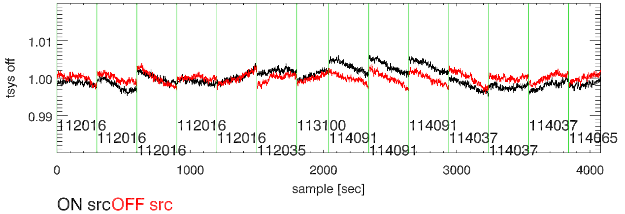
band 1 PoIB
