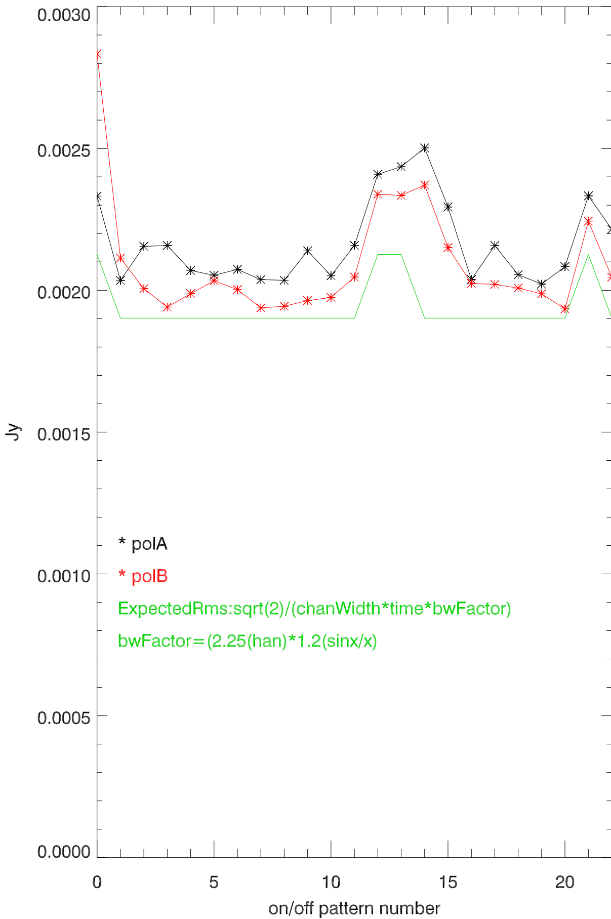
08apr13 lbw a2749 rms Noise for each on/off
