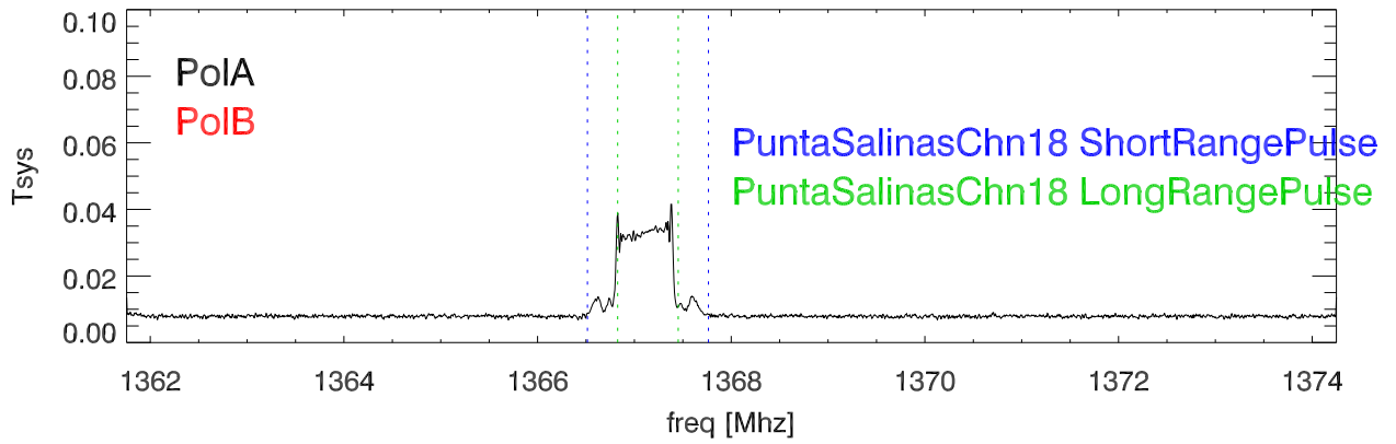
rms by channel (600 sec of data) (src:23102) sbc:1
