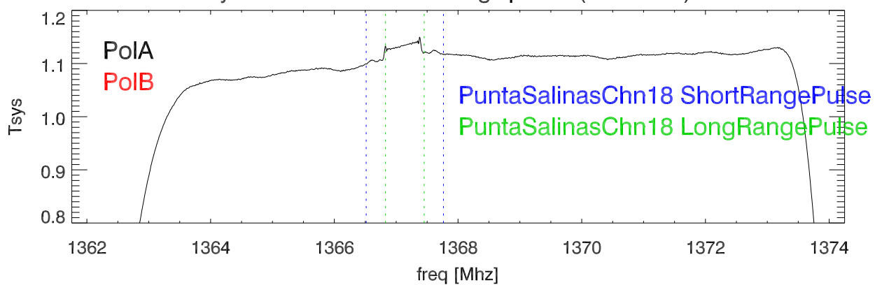
18may11 lbw a2335 600 sec avg spectra (src:23102) sbc:1
