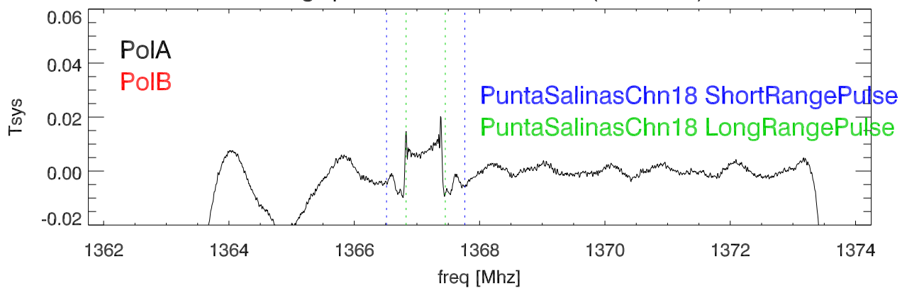
600 sec avg spectra baseline removed (src:23102) sbc:1
