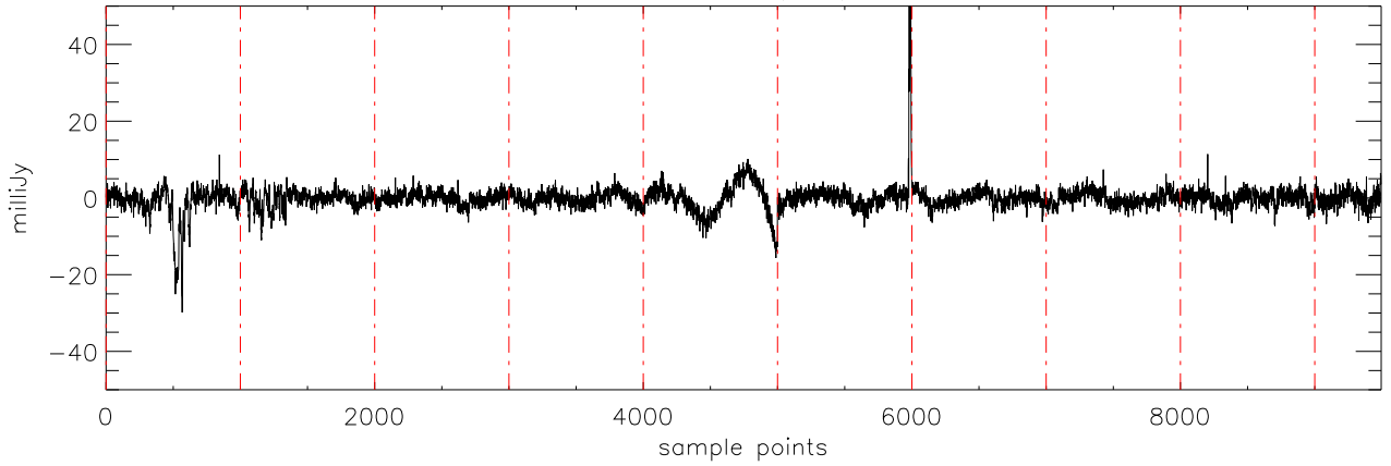
a2430 2MASS0746 06dec09 (AST) StokesQ freq:5125.
