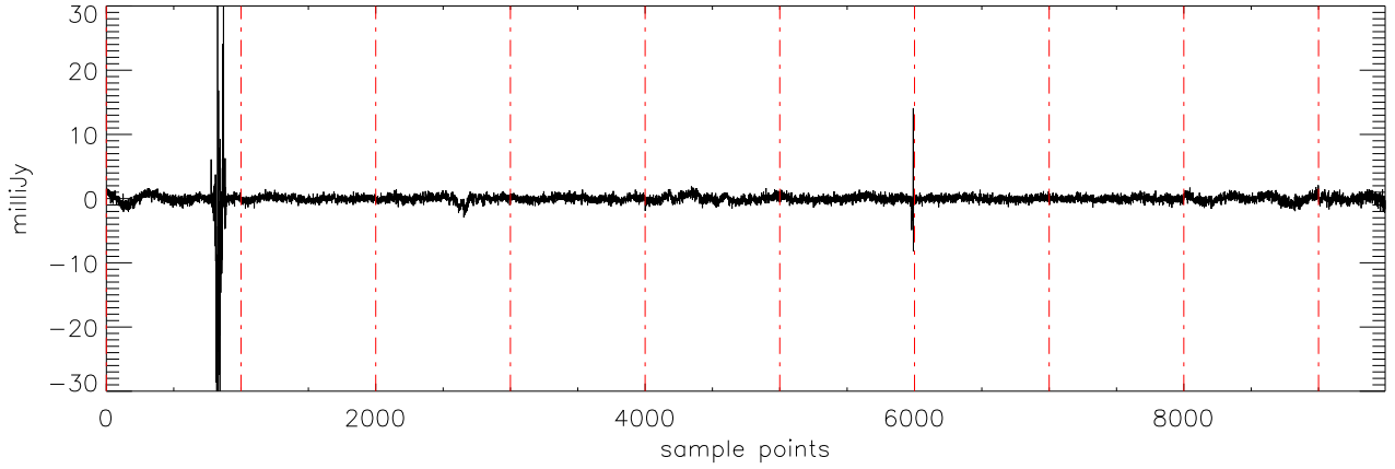
a2430 2MASS0746 06dec09 (AST) StokesV freq:4545.
