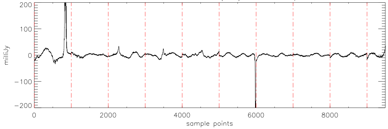
a2430 2MASS0746 06dec09 (AST) StokesI freq:4545.
