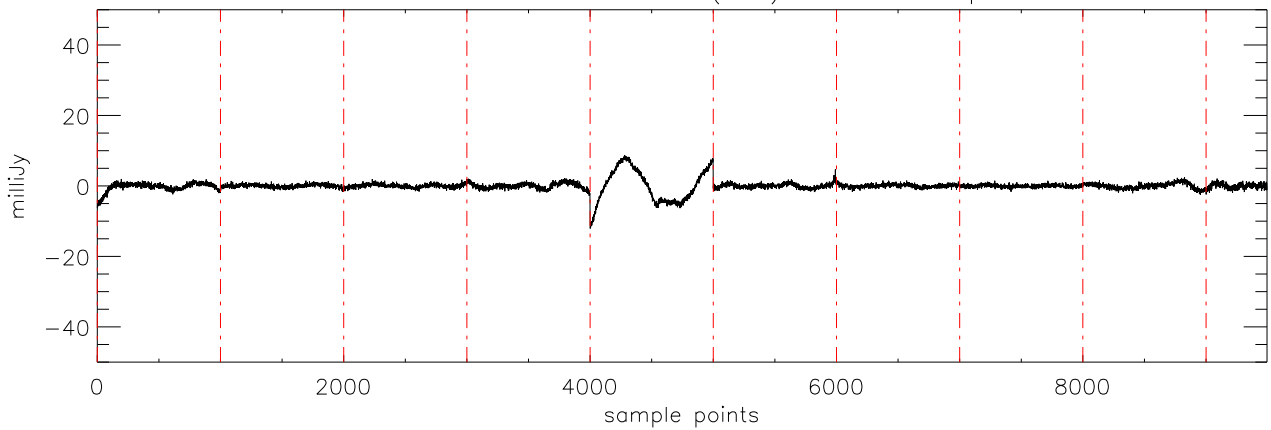
a2430 2MASS0746 06dec09 (AST) StokesU freq:4695.
