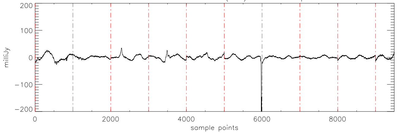
a2430 2MASS0746 06dec09 (AST) StokesI freq:4695.
