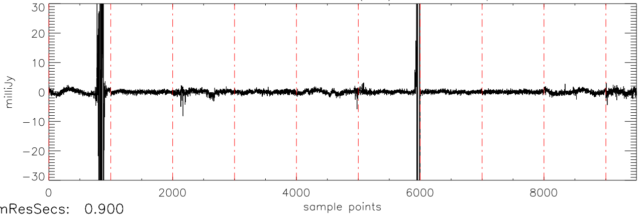
a2430 2MASS0746 06dec09 (AST) StokesV freq:4405.
