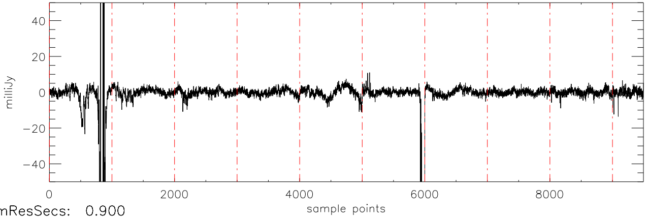
a2430 2MASS0746 06dec09 (AST) StokesQ freq:4405.
