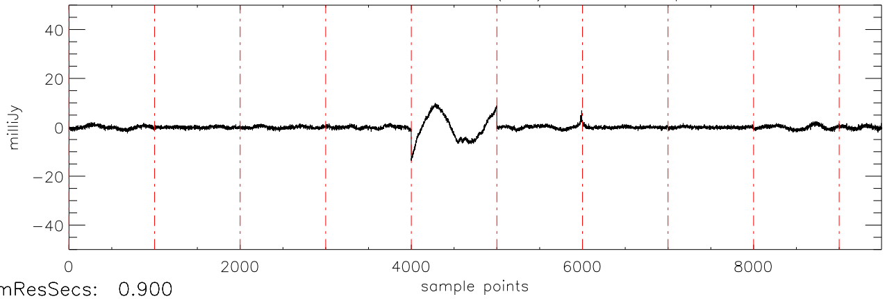
a2430 2MASS0746 06dec09 (AST) StokesU freq:4975.
