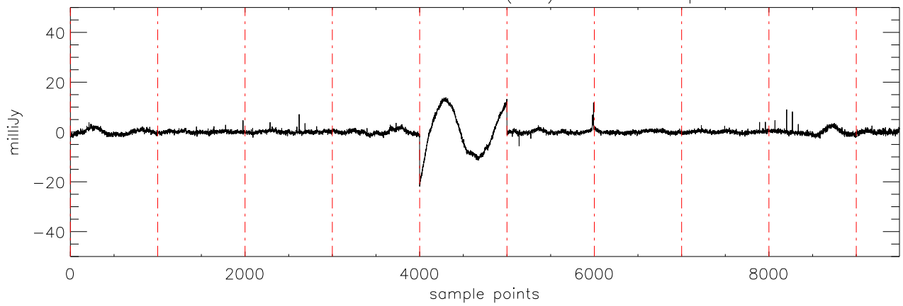
a2430 2MASS0746 06dec09 (AST) StokesU freq:5125.
