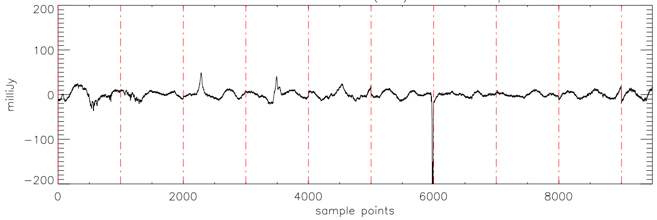
a2430 2MASS0746 06dec09 (AST) StokesI freq:5125.
