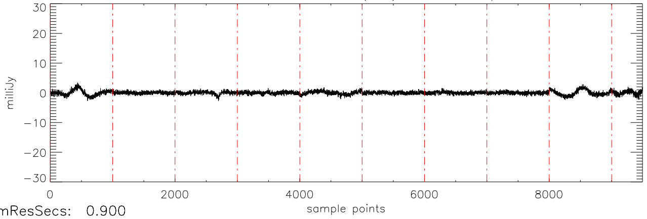
a2430 2MASS0746 06dec09 (AST) StokesV freq:4975.
