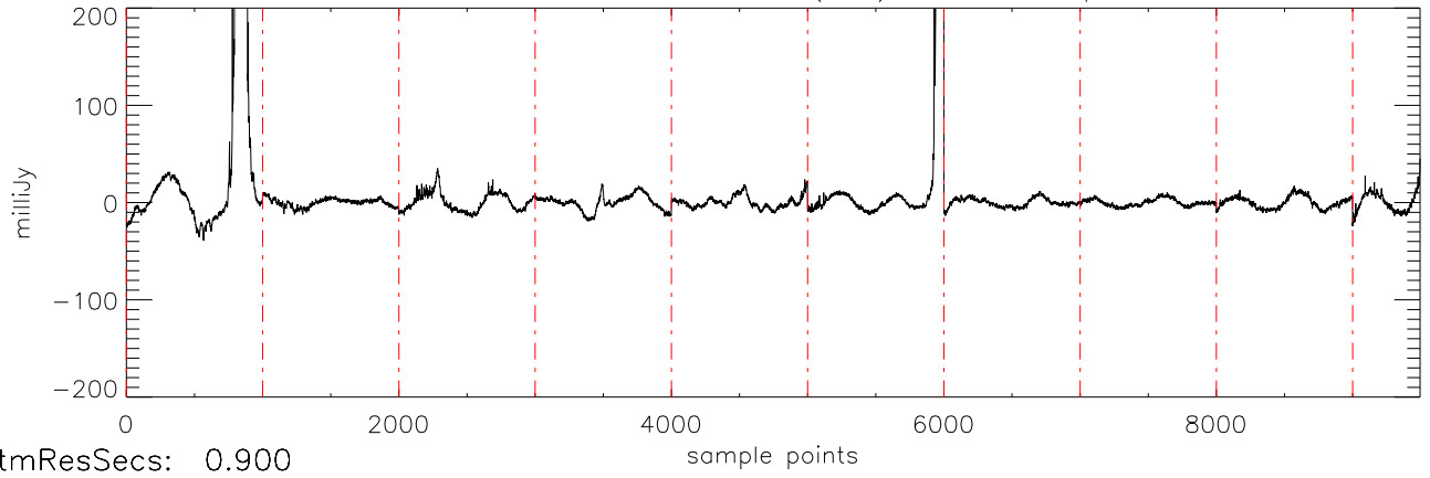
a2430 2MASS0746 06dec09 (AST) StokesI freq:4405.
