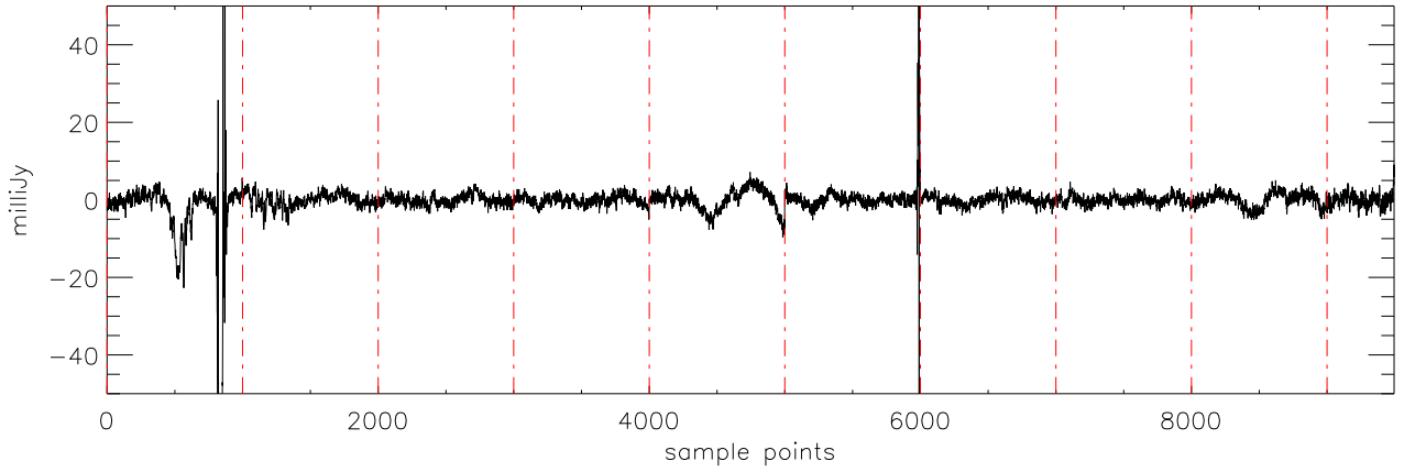
a2430 2MASS0746 06dec09 (AST) StokesQ freq:4545.
