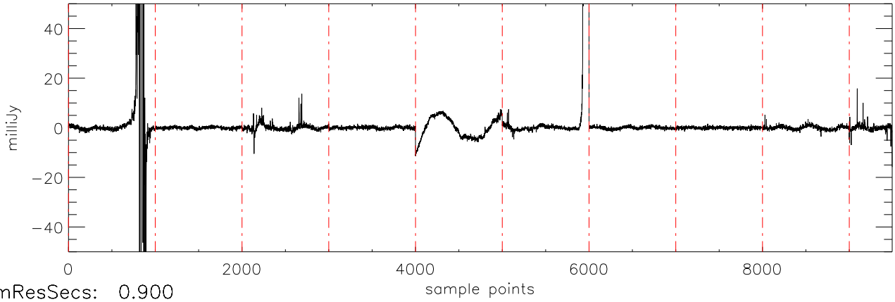
a2430 2MASS0746 06dec09 (AST) StokesU freq:4405.
