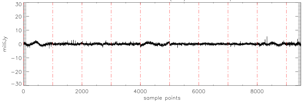
a2430 2MASS0746 06dec09 (AST) StokesV freq:5125.
