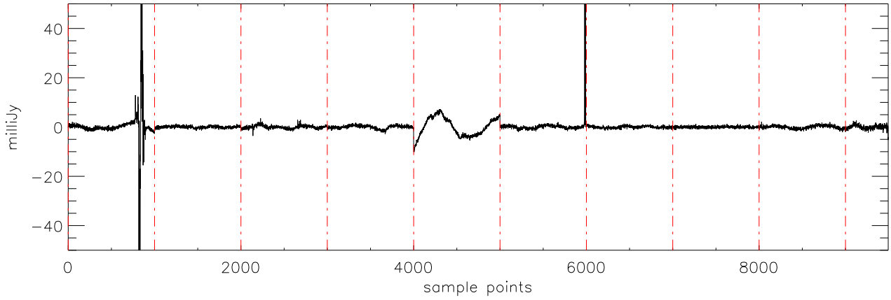
a2430 2MASS0746 06dec09 (AST) StokesU freq:4545.
