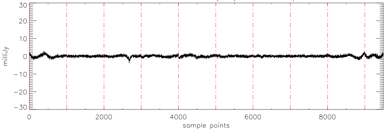
a2430 2MASS0746 06dec09 (AST) StokesV freq:4695.
