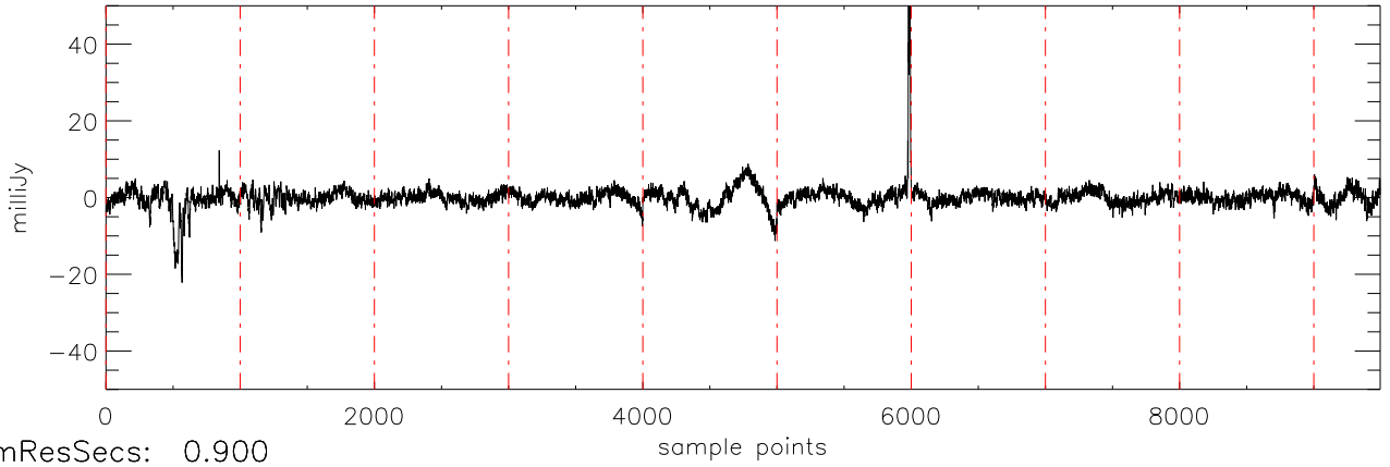
a2430 2MASS0746 06dec09 (AST) StokesQ freq:4975.
