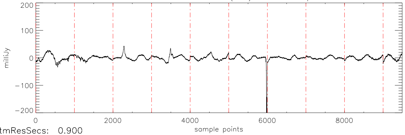
a2430 2MASS0746 06dec09 (AST) StokesI freq:4975.
