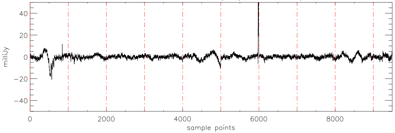
a2430 2MASS0746 06dec09 (AST) StokesQ freq:4695.
