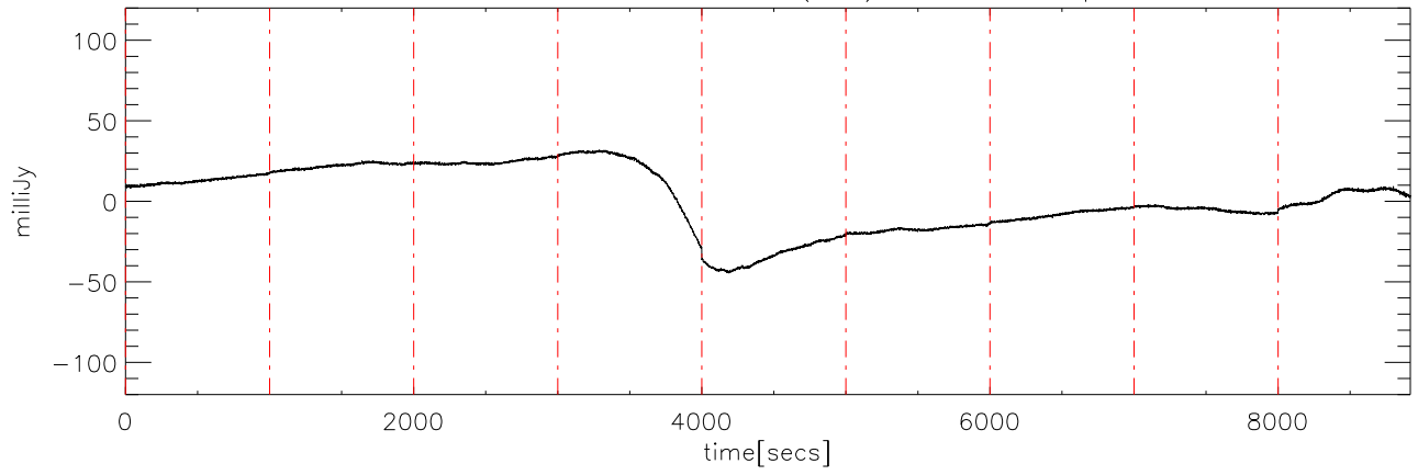
a2430 2MASS0746 04dec09 (AST) StokesU freq:4975.
