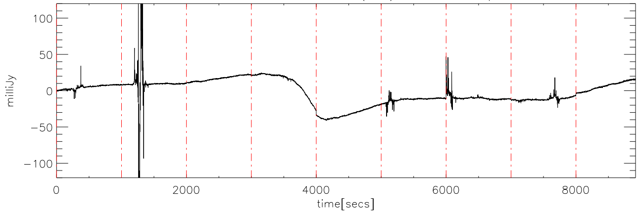
a2430 2MASS0746 04dec09 (AST) StokesU freq:4405.
