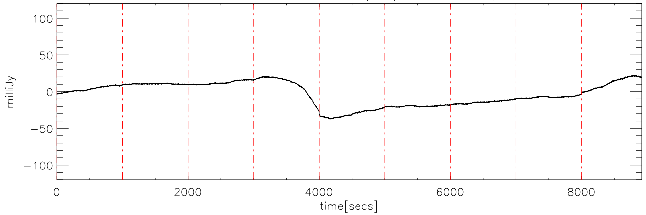
a2430 2MASS0746 04dec09 (AST) StokesU freq:4695.
