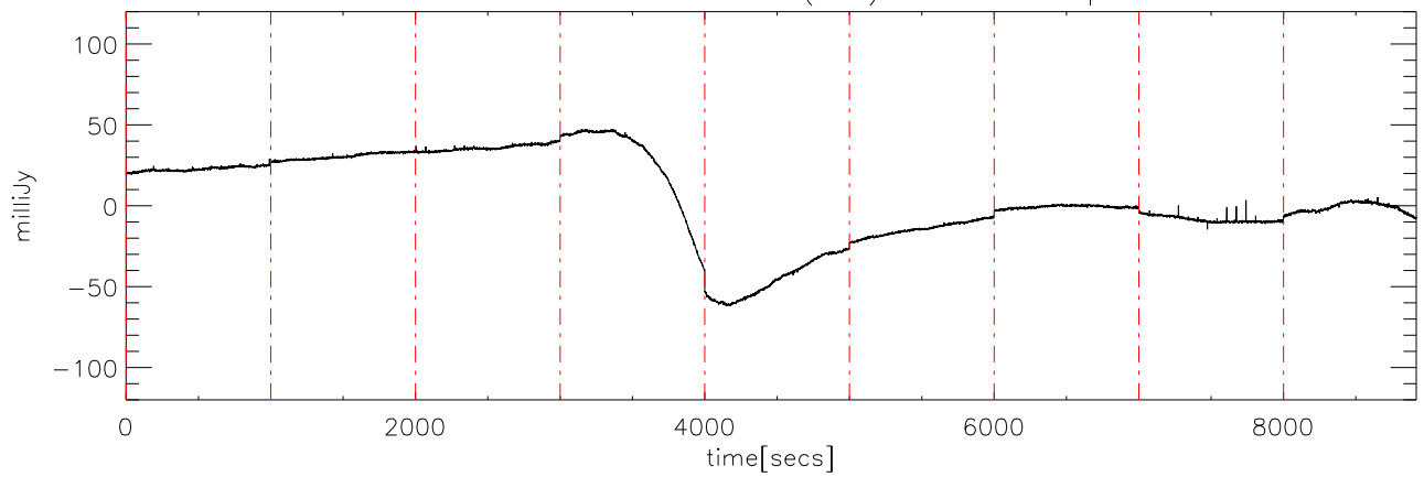
a2430 2MASS0746 04dec09 (AST) StokesU freq:5125.
