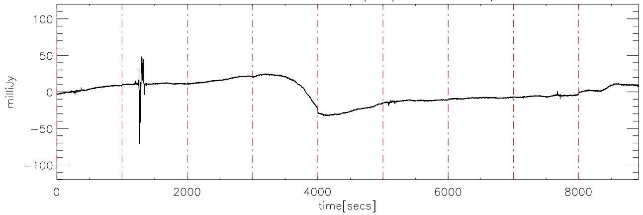
a2430 2MASS0746 04dec09 (AST) StokesU freq:4545.
