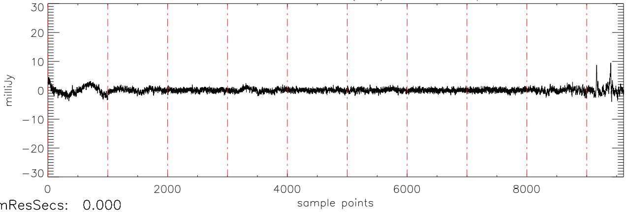
a2430 2MASS0036 05dec09 (AST) StokesV freq:2298.
