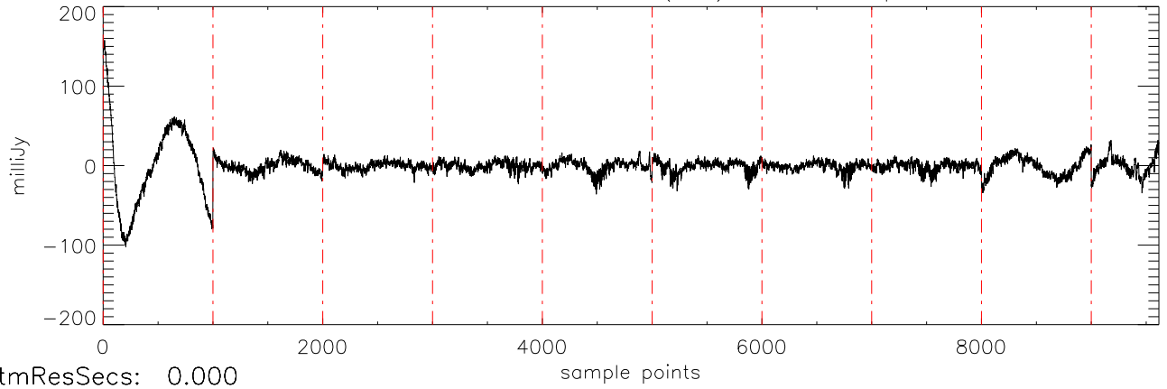
a2430 2MASS0036 05dec09 (AST) StokesI freq:2298.
