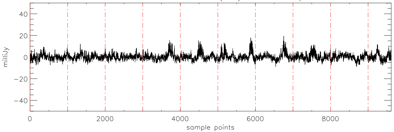
a2430 2MASS0036 05dec09 (AST) StokesQ freq:2754.
