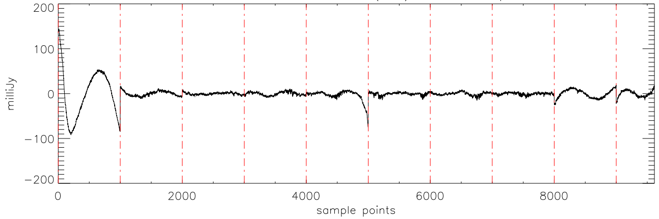
a2430 2MASS0036 05dec09 (AST) StokesI freq:2754.
