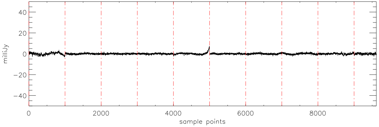
a2430 2MASS0036 05dec09 (AST) StokesU freq:2594.
