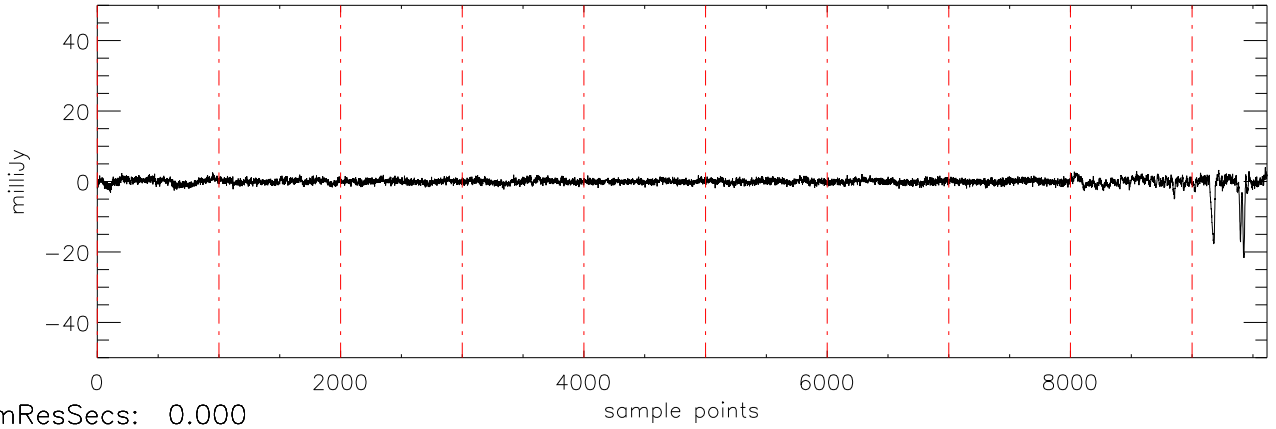
a2430 2MASS0036 05dec09 (AST) StokesU freq:2298.
