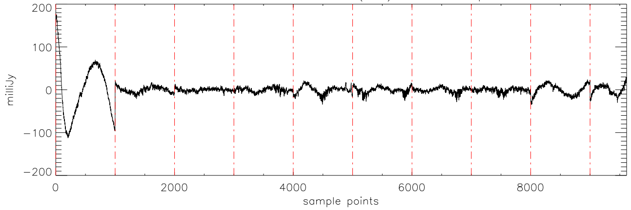
a2430 2MASS0036 05dec09 (AST) StokesI freq:2594.
