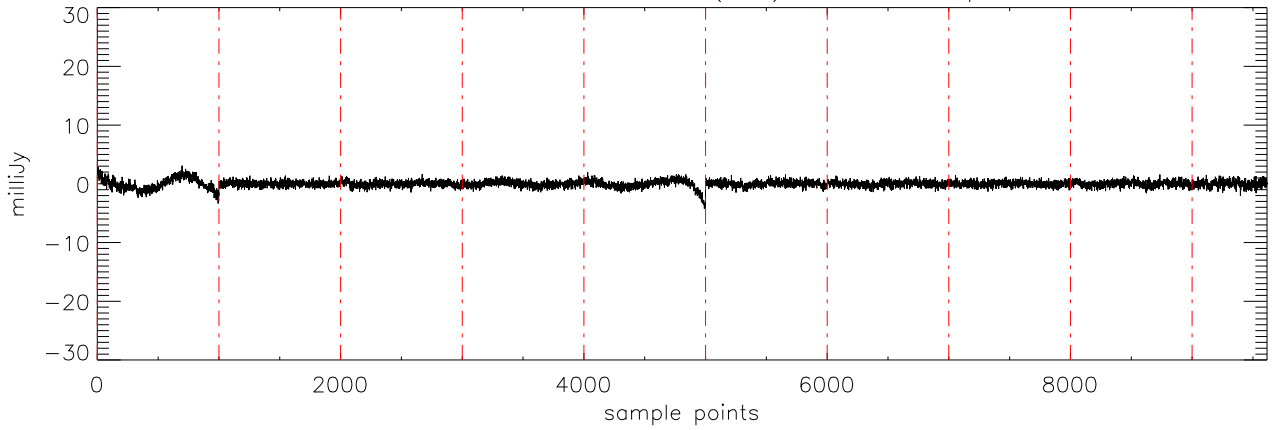
a2430 2MASS0036 05dec09 (AST) StokesV freq:2754.
