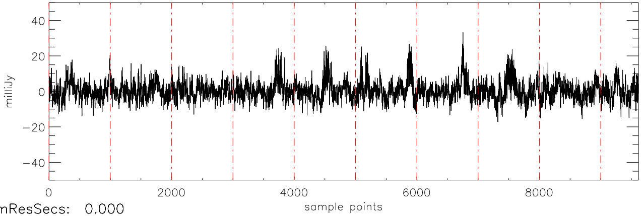
a2430 2MASS0036 05dec09 (AST) StokesQ freq:2298.
