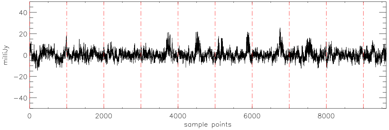
a2430 2MASS0036 05dec09 (AST) StokesQ freq:2594.
