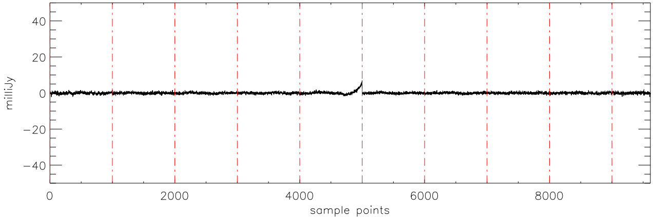
a2430 2MASS0036 05dec09 (AST) StokesU freq:2754.
