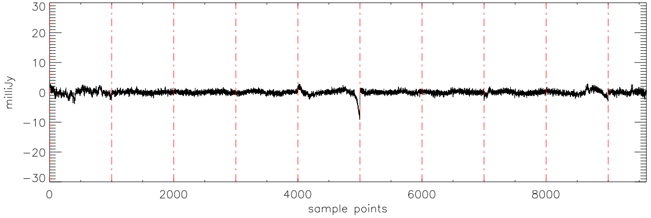
a2430 2MASS0036 05dec09 (AST) StokesV freq:2594.
