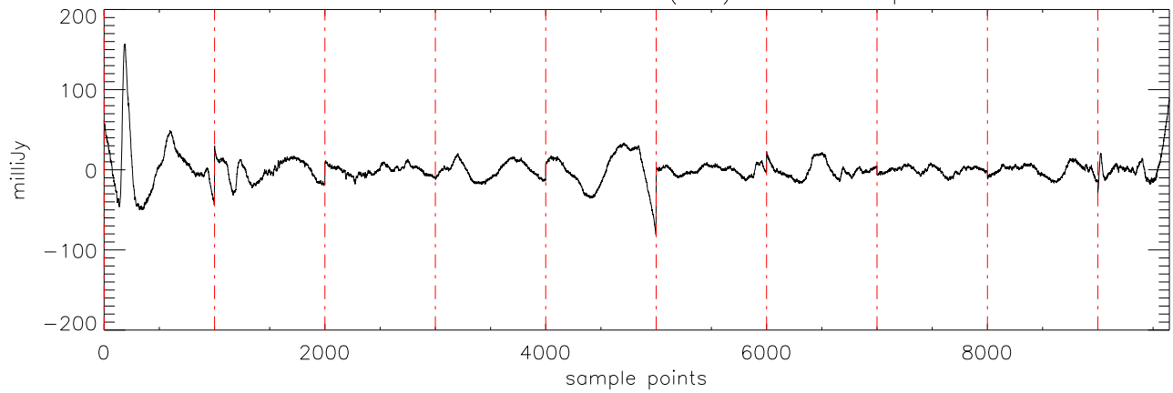
a2430 2MASS0036 03dec09 (AST) StokesI freq:5125.
