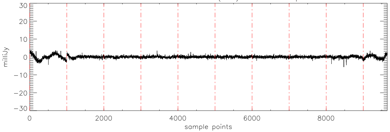
a2430 2MASS0036 03dec09 (AST) StokesV freq:5125.
