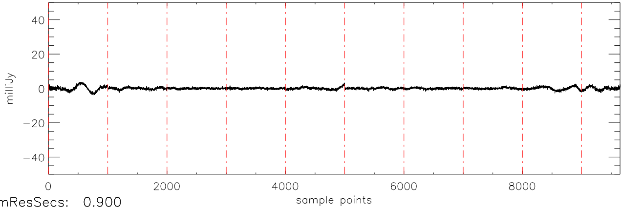
a2430 2MASS0036 03dec09 (AST) StokesU freq:4975.
