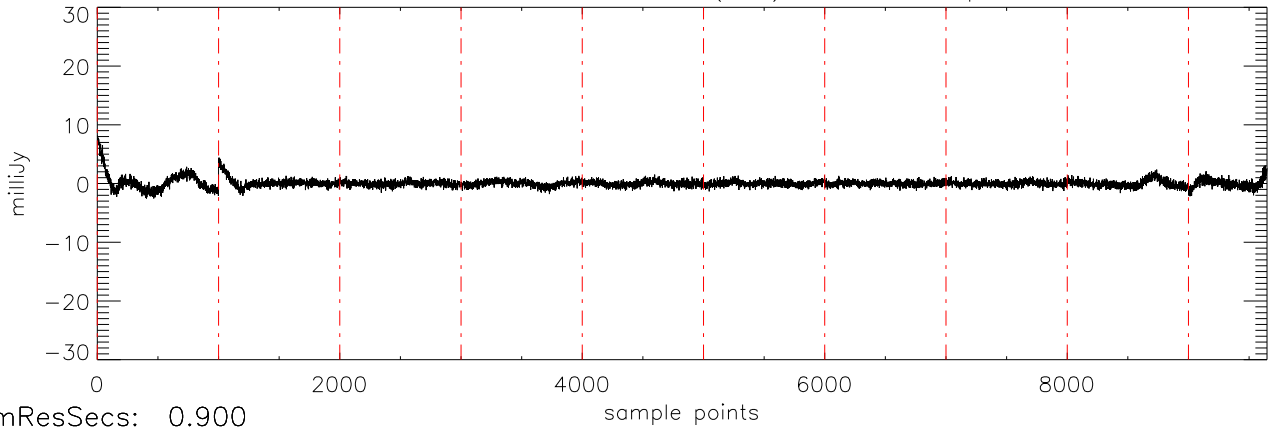
a2430 2MASS0036 03dec09 (AST) StokesV freq:4975.
