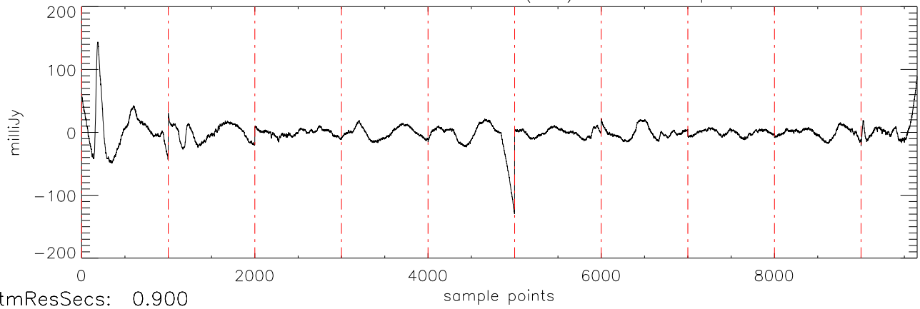
a2430 2MASS0036 03dec09 (AST) StokesI freq:4975.
