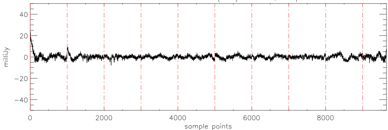
a2430 2MASS0036 03dec09 (AST) StokesQ freq:4695.
