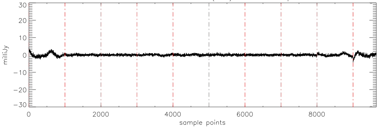
a2430 2MASS0036 03dec09 (AST) StokesV freq:4695.
