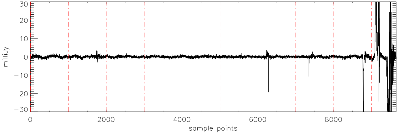
a2430 2MASS0036 03dec09 (AST) StokesV freq:4545.
