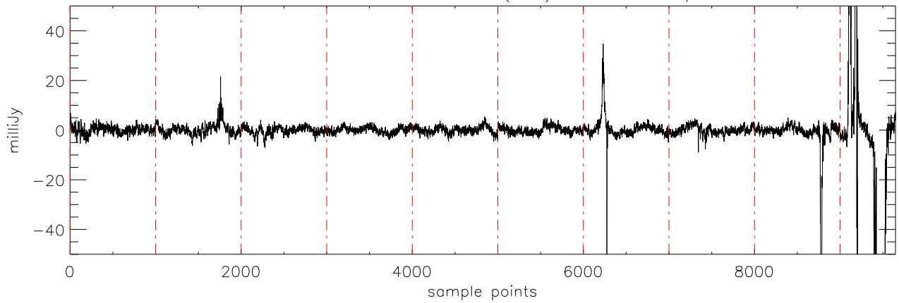
a2430 2MASS0036 03dec09 (AST) StokesQ freq:4545.
