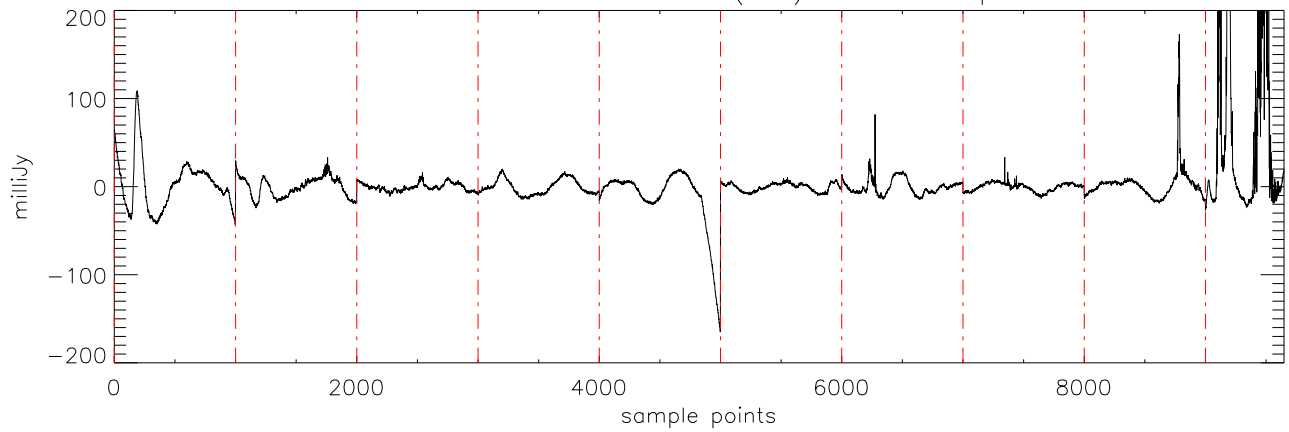
a2430 2MASS0036 03dec09 (AST) StokesI freq:4545.
