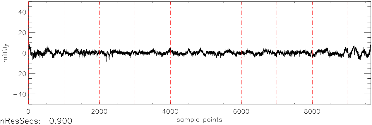
a2430 2MASS0036 03dec09 (AST) StokesQ freq:4975.
