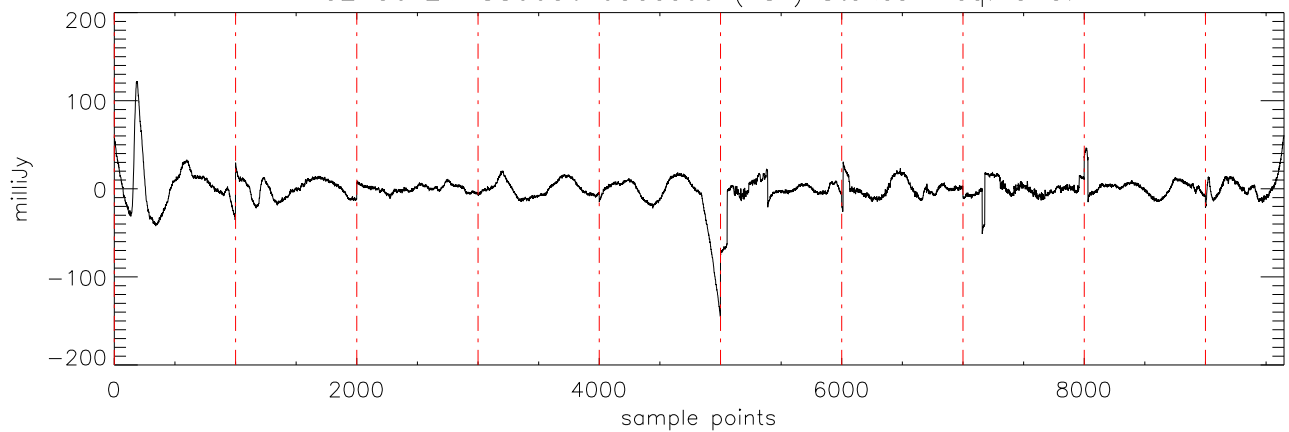
a2430 2MASS0036 03dec09 (AST) StokesI freq:4695.
