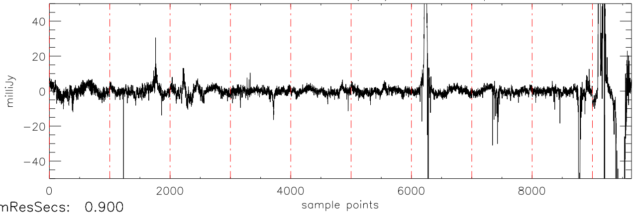
a2430 2MASS0036 03dec09 (AST) StokesQ freq:4405.
