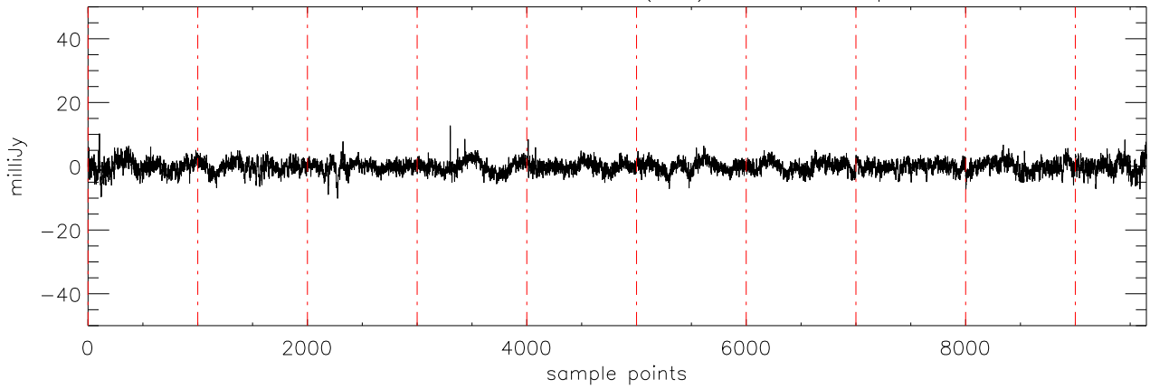
a2430 2MASS0036 03dec09 (AST) StokesQ freq:5125.
