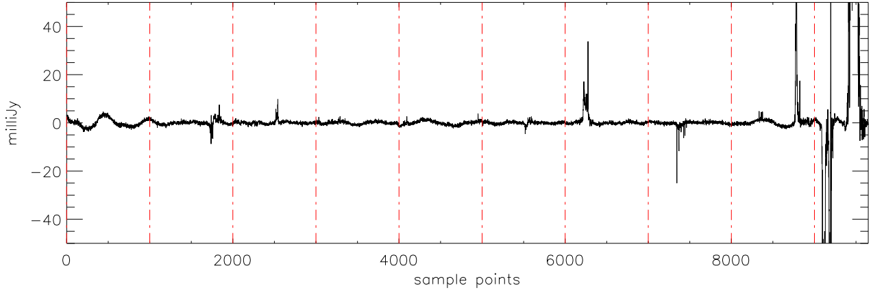
a2430 2MASS0036 03dec09 (AST) StokesU freq:4545.
