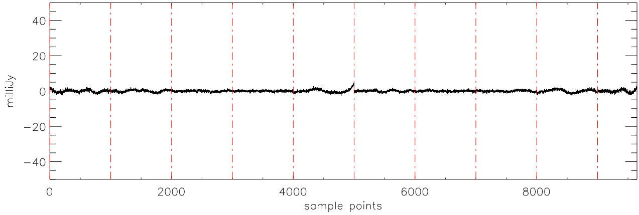
a2430 2MASS0036 03dec09 (AST) StokesU freq:5125.
