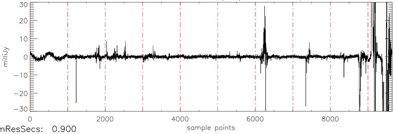
a2430 2MASS0036 03dec09 (AST) StokesV freq:4405.
