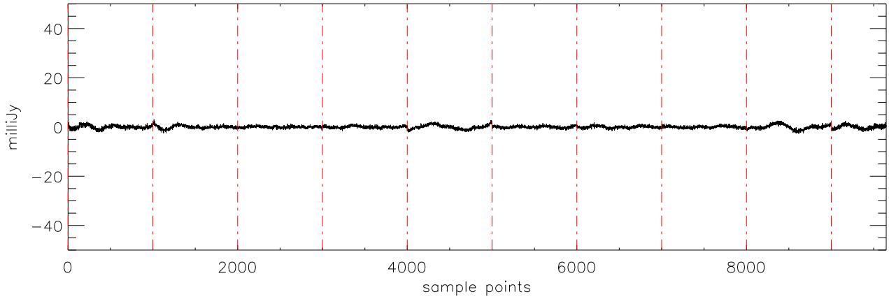
a2430 2MASS0036 03dec09 (AST) StokesU freq:4695.
