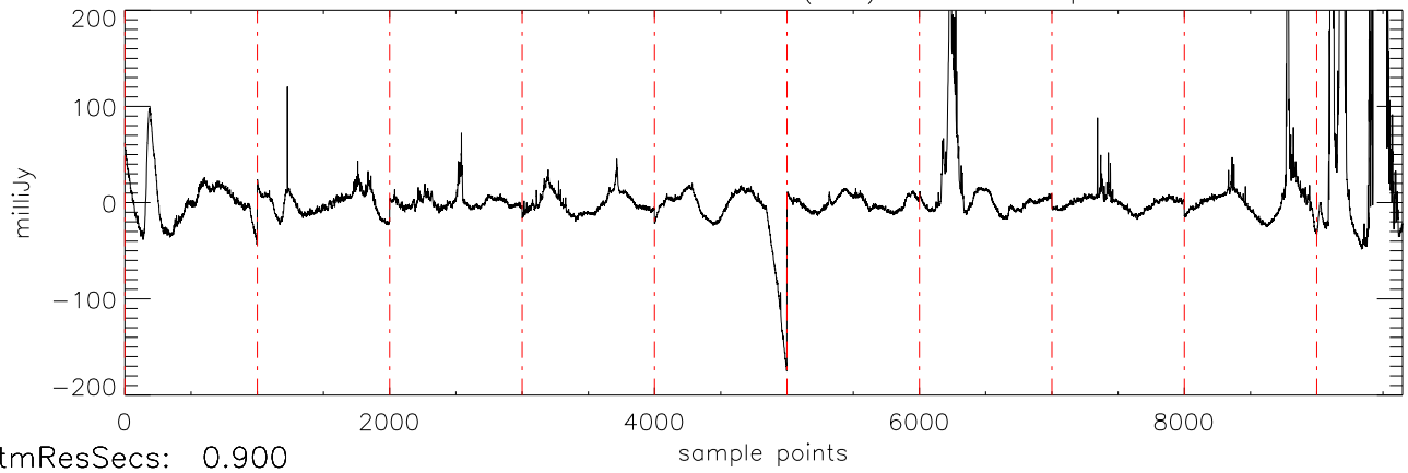
a2430 2MASS0036 03dec09 (AST) StokesI freq:4405.
