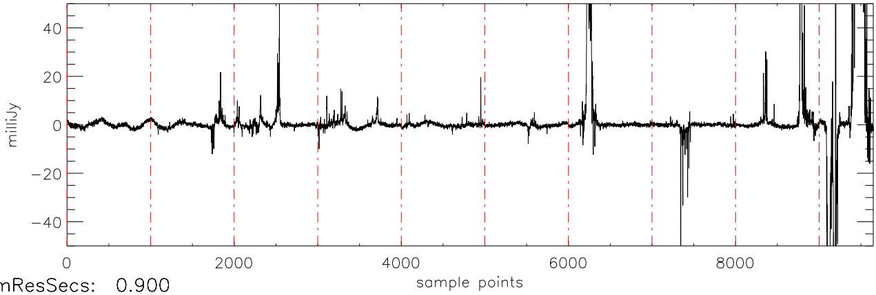
a2430 2MASS0036 03dec09 (AST) StokesU freq:4405.
