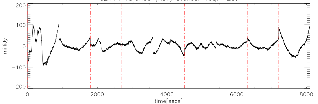
a2414 15jun09 (AST) StokesI freq:4725.
