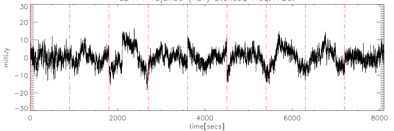
a2414 15jun09 (AST) StokesQ freq:4725.
