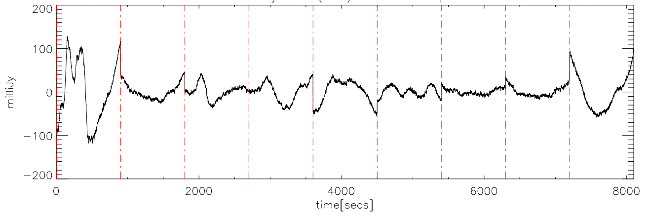
a2414 15jun09 (AST) StokesI freq:5125.
