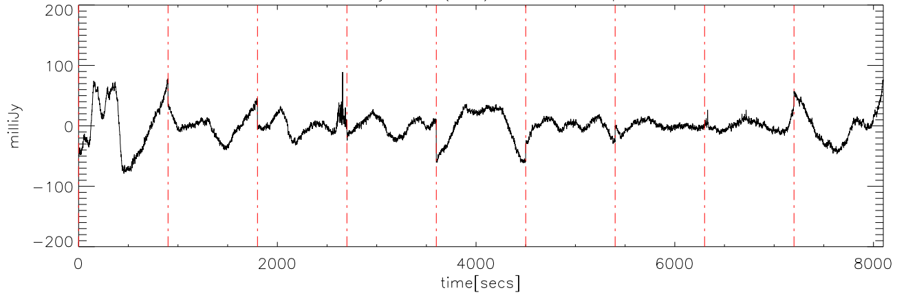
a2414 15jun09 (AST) StokesI freq:4475.
