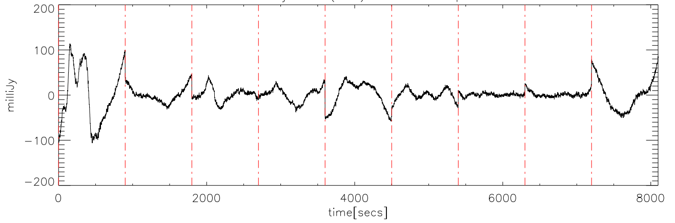
a2414 15jun09 (AST) StokesI freq:5000.
