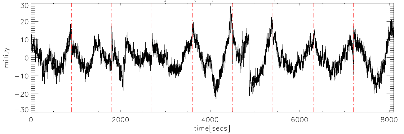
a2414 15jun09 (AST) StokesQ freq:4600.
