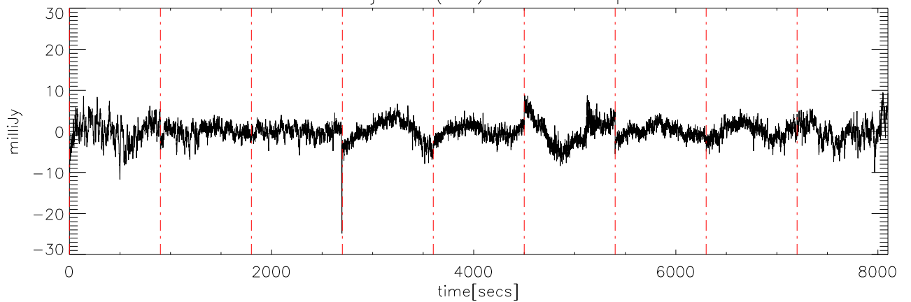
a2414 15jun09 (AST) StokesU freq:5250.
