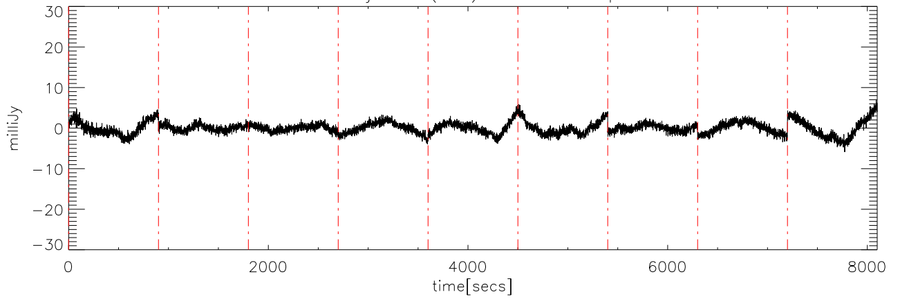
a2414 15jun09 (AST) StokesU freq:5000.
