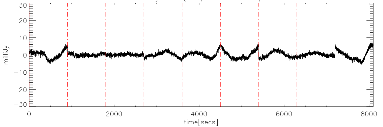
a2414 15jun09 (AST) StokesU freq:5125.
