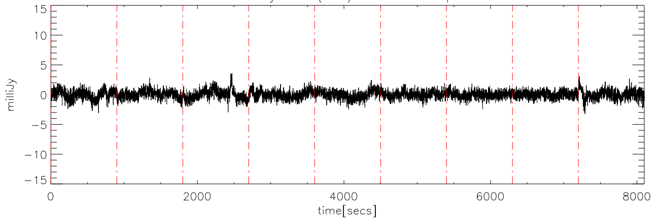
a2414 15jun09 (AST) StokesV freq:4600.
