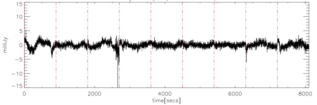
a2414 15jun09 (AST) StokesV freq:4475.
