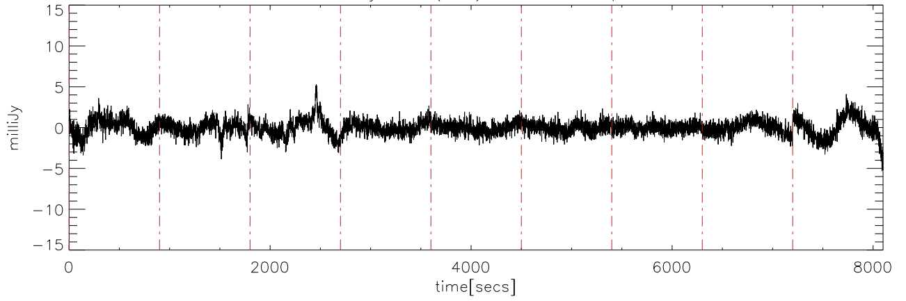
a2414 15jun09 (AST) StokesV freq:5000.
