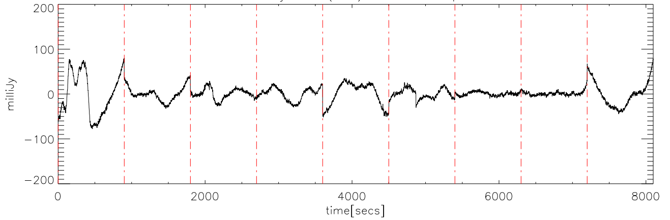
a2414 15jun09 (AST) StokesI freq:4600.
