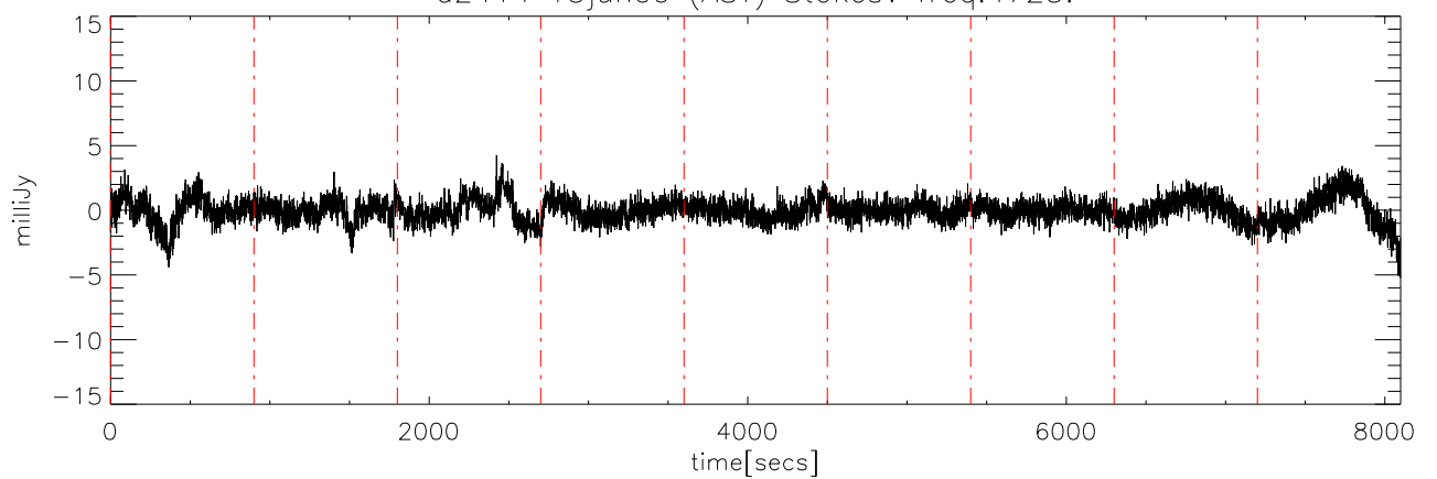
a2414 15jun09 (AST) StokesV freq:4725.
