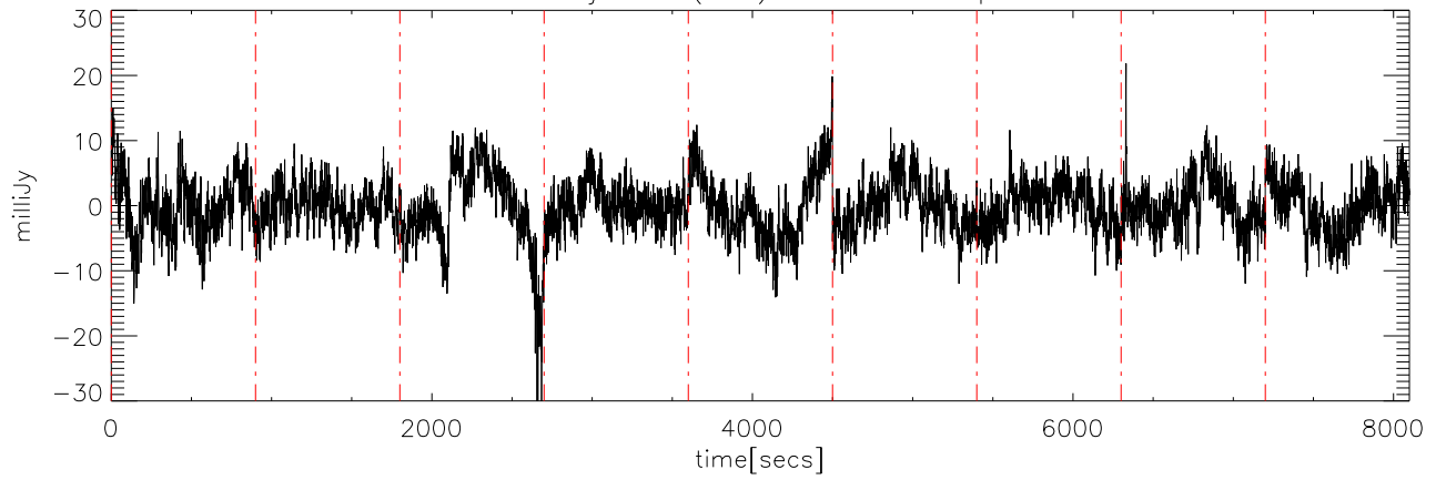
a2414 15jun09 (AST) StokesQ freq:4475.
