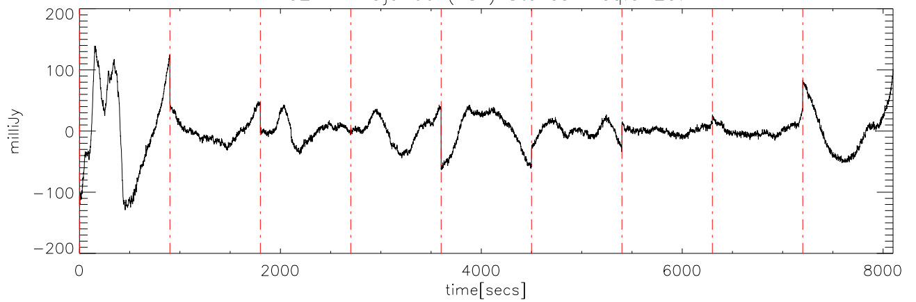
a2414 15jun09 (AST) StokesI freq:5250.
