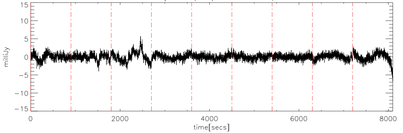
a2414 15jun09 (AST) StokesV freq:5125.
