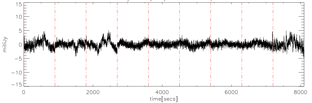
a2414 15jun09 (AST) StokesV freq:5250.
