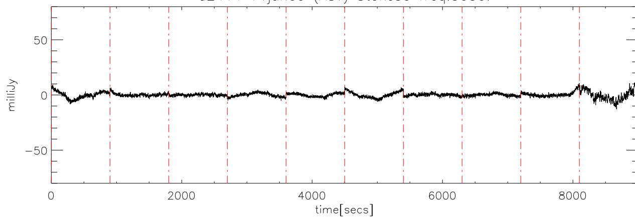
a2414 14jun09 (AST) StokesU freq:3150.
