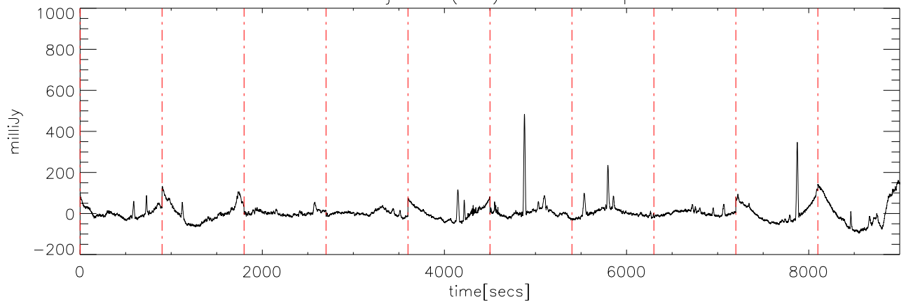
a2414 14jun09 (AST) StokesI freq:3850.
