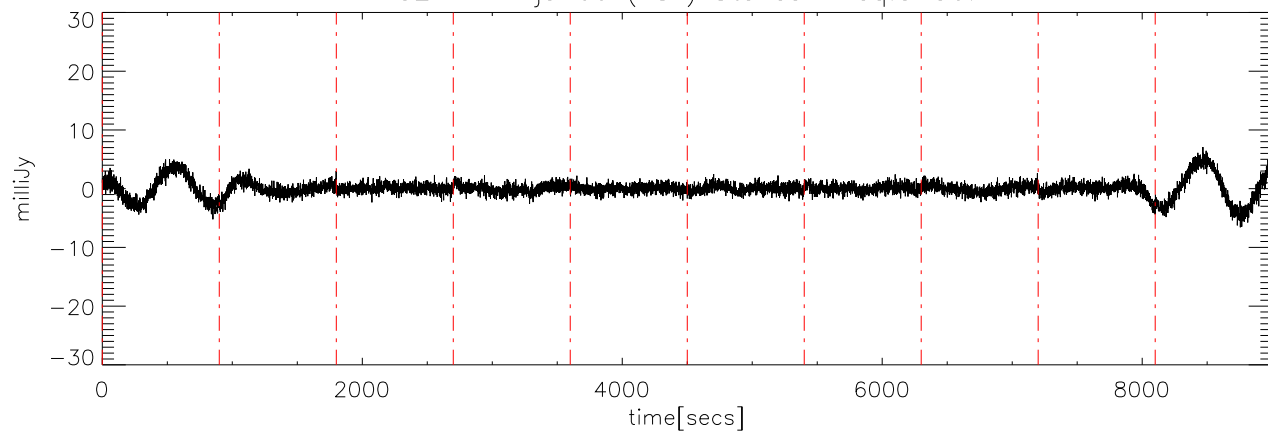
a2414 14jun09 (AST) StokesV freq:3250.
