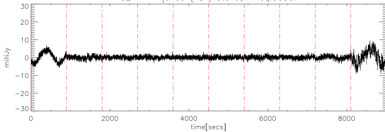
a2414 14jun09 (AST) StokesV freq:3150.
