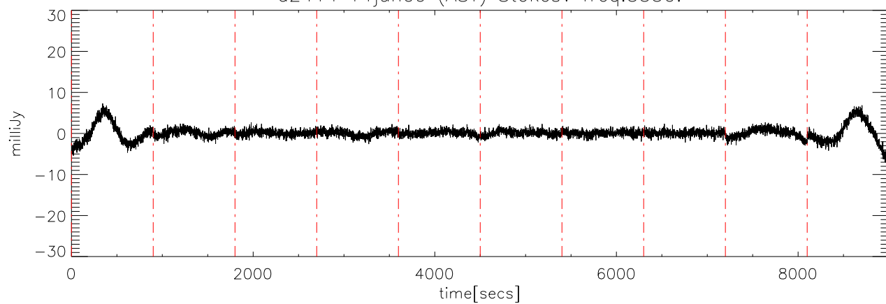
a2414 14jun09 (AST) StokesV freq:3350.
