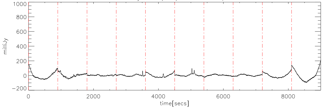
a2414 14jun09 (AST) StokesI freq:3700.
