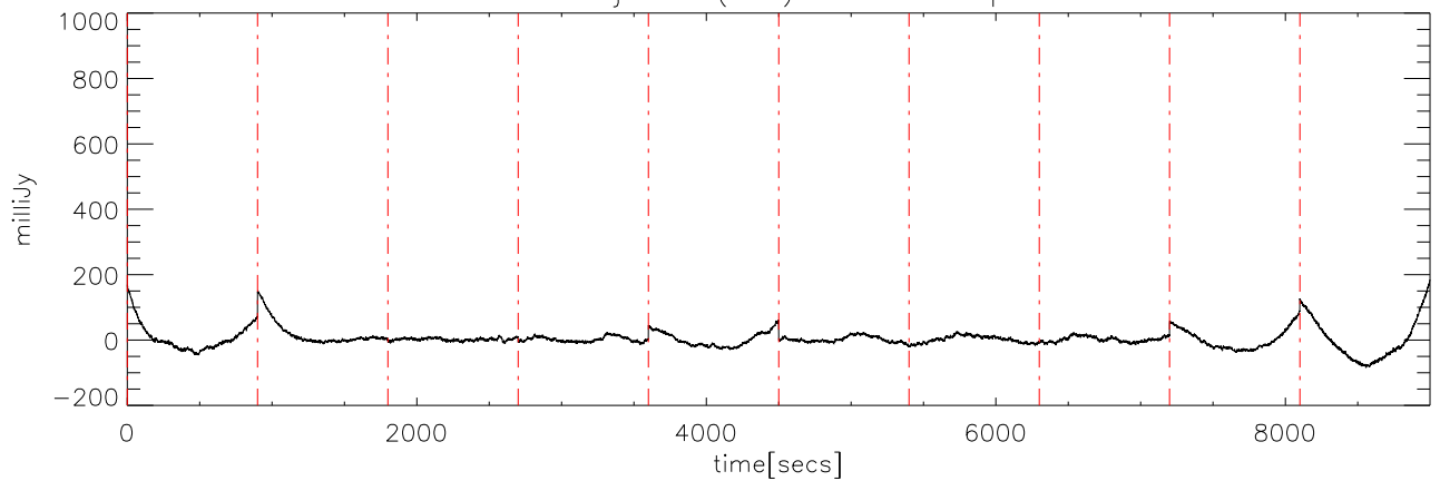
a2414 14jun09 (AST) StokesI freq:3350.
