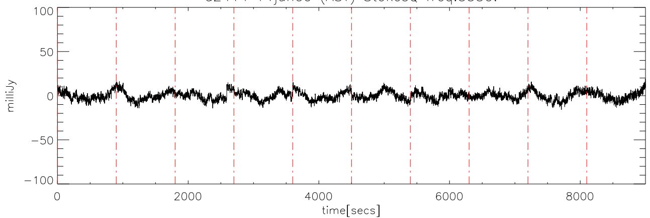
a2414 14jun09 (AST) StokesQ freq:3350.
