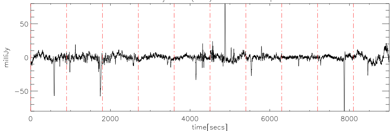
a2414 14jun09 (AST) StokesU freq:3850.
