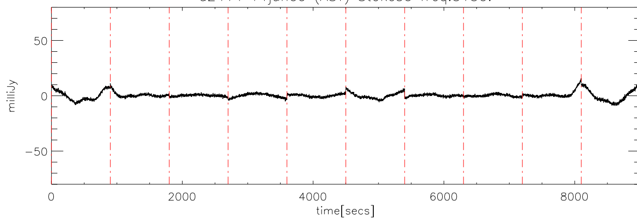
a2414 14jun09 (AST) StokesU freq:3250.
