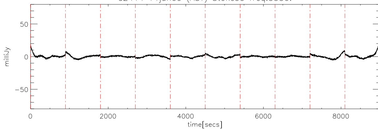
a2414 14jun09 (AST) StokesU freq:3350.
