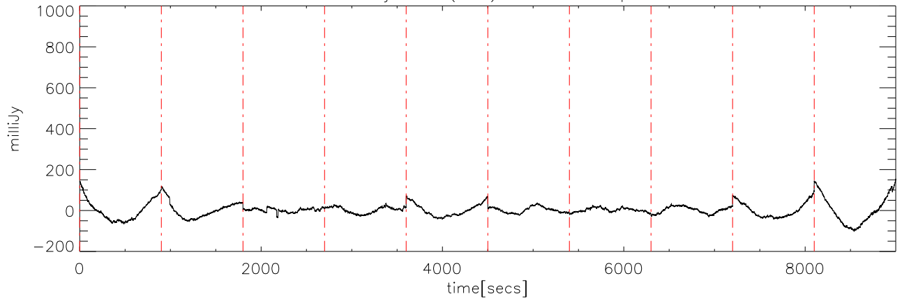
a2414 14jun09 (AST) StokesI freq:3250.
