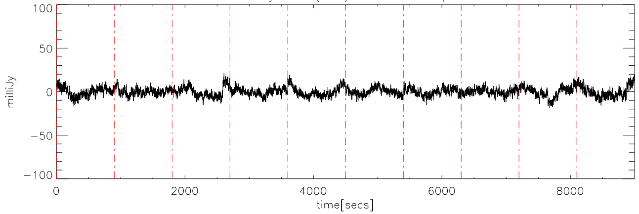
a2414 14jun09 (AST) StokesQ freq:3150.
