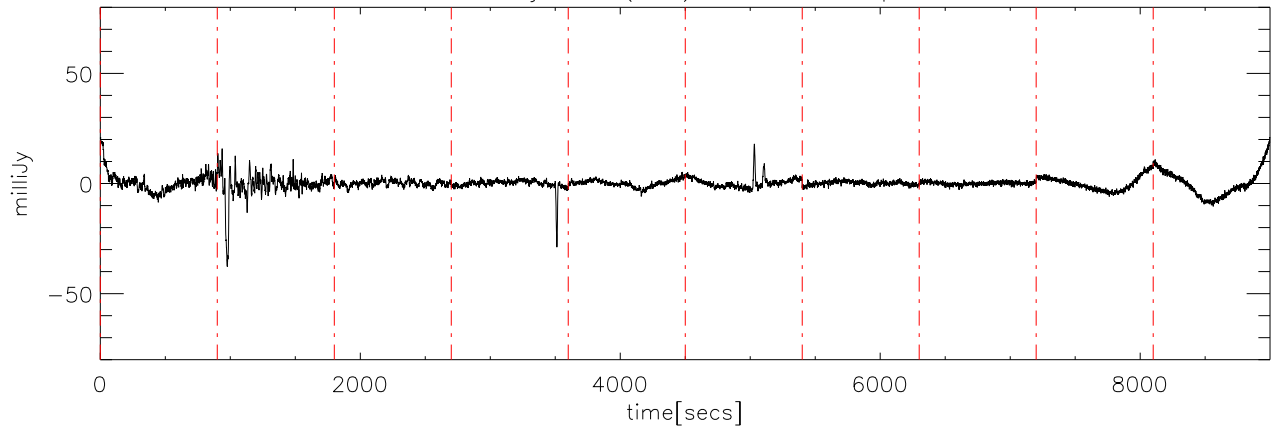
a2414 14jun09 (AST) StokesU freq:3550.
