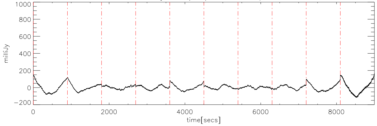
a2414 14jun09 (AST) StokesI freq:3150.
