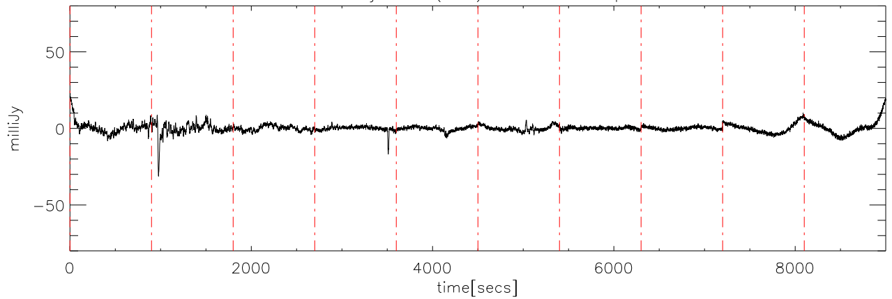
a2414 14jun09 (AST) StokesU freq:3700.
