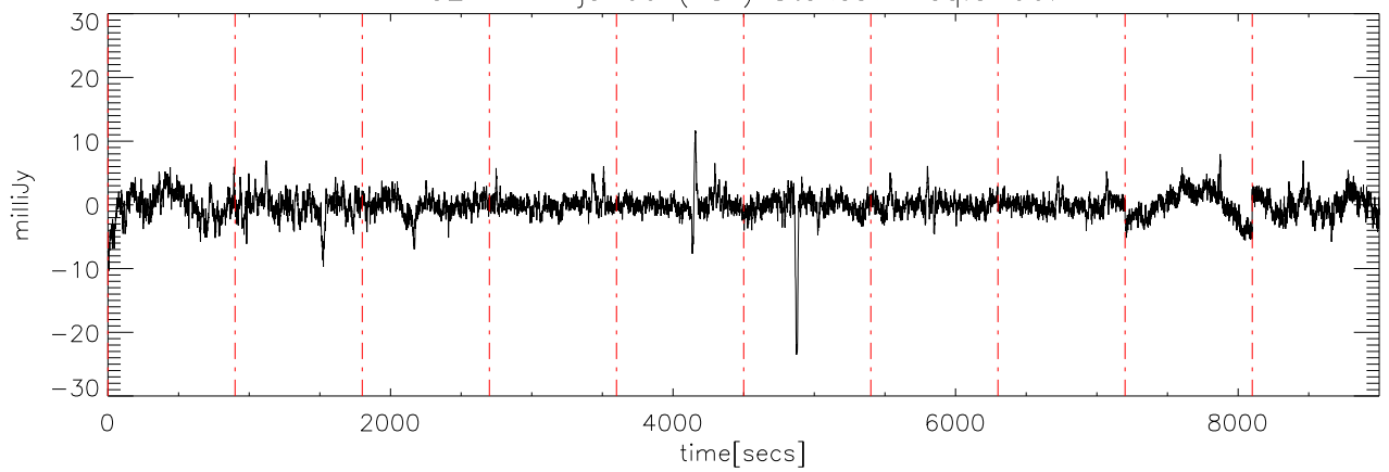
a2414 14jun09 (AST) StokesV freq:3850.
