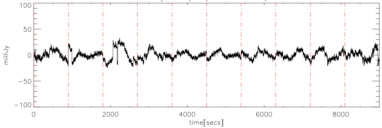
a2414 14jun09 (AST) StokesQ freq:3250.
