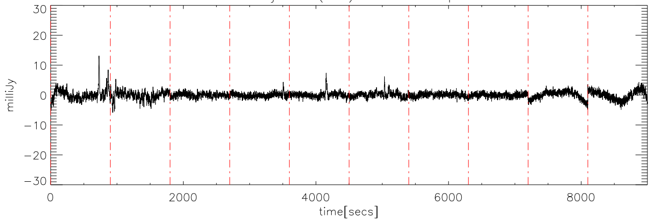
a2414 14jun09 (AST) StokesV freq:3700.
