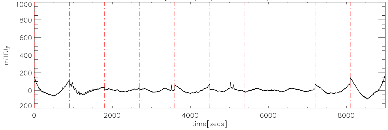
a2414 14jun09 (AST) StokesI freq:3550.
