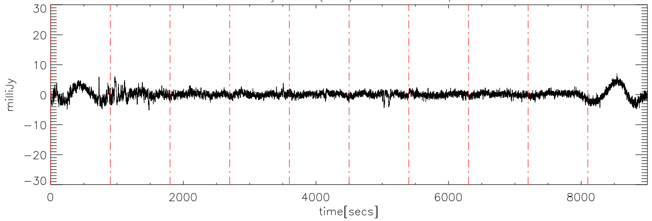
a2414 14jun09 (AST) StokesV freq:3550.
