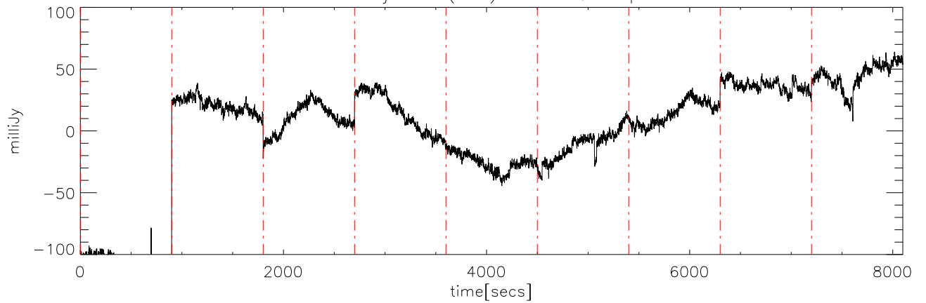
a2414 13jun09 (AST) StokesQ freq:4600.
