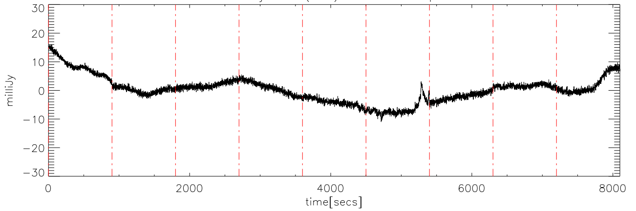
a2414 13jun09 (AST) StokesV freq:5000.
