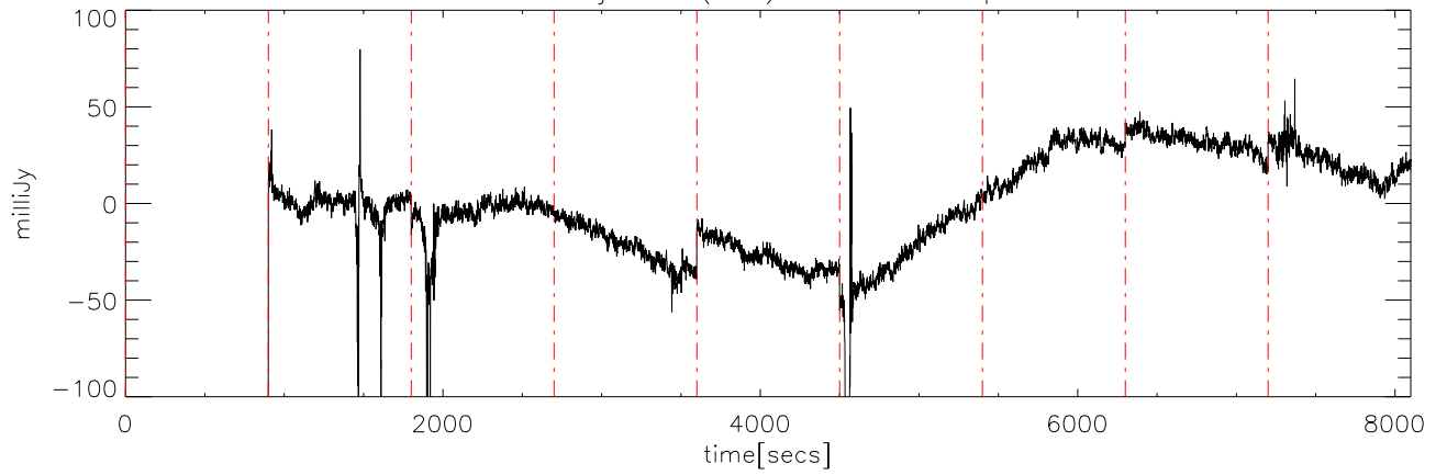
a2414 13jun09 (AST) StokesQ freq:4475.
