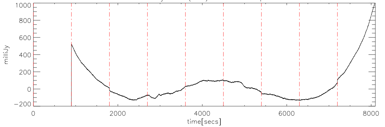
a2414 13jun09 (AST) StokesI freq:5125.
