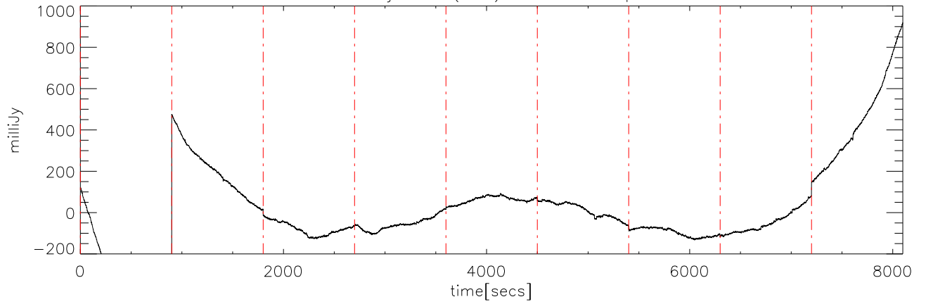
a2414 13jun09 (AST) StokesI freq:4600.
