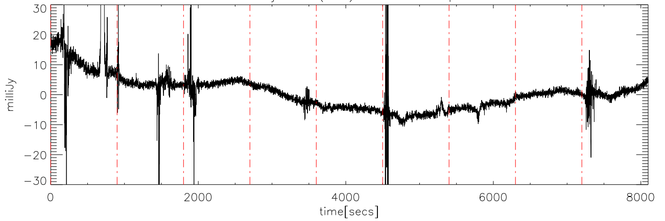
a2414 13jun09 (AST) StokesV freq:4475.
