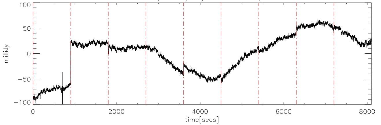
a2414 13jun09 (AST) StokesQ freq:5000.
