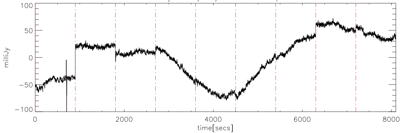
a2414 13jun09 (AST) StokesQ freq:5125.
