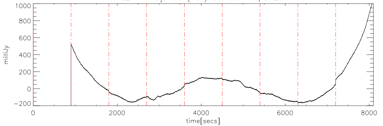
a2414 13jun09 (AST) StokesI freq:5250.
