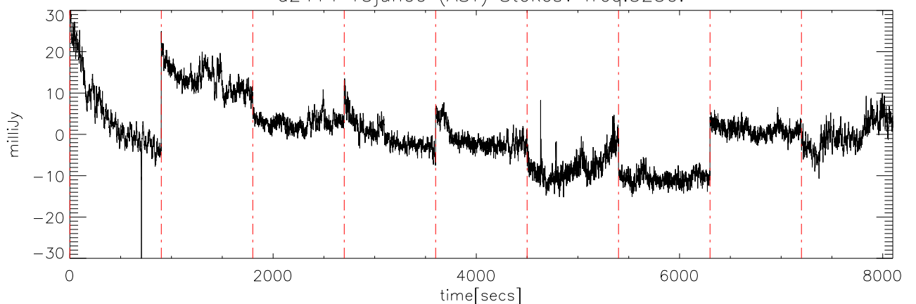
a2414 13jun09 (AST) StokesV freq:5250.
