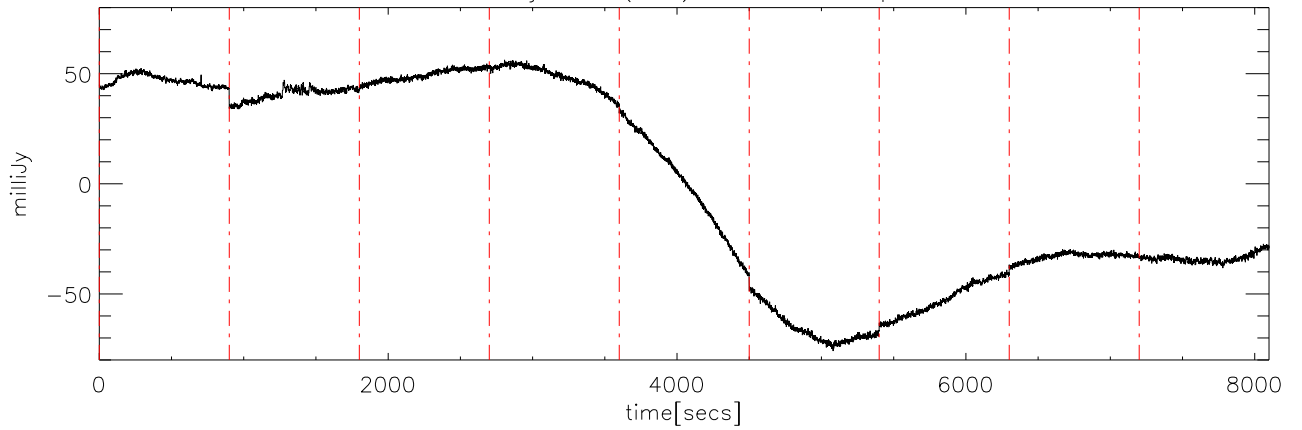
a2414 13jun09 (AST) StokesU freq:5250.
