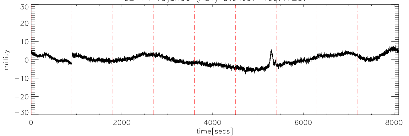
a2414 13jun09 (AST) StokesV freq:4725.
