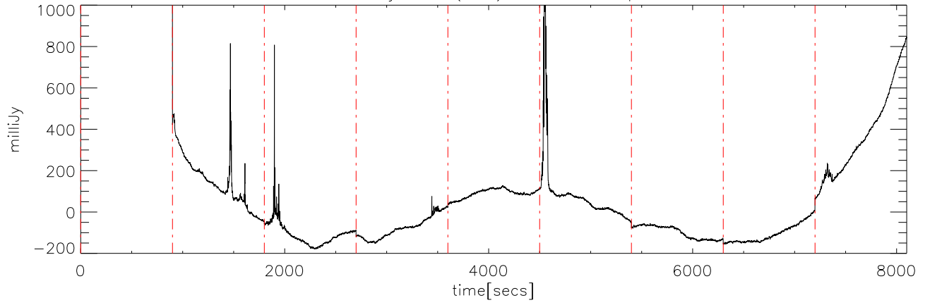
a2414 13jun09 (AST) StokesI freq:4475.
