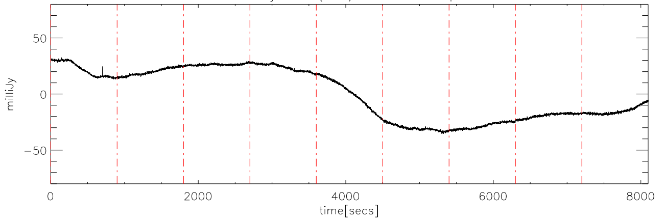
a2414 13jun09 (AST) StokesU freq:4600.
