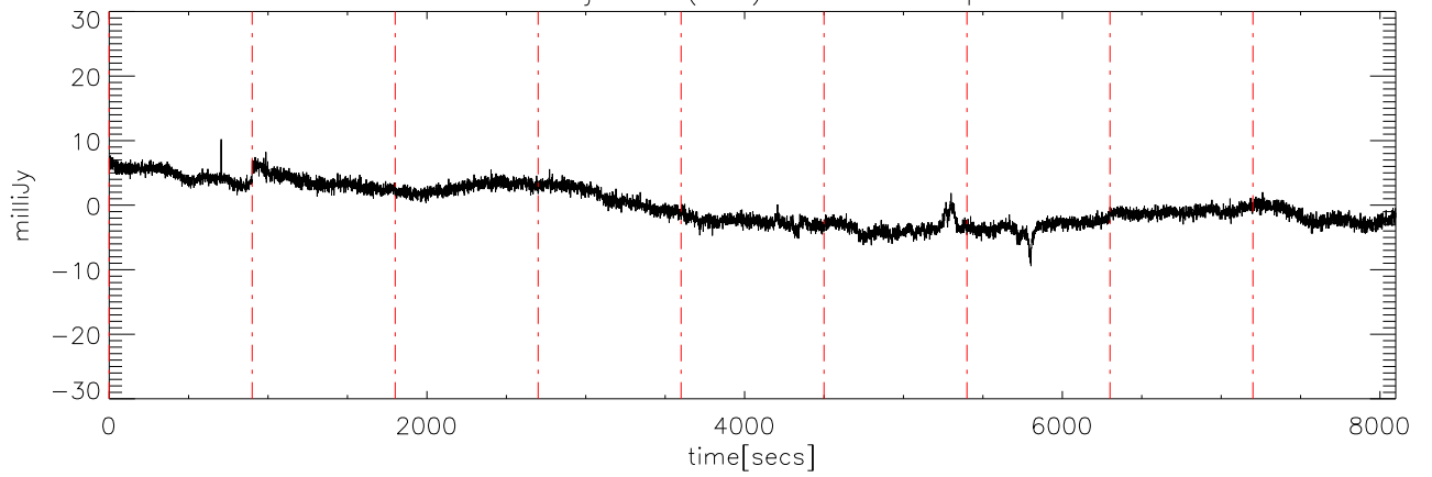
a2414 13jun09 (AST) StokesV freq:4600.
