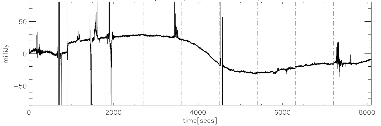
a2414 13jun09 (AST) StokesU freq:4475.
