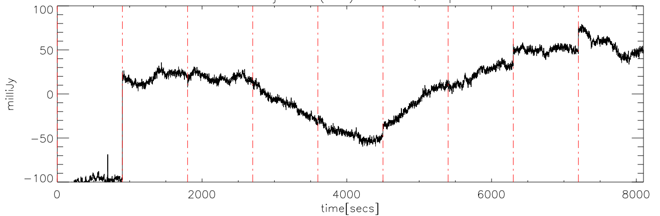
a2414 13jun09 (AST) StokesQ freq:4725.
