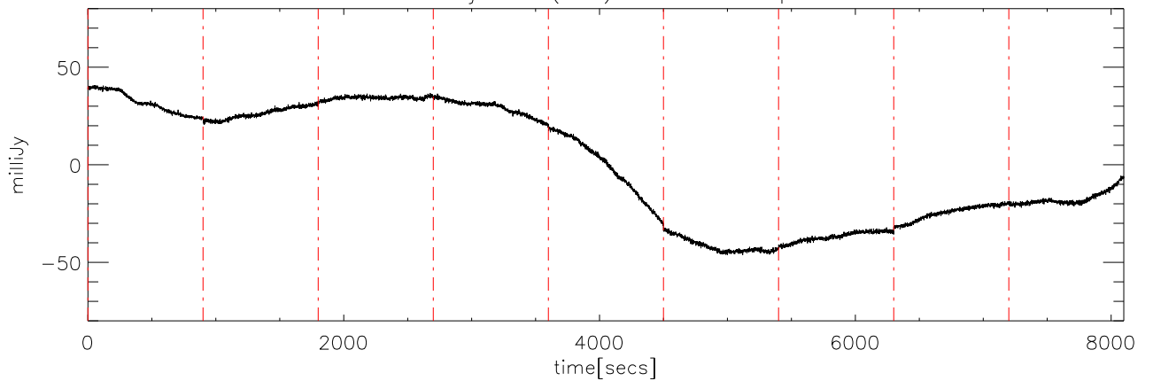
a2414 13jun09 (AST) StokesU freq:4725.
