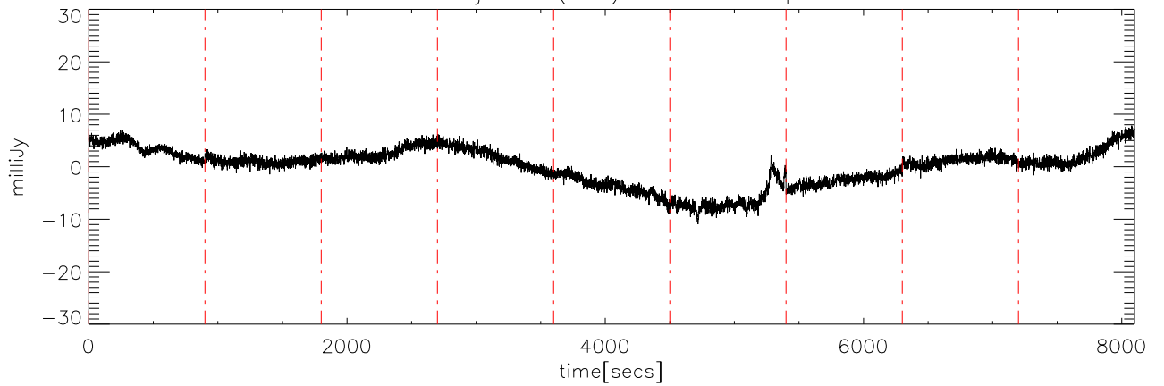
a2414 13jun09 (AST) StokesV freq:5125.
