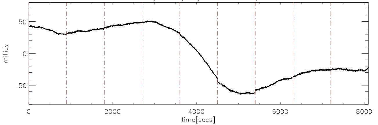
a2414 13jun09 (AST) StokesU freq:5125.
