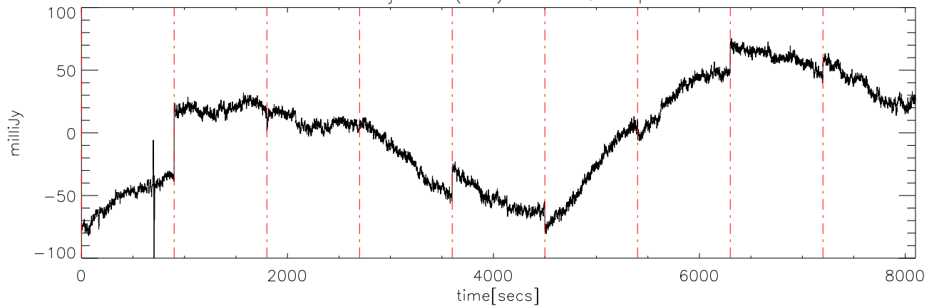
a2414 13jun09 (AST) StokesQ freq:5250.
