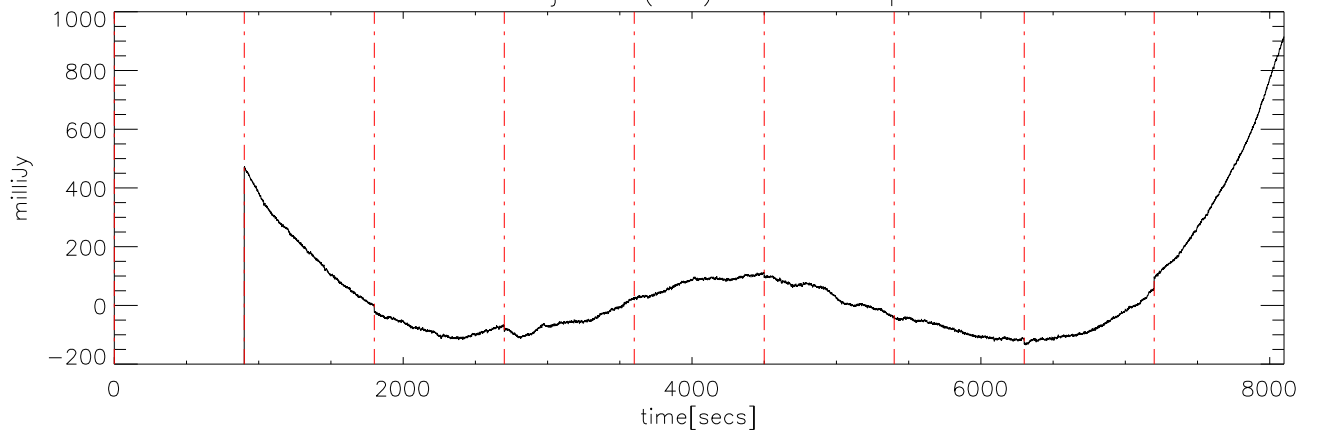
a2414 13jun09 (AST) StokesI freq:4725.
