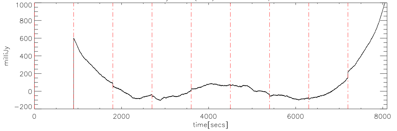
a2414 13jun09 (AST) StokesI freq:5000.
