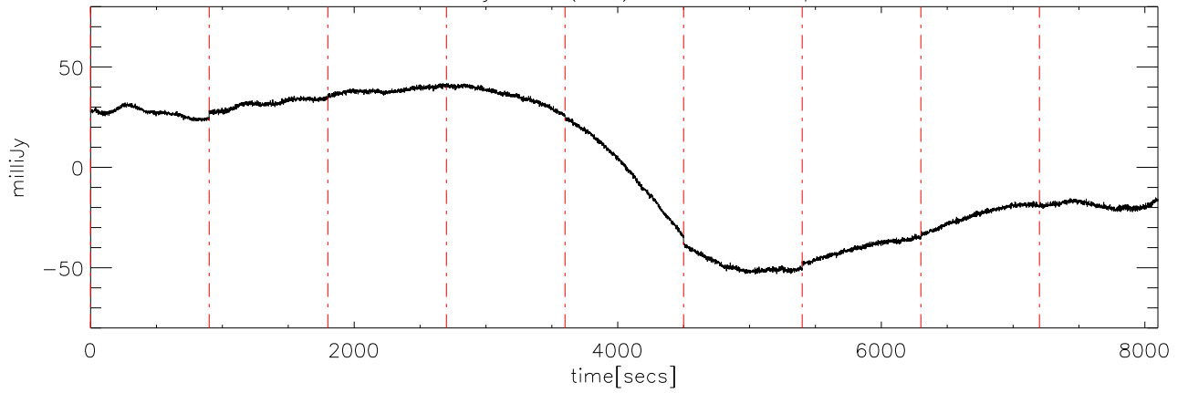
a2414 13jun09 (AST) StokesU freq:5000.
