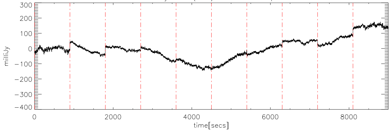
a2414 08jun09 (AST) StokesQ freq:6675.
