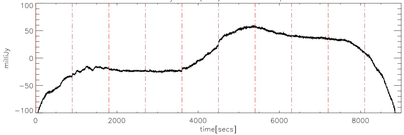
a2414 08jun09 (AST) StokesU freq:7300.
