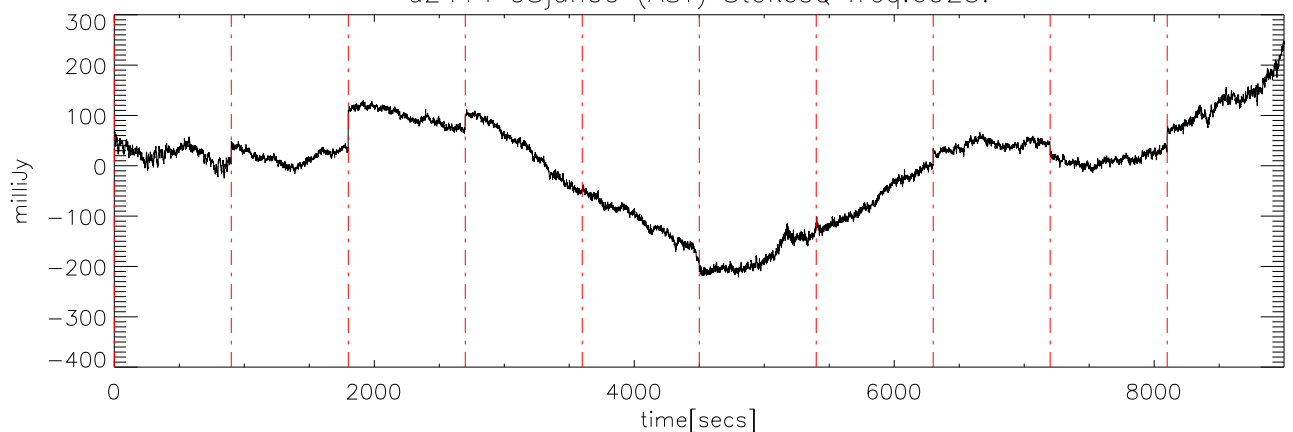
a2414 08jun09 (AST) StokesQ freq:6925.
