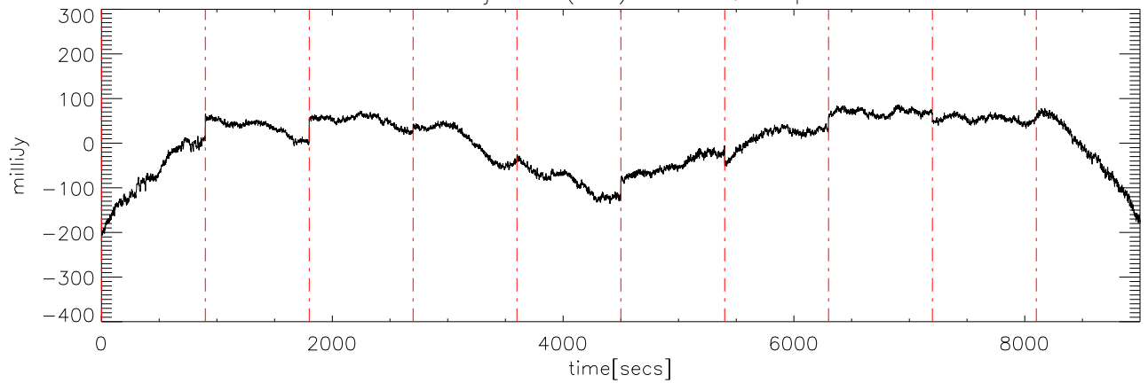
a2414 08jun09 (AST) StokesQ freq:6800.
