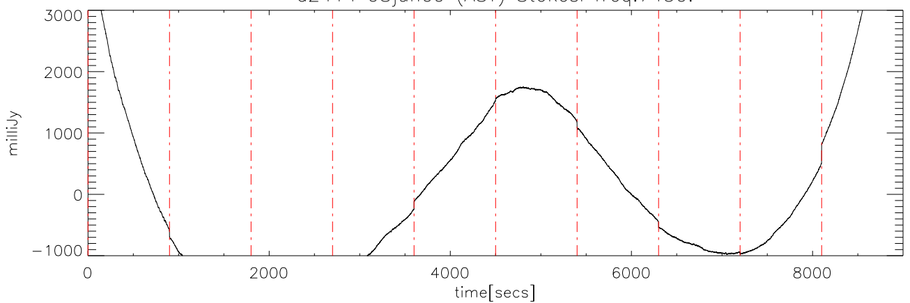
a2414 08jun09 (AST) StokesI freq:7450.
