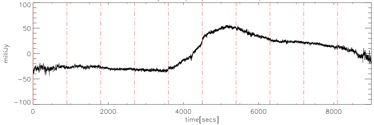
a2414 08jun09 (AST) StokesU freq:7175.
