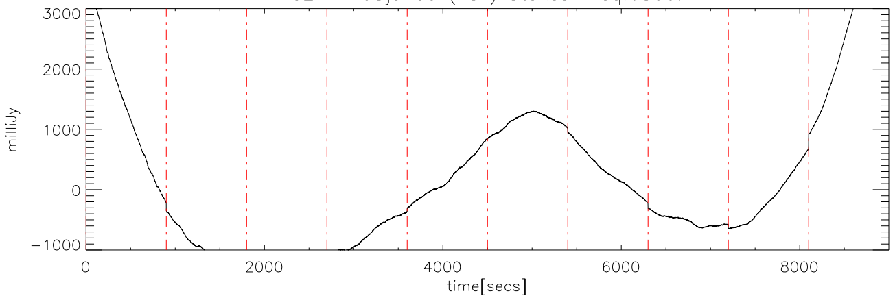
a2414 08jun09 (AST) StokesI freq:6925.
