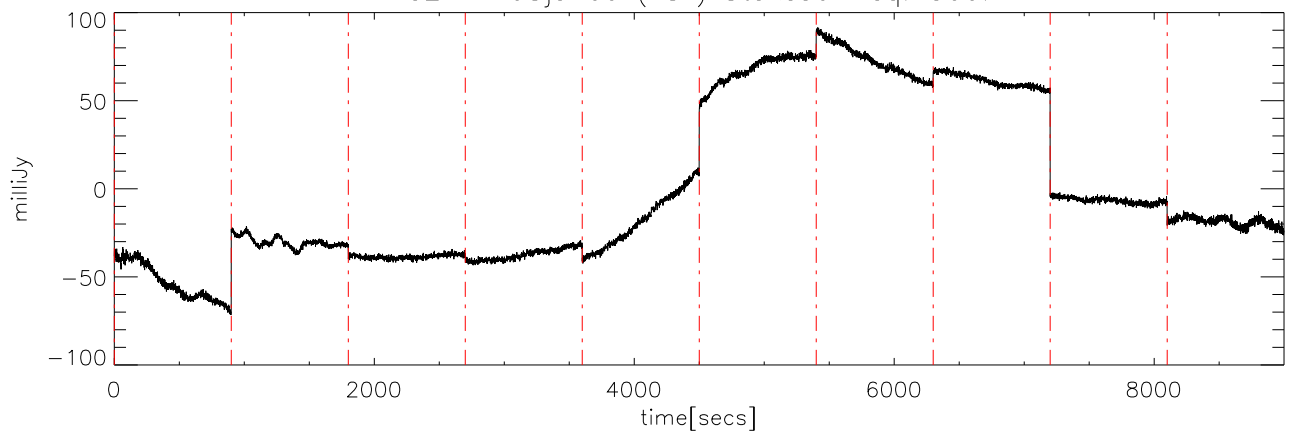
a2414 08jun09 (AST) StokesU freq:7450.
