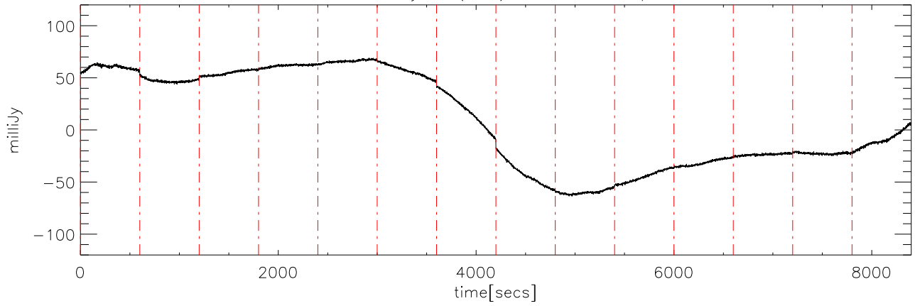
a2327 18may08 (AST) StokesU freq:5125.
