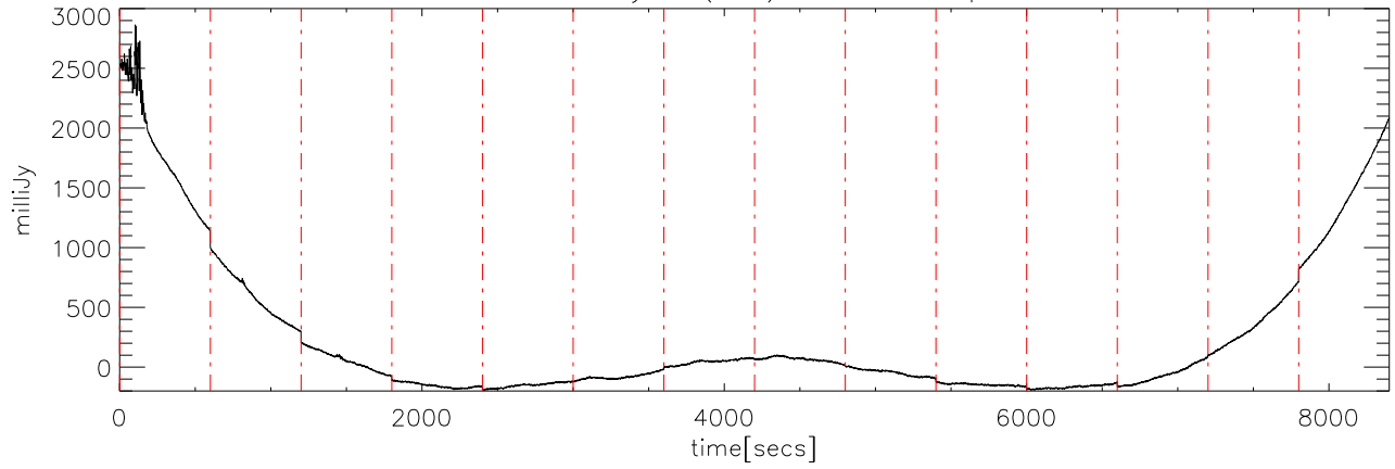
a2327 18may08 (AST) StokesI freq:4475.
