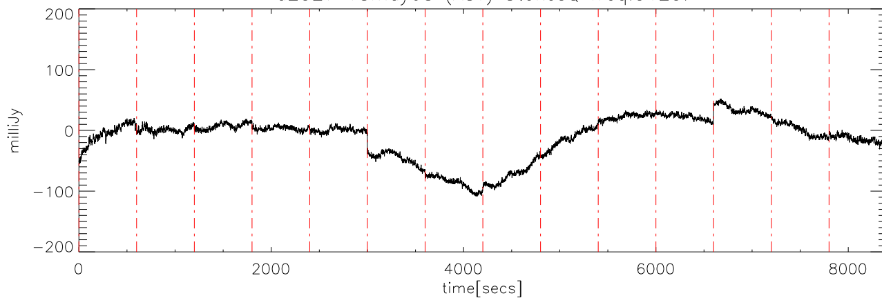
a2327 18may08 (AST) StokesQ freq:5250.
