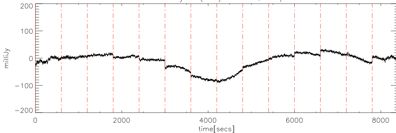
a2327 18may08 (AST) StokesQ freq:5000.
