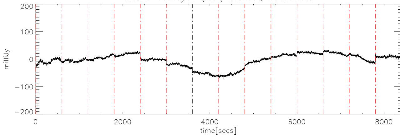
a2327 18may08 (AST) StokesQ freq:4725.
