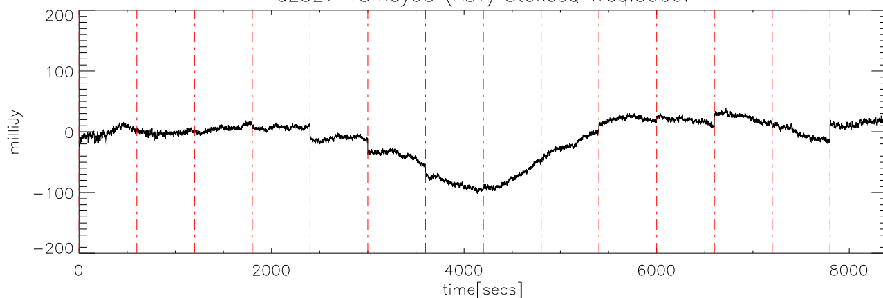
a2327 18may08 (AST) StokesQ freq:5125.
