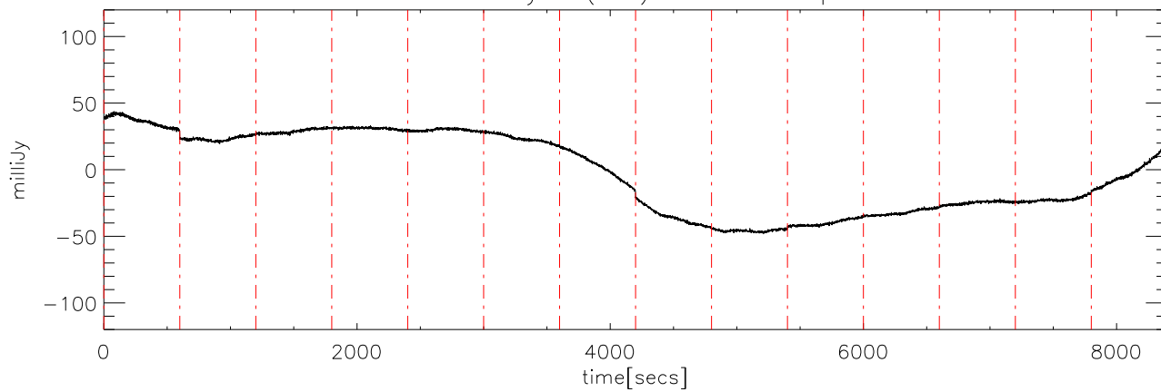
a2327 18may08 (AST) StokesU freq:4725.
