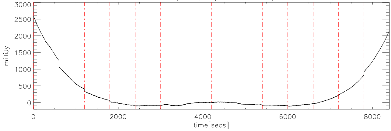
a2327 18may08 (AST) StokesI freq:5000.
