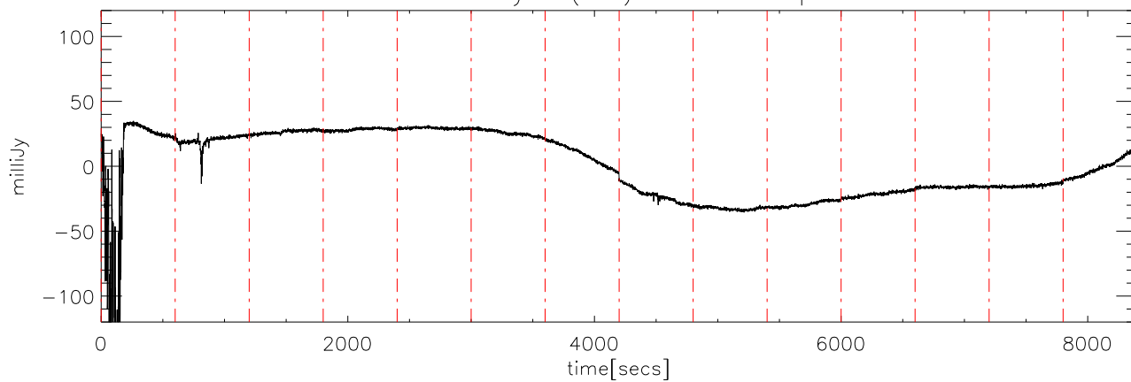
a2327 18may08 (AST) StokesU freq:4475.
