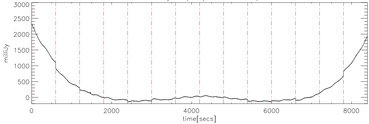
a2327 18may08 (AST) StokesI freq:4725.
