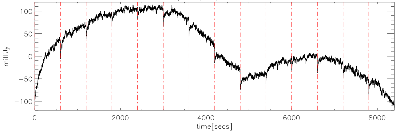
a2327 18may08 (AST) StokesU freq:5250.
