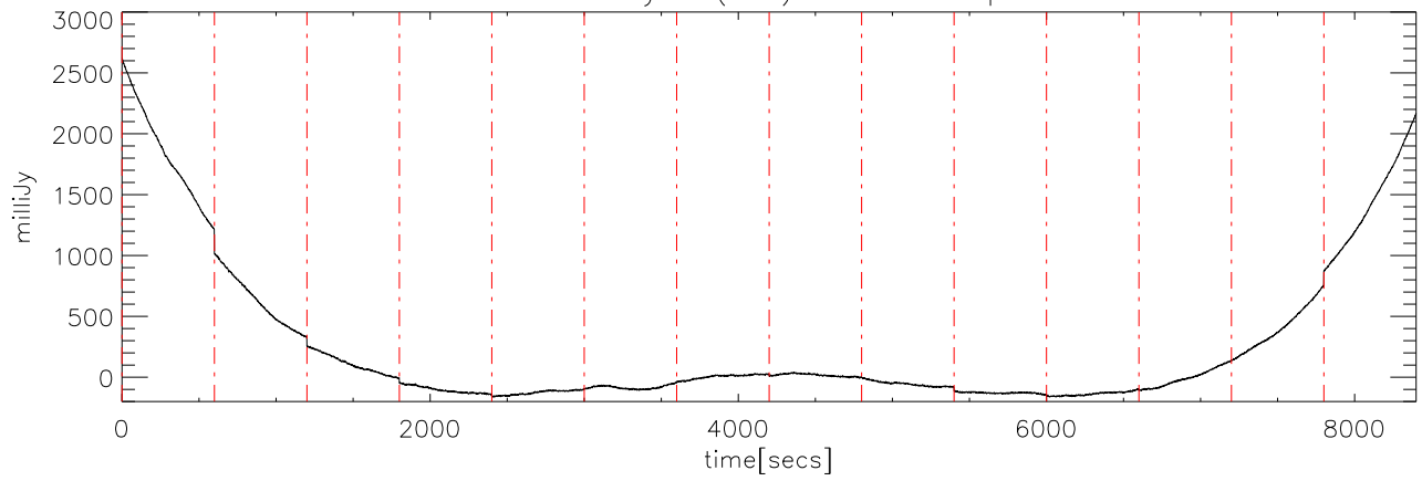
a2327 18may08 (AST) StokesI freq:5125.
