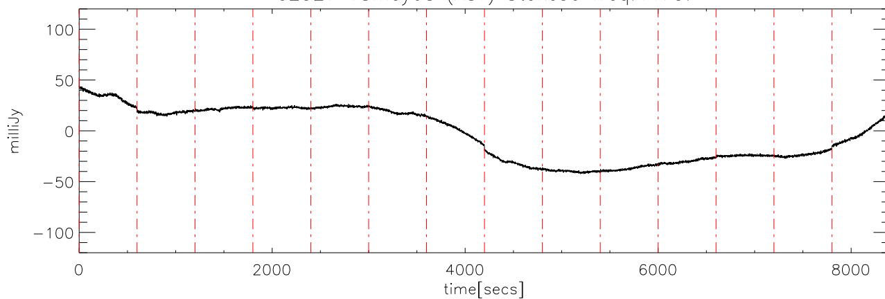
a2327 18may08 (AST) StokesU freq:4600.
