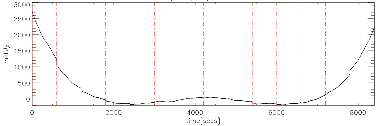
a2327 18may08 (AST) StokesI freq:5250.
