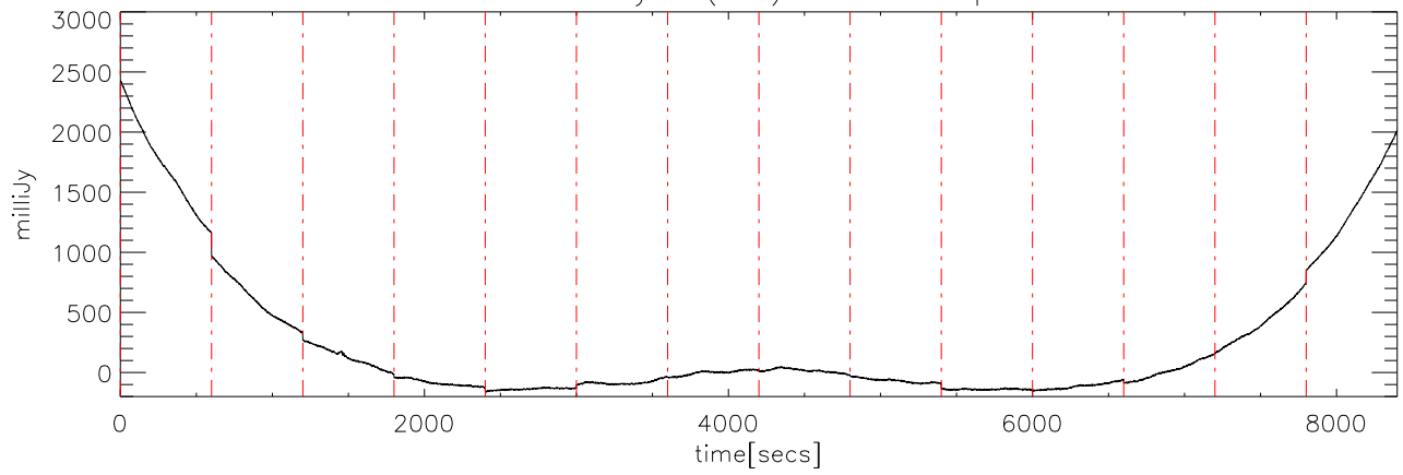
a2327 18may08 (AST) StokesI freq:4600.
