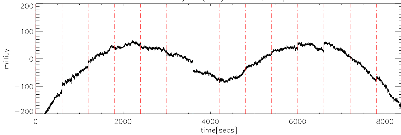
a2327 18may08 (AST) StokesQ freq:4475.
