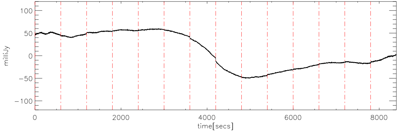
a2327 18may08 (AST) StokesU freq:5000.
