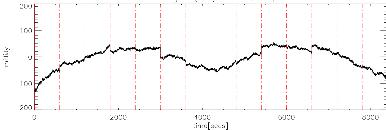
a2327 18may08 (AST) StokesQ freq:4600.
