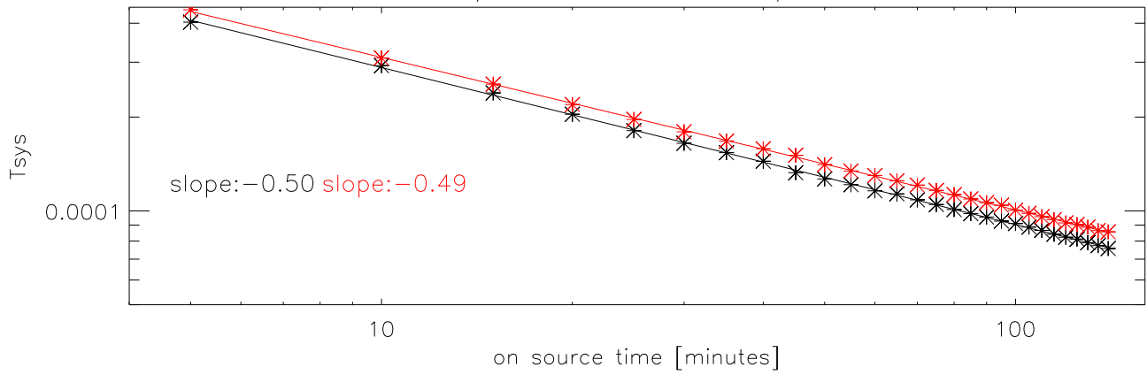
8127. on/off rms vs number pairs added
