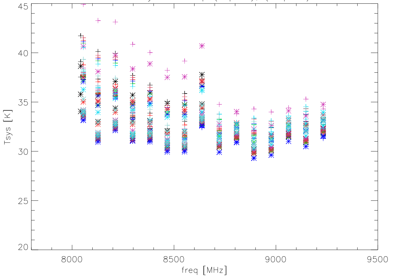
A2228 Tsys vs Freq. (* polA), (+ polB)
