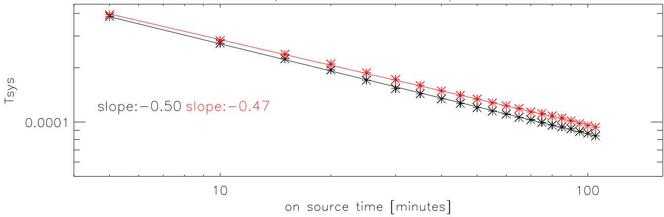
9147. on/off rms vs number pairs added
