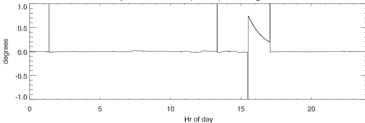
position error \text{abs}(\text{encVel}) < .003\text{deg/sec}
