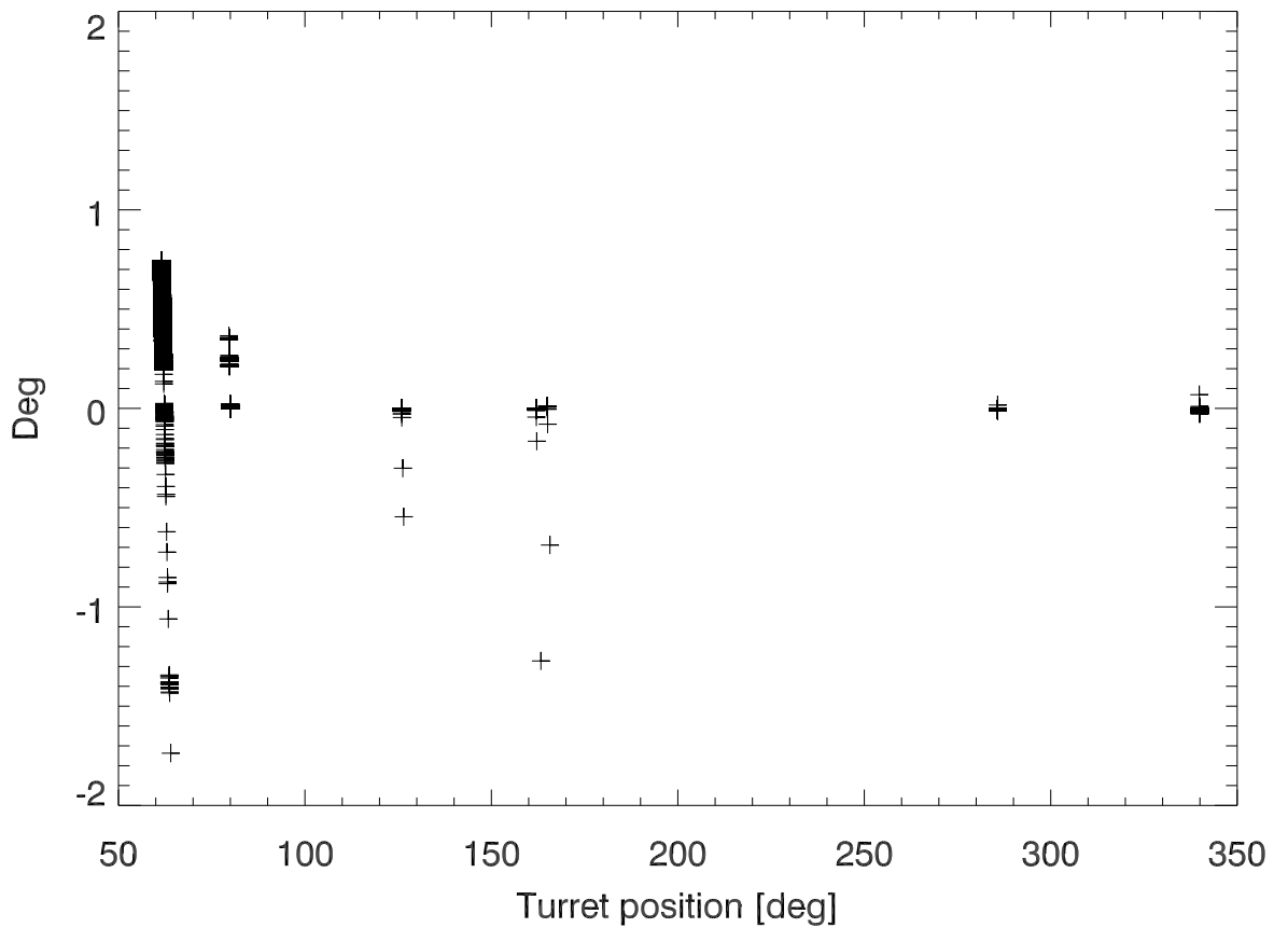
23jul20 turret positoin error when turvel < 2 counts
