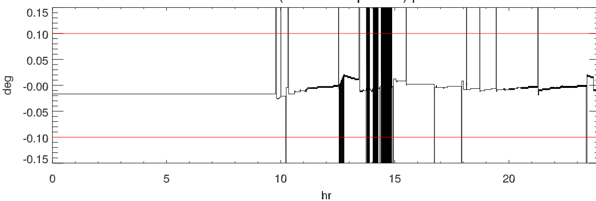
170203 turret (Actual - Requested) position
