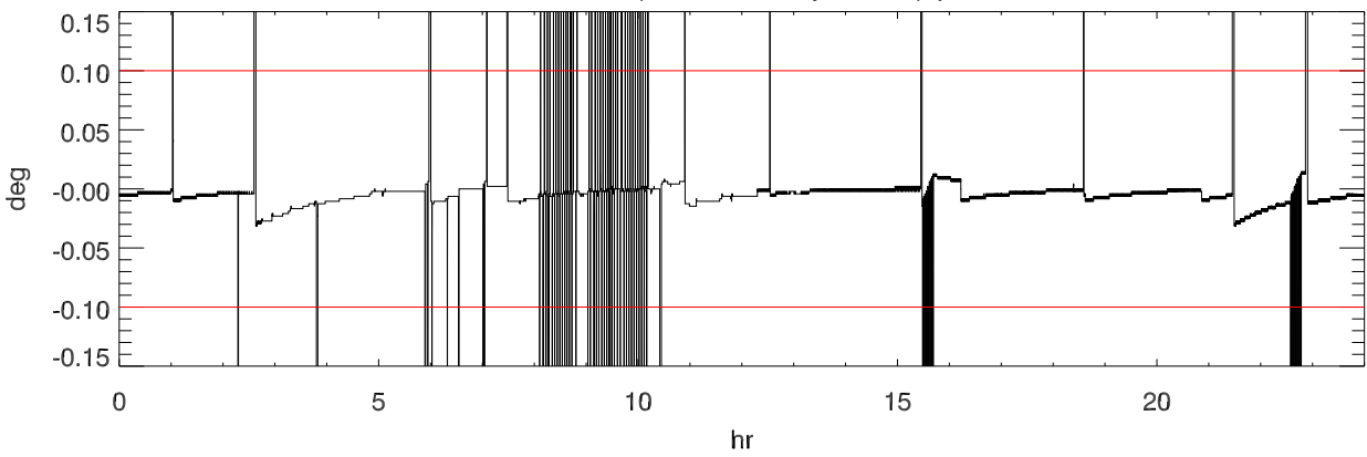
170209 turret (Actual - Requested) position
