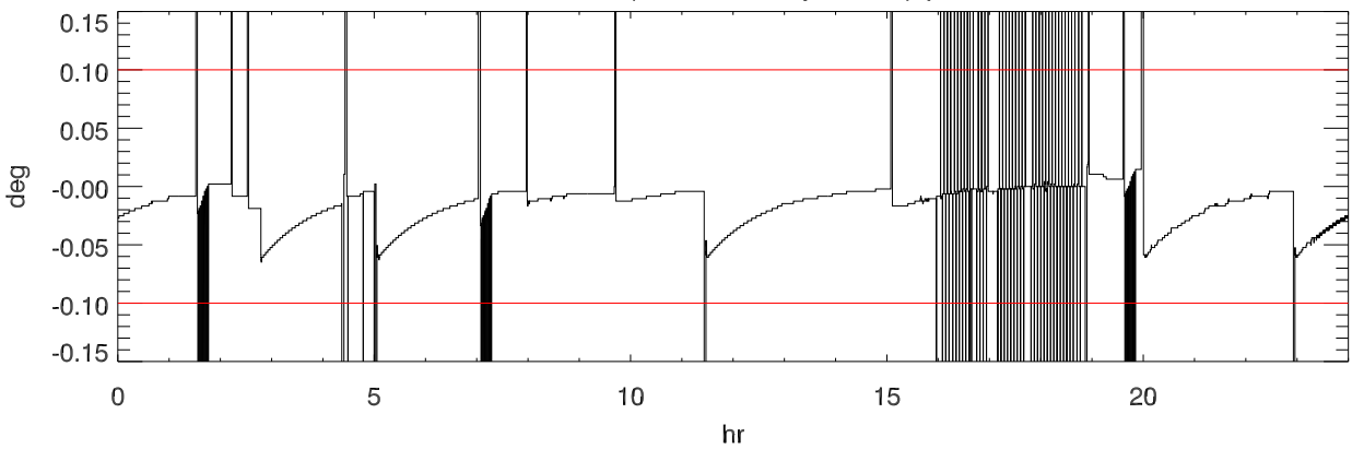
170217 turret (Actual - Requested) position
