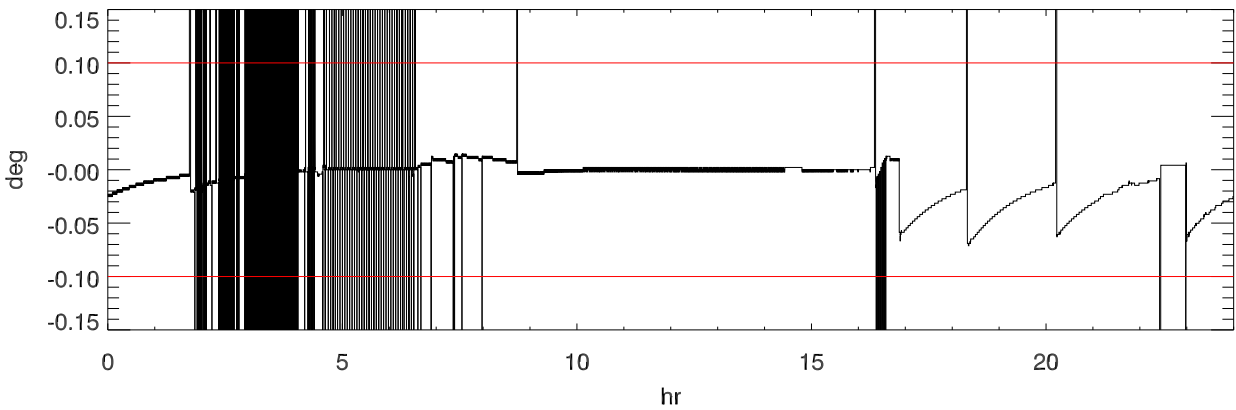
170214 turret (Actual - Requested) position
