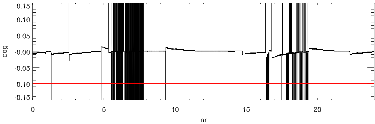
170206 turret (Actual - Requested) position
