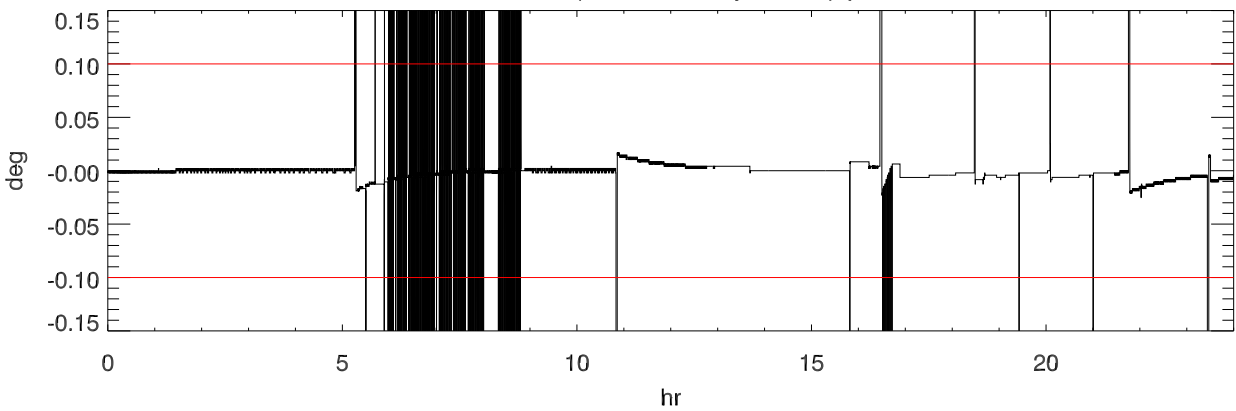
170207 turret (Actual - Requested) position
