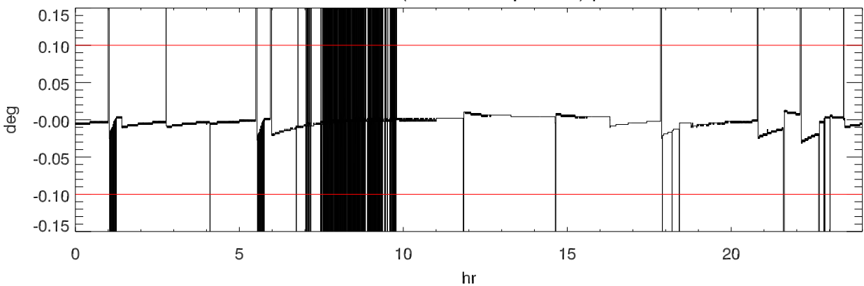
170208 turret (Actual - Requested) position
