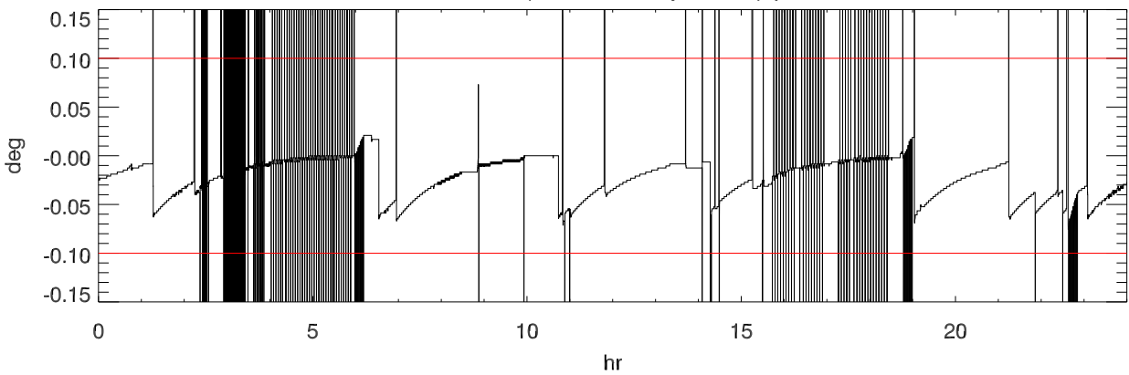
170215 turret (Actual - Requested) position
