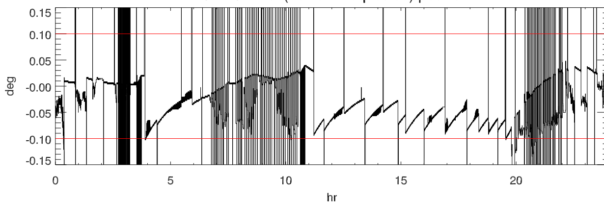
151129 turret (Actual - Requested) position
