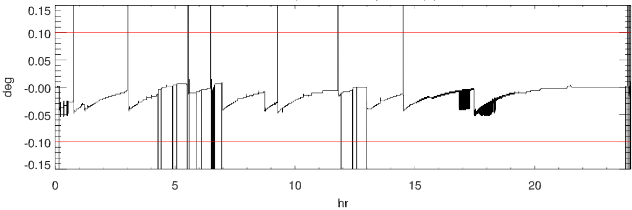
151119 turret (Actual - Requested) position
