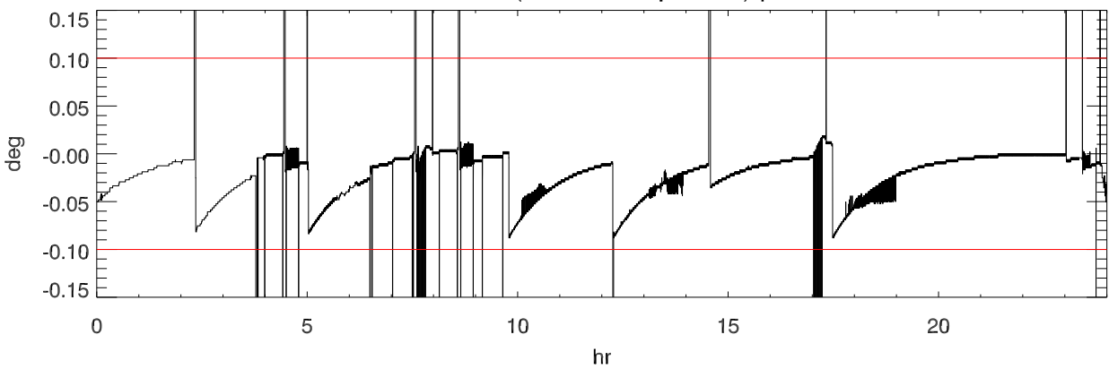
151128 turret (Actual - Requested) position
