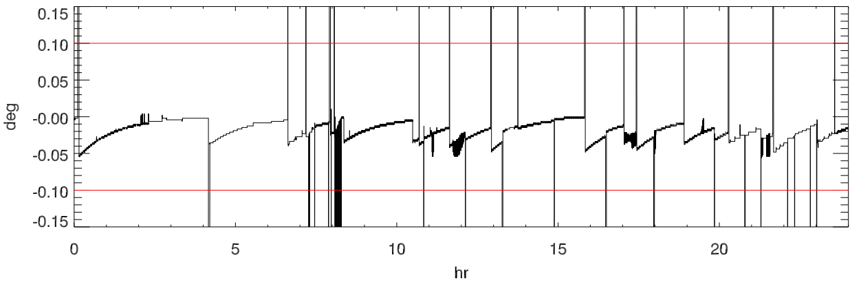
151122 turret (Actual - Requested) position
