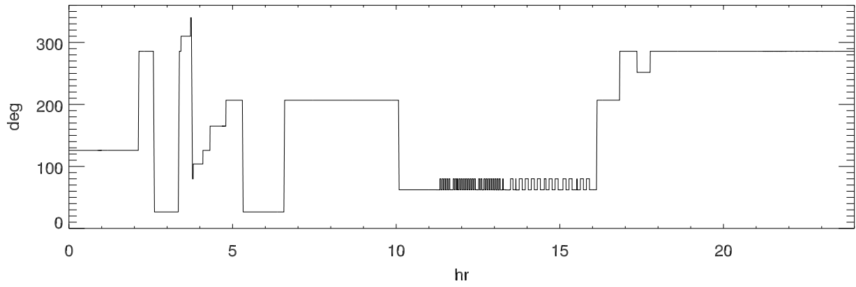
151125 turret (Actual - Requested) position
