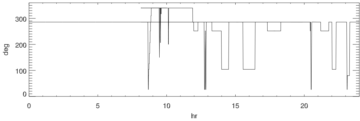
151108 turret (Actual - Requested) position
