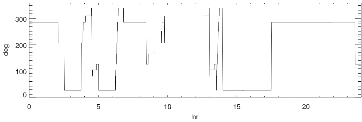
151126 turret (Actual - Requested) position
