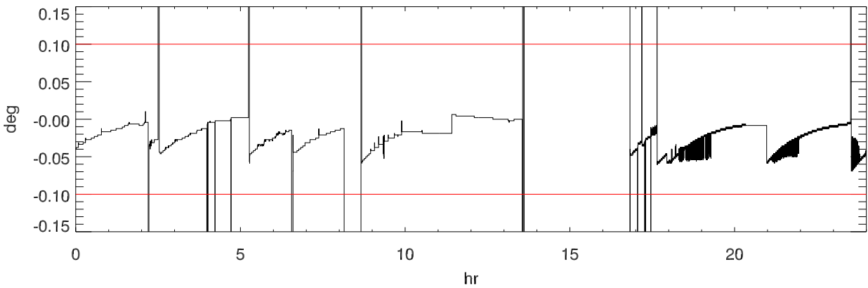
151124 turret (Actual - Requested) position
