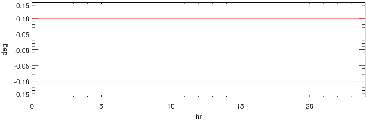
151111 turret (Actual - Requested) position
