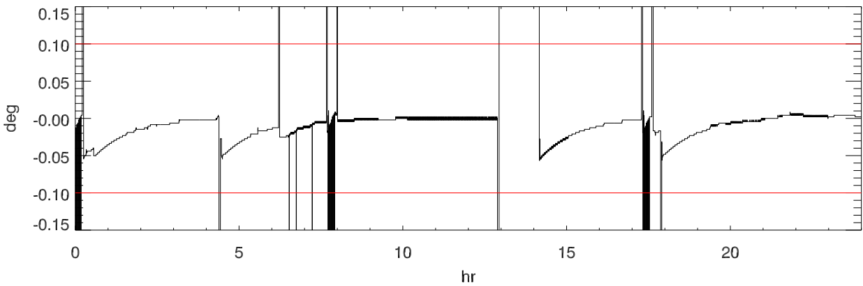
151120 turret (Actual - Requested) position
