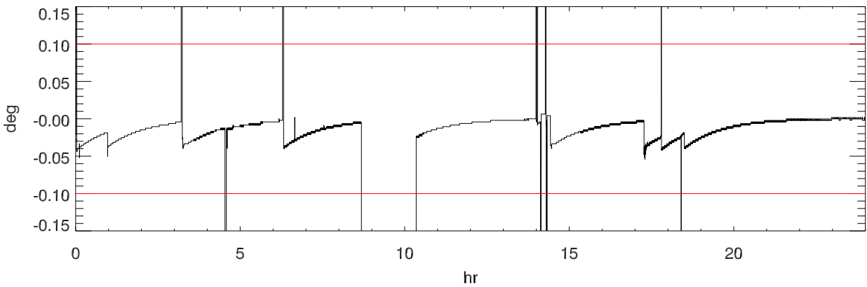
151118 turret (Actual - Requested) position
