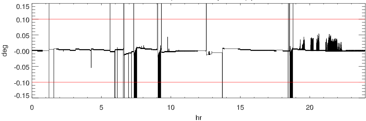
151106 turret (Actual - Requested) position
