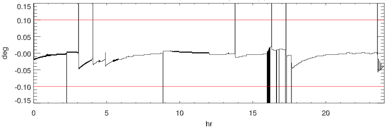
151123 turret (Actual - Requested) position
