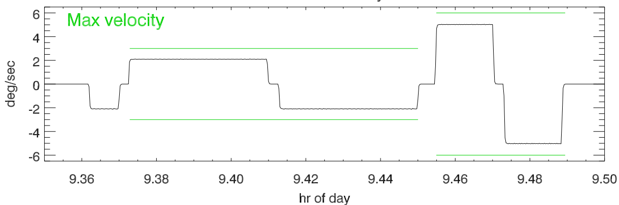
Turrent encoder velocity vs time
