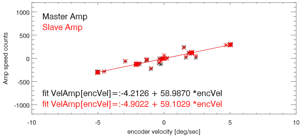
Amplifier speed monitor value vs encoder Velocity
