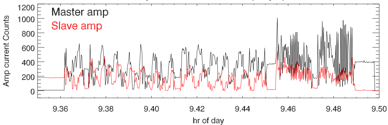
Amplifier current feedback (torque)
