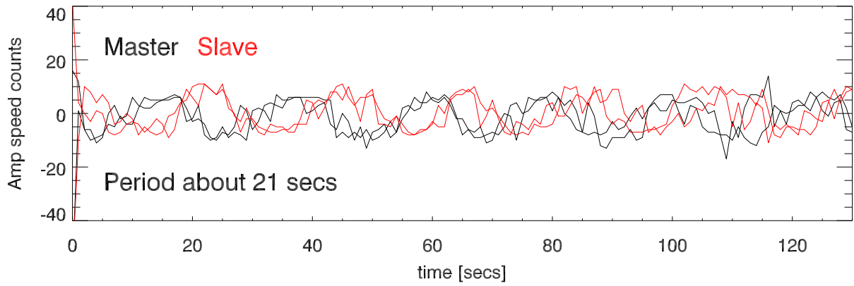
Amp speed for +/- 3deg/sec (remove mean)
