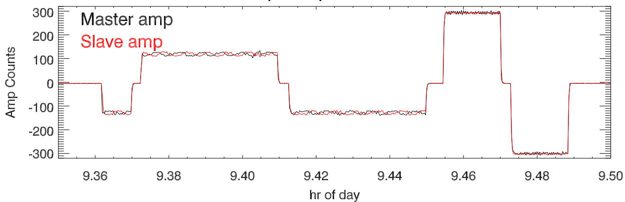
Amplifier speed feedback
