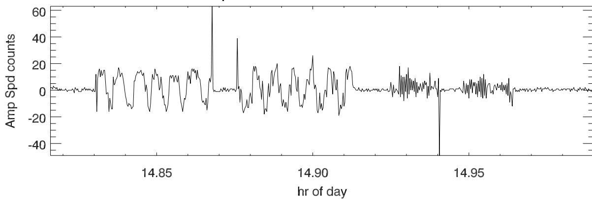
Speed difference Master - slave
