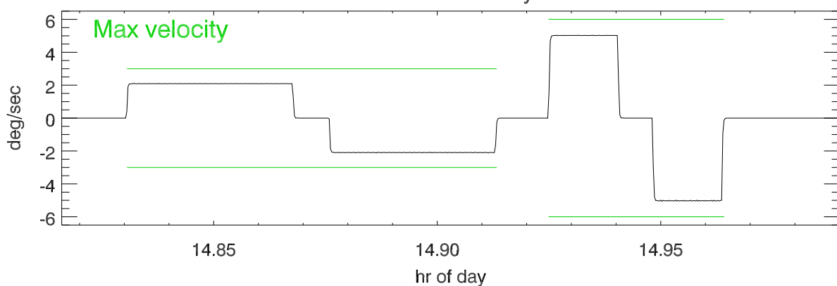
Turrent encoder velocity vs time
