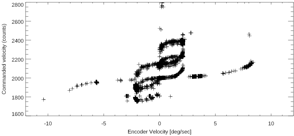
180501 - 180529 turret data. Commanded velocity vs encoder velocity
