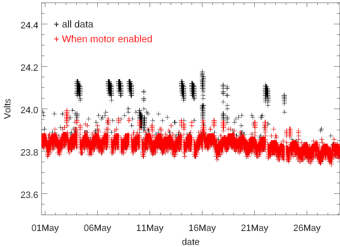
180501 - 180529 turret + 24 Volt power supply vs date
