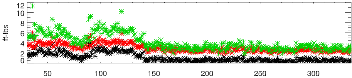
Motor torques vs turret position
