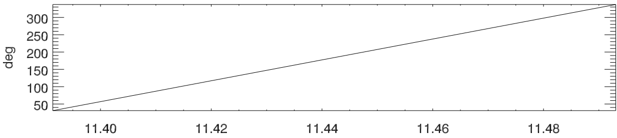
CCW turMaxVel=2deg/sec. Turret position vs hour
