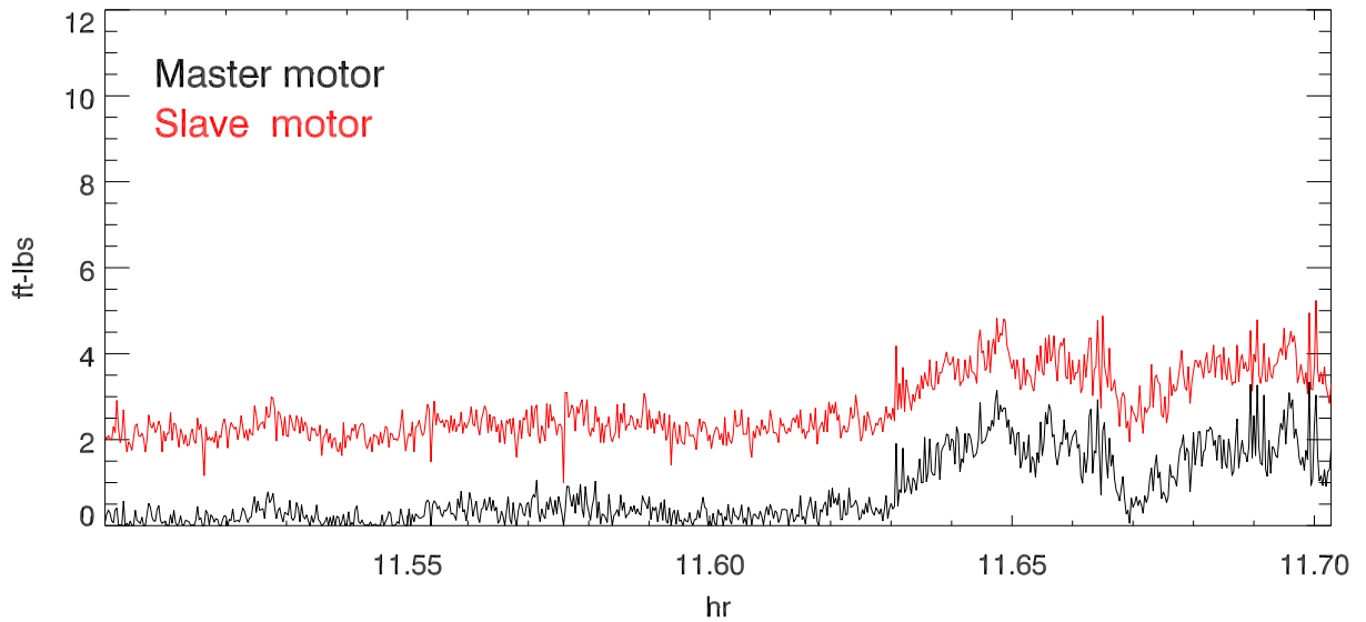
Motor torques vs hour
