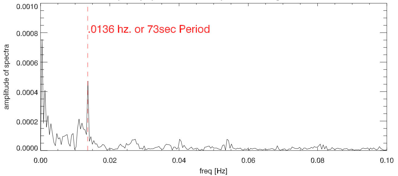
frequency spectrum of turret position during oscillation
