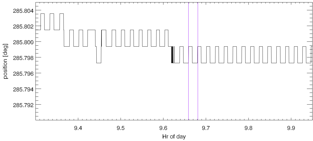
30oct19. Turret position while sitting at lbw rcvr
