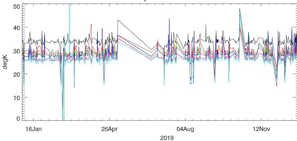
alfa Tsys for 2019 PoIB
