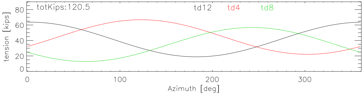
dome za= 5.0
