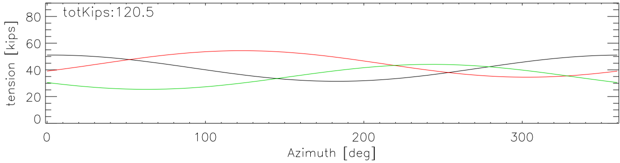
dome za=10.0
