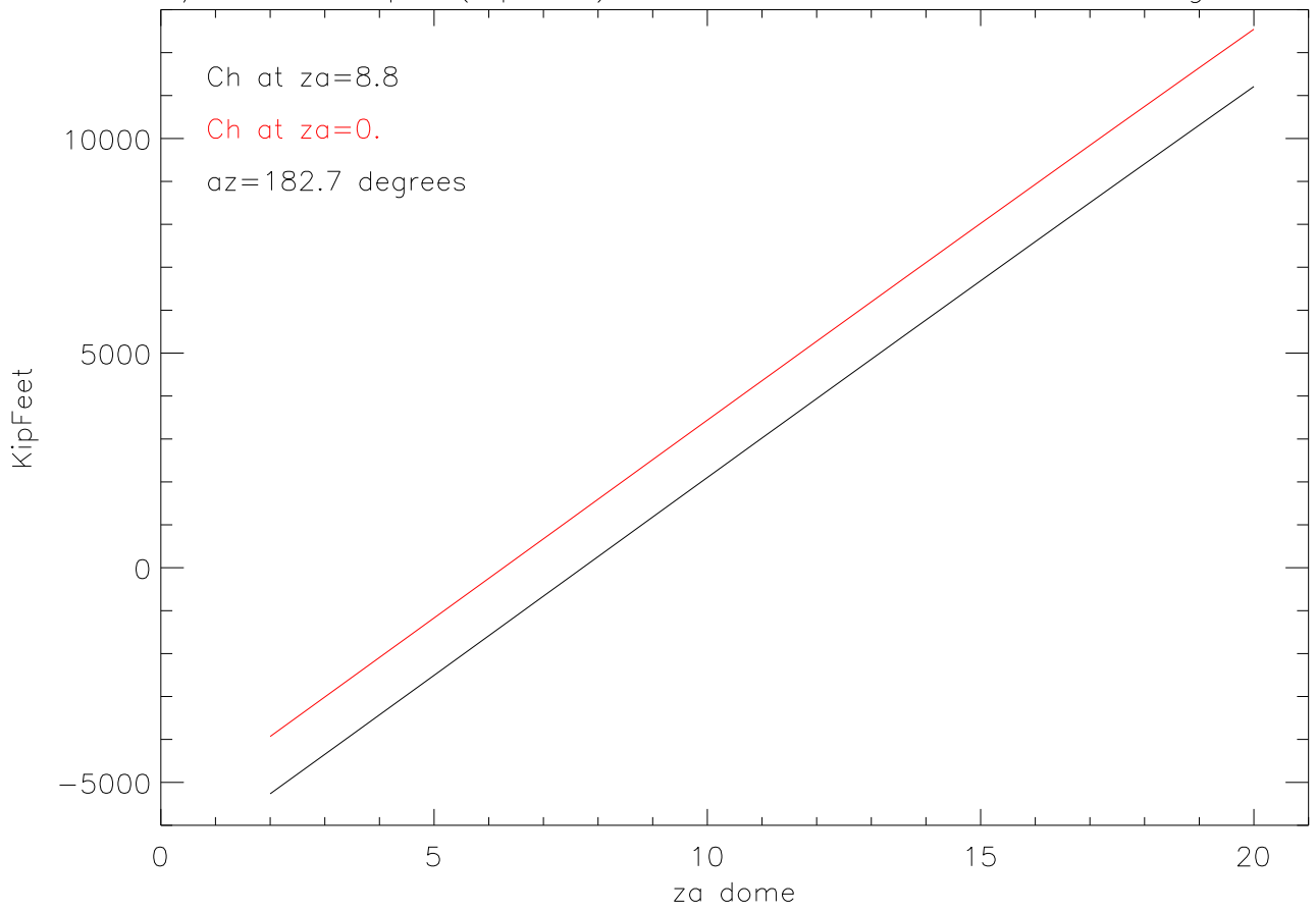
North/South torque (kipFeet) from TieDowns when dome za goes 2–20
