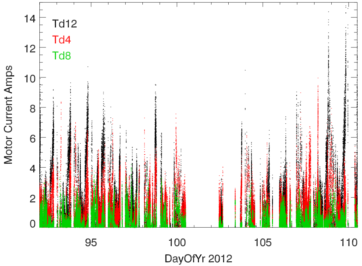
01mar12-19apr12 tiedown motor torques vs daynumber
