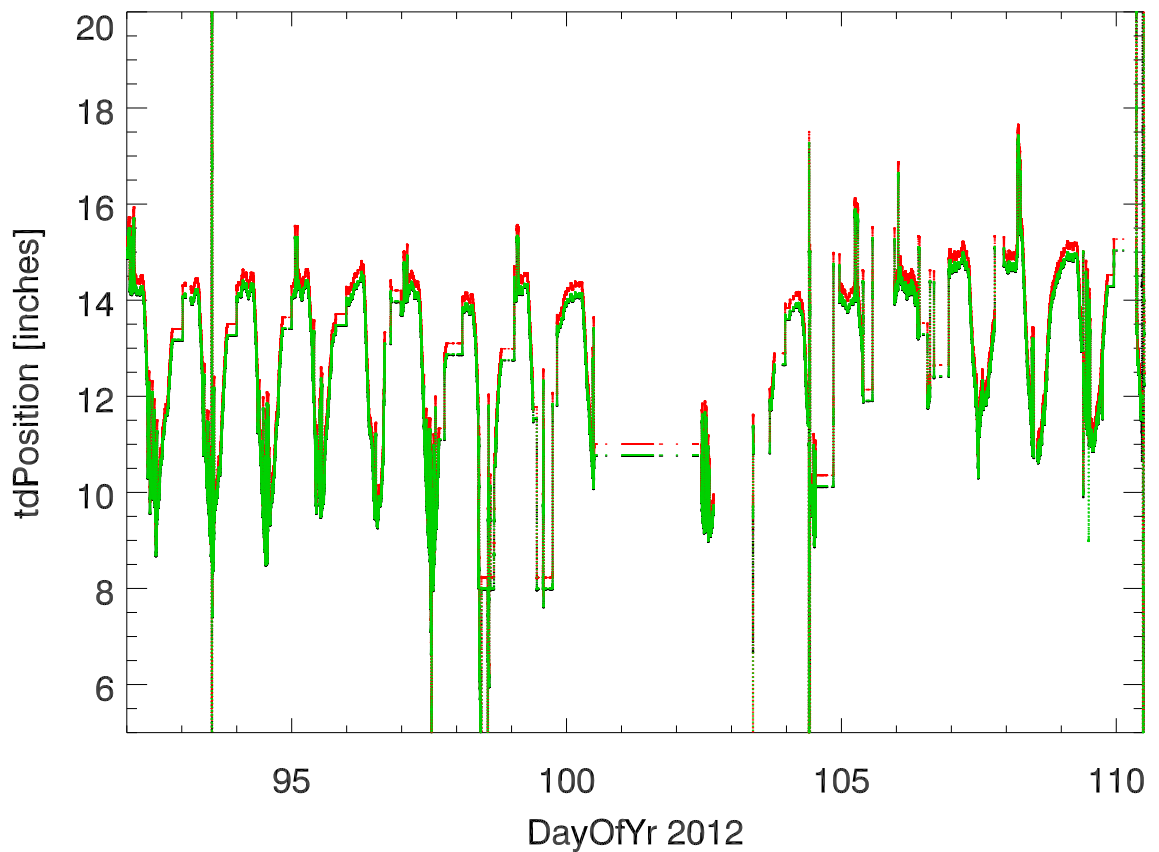
tiedown position vs daynumber
