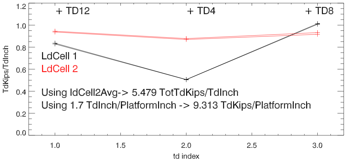
Measured tdKips/TdInch from linear fit to ramps
