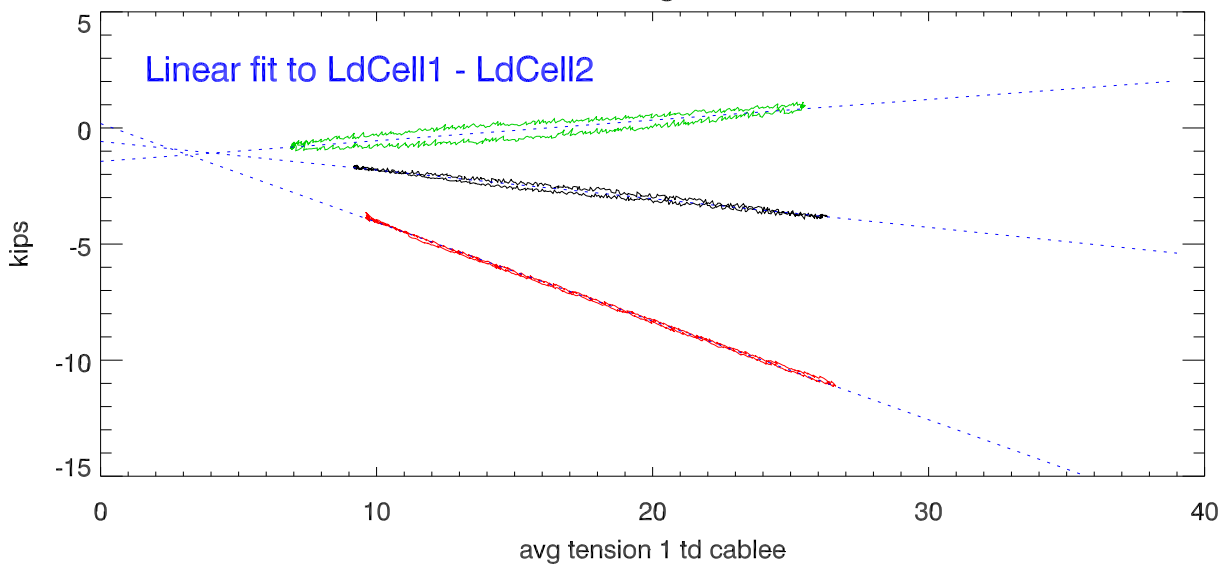
LdCell1 - LdCell2 during the 3-22 inch moves
