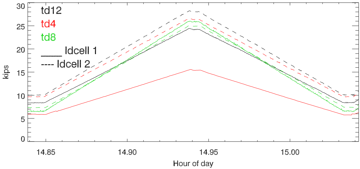
191118 tension when ramping Td's 3 to 22 inches (@ .06 inches/second)
