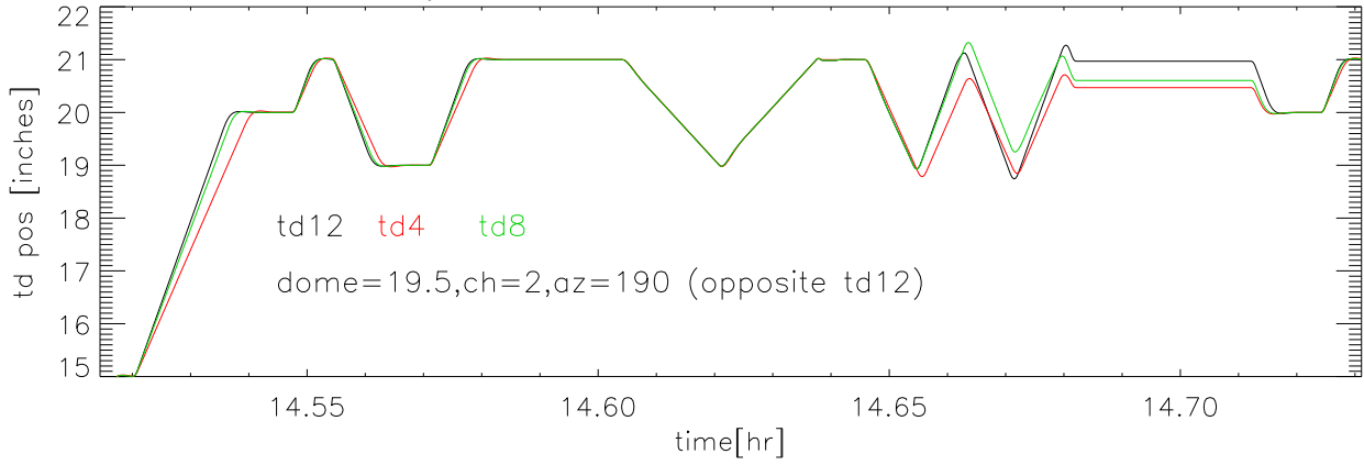
tieDown Vel (from encoder)
