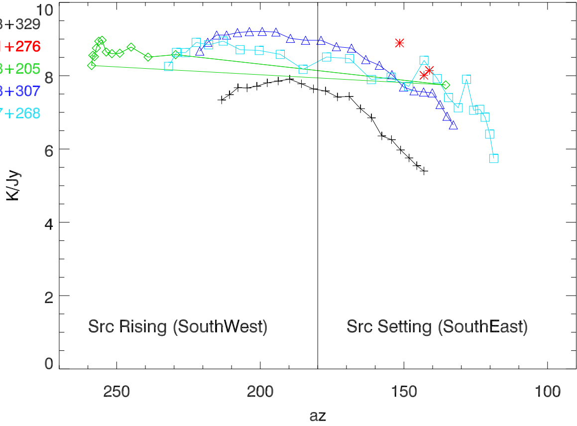
gain K/Jy vs azimuth (feed in South)
