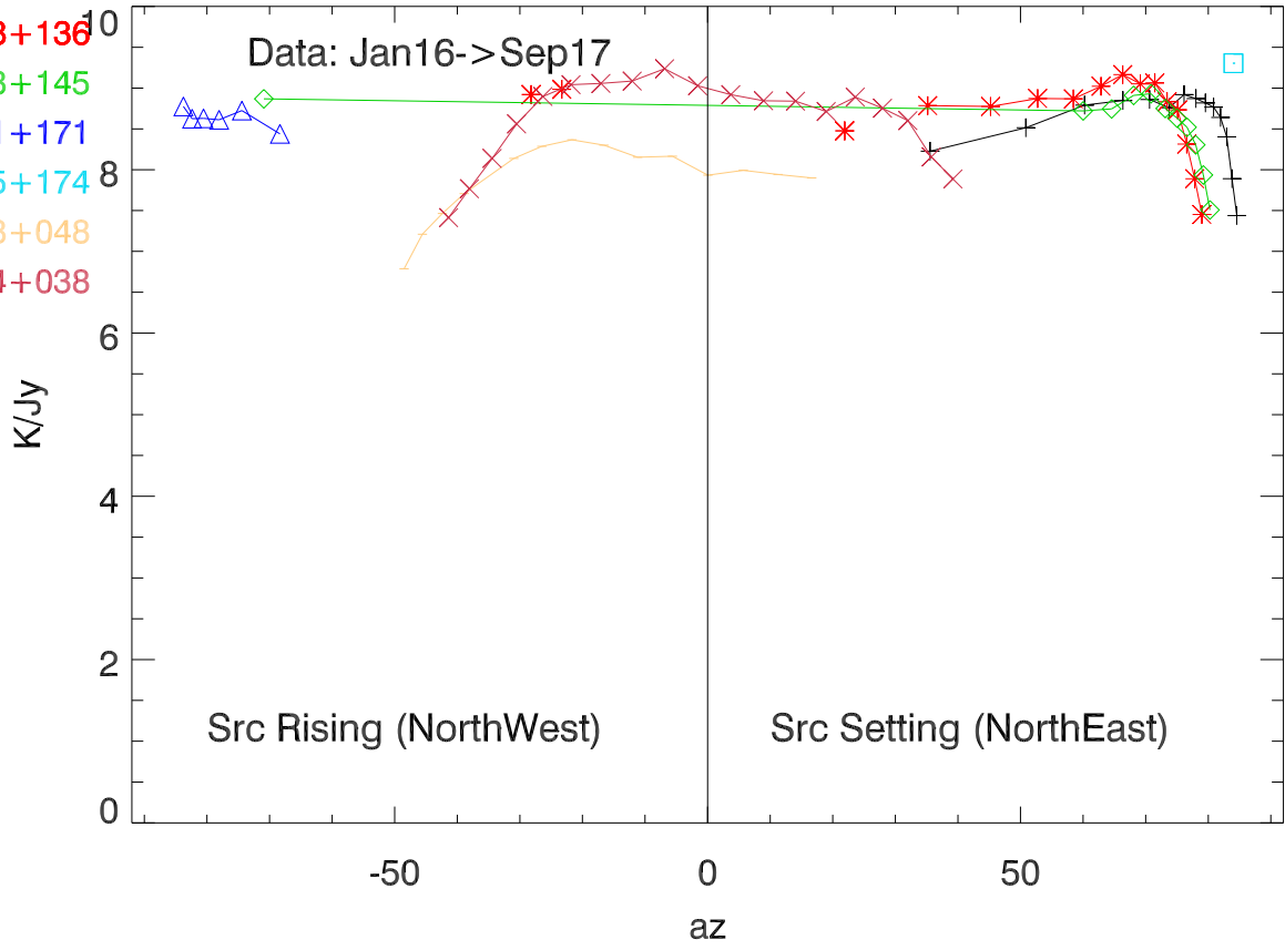
Gain (K/Jy) vs azimuth (feed in North). sbh
