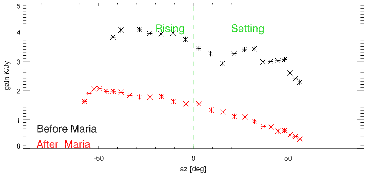
XBAND 9000 MHz src:B1328+307
