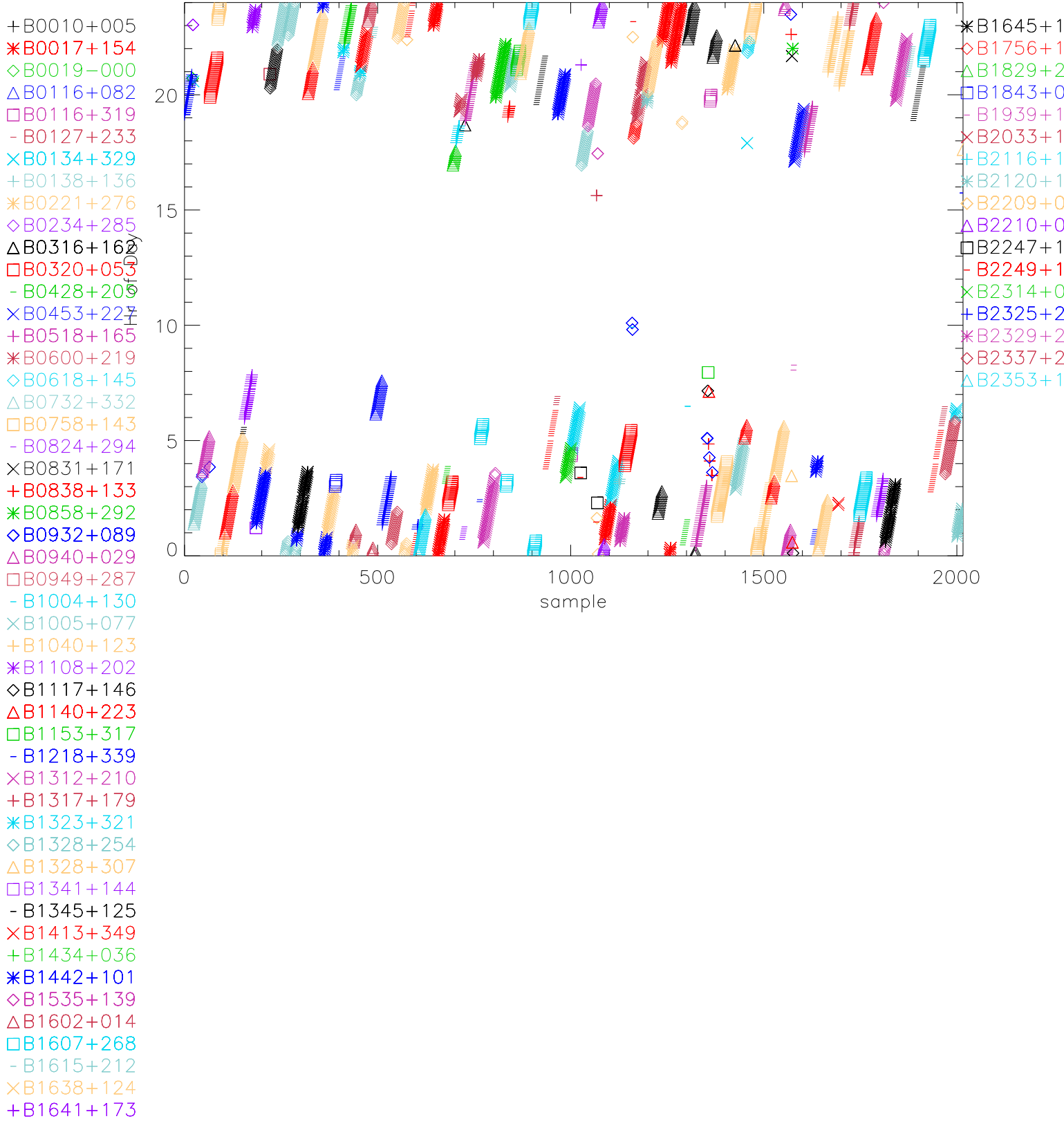
lbw hour of day for data
