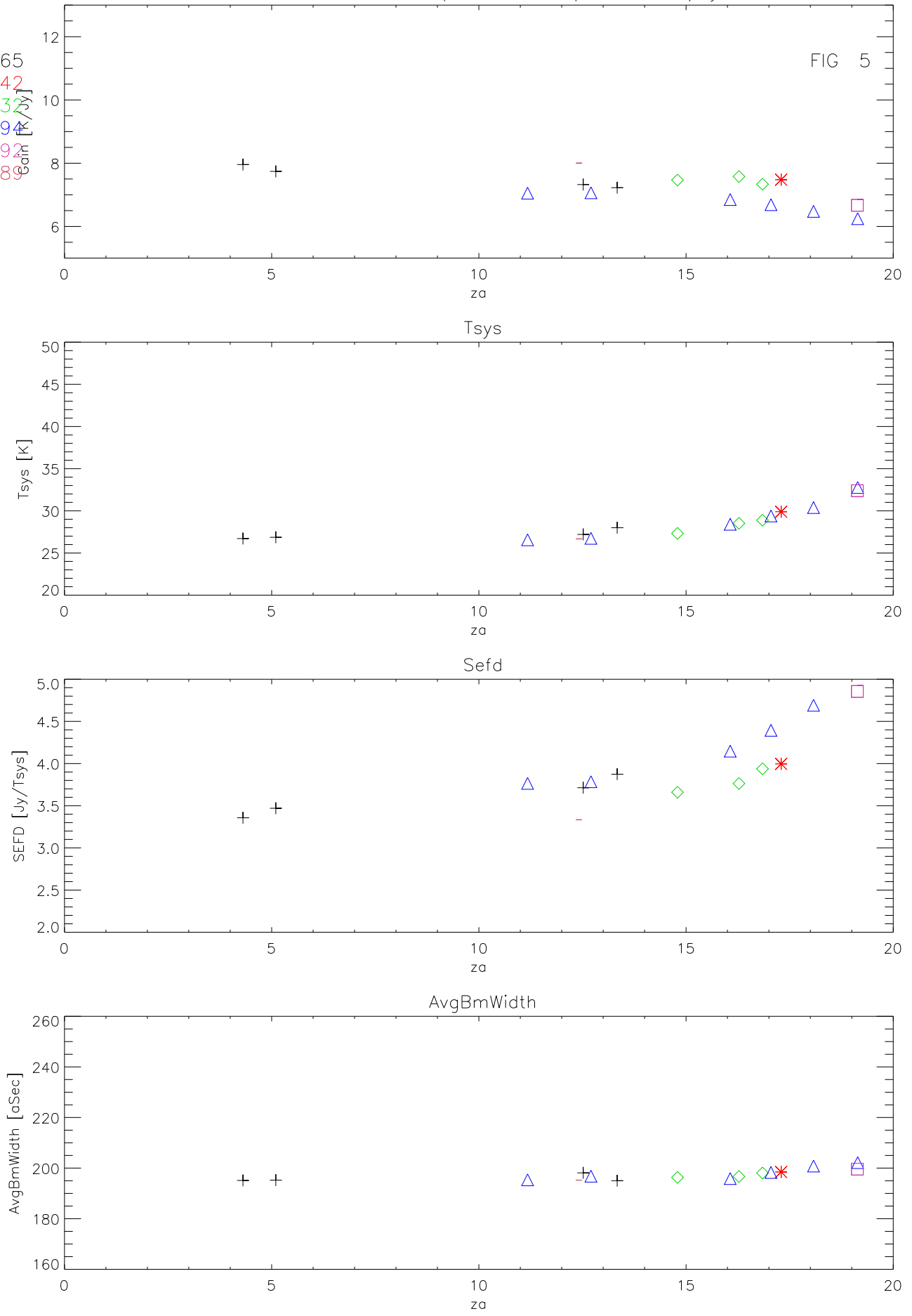
01oct11 to 31oct11 pixel 3 16 pnts. Gain K/Jy
