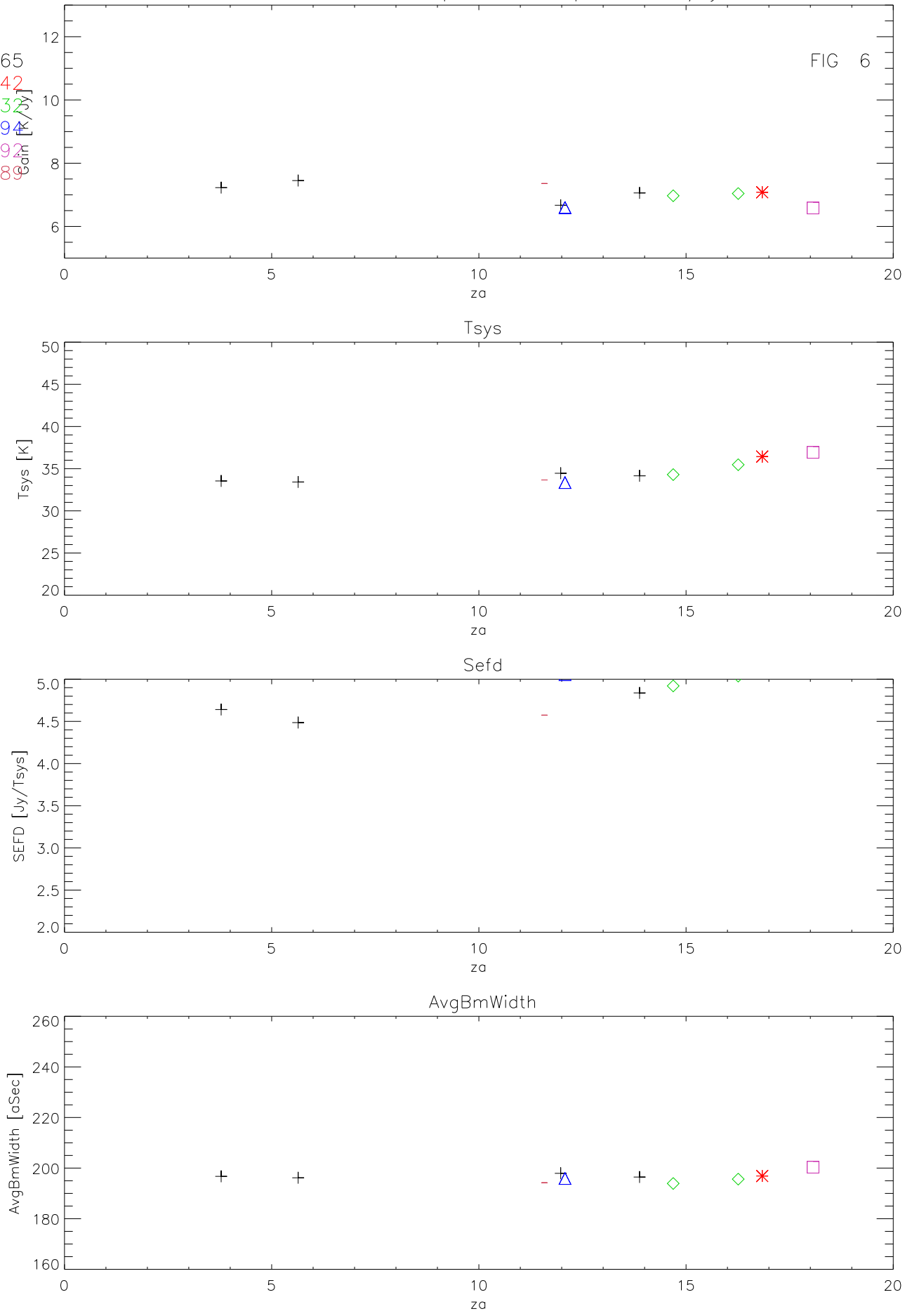
01oct11 to 31oct11 pixel 4 10 pnts. Gain K/Jy
