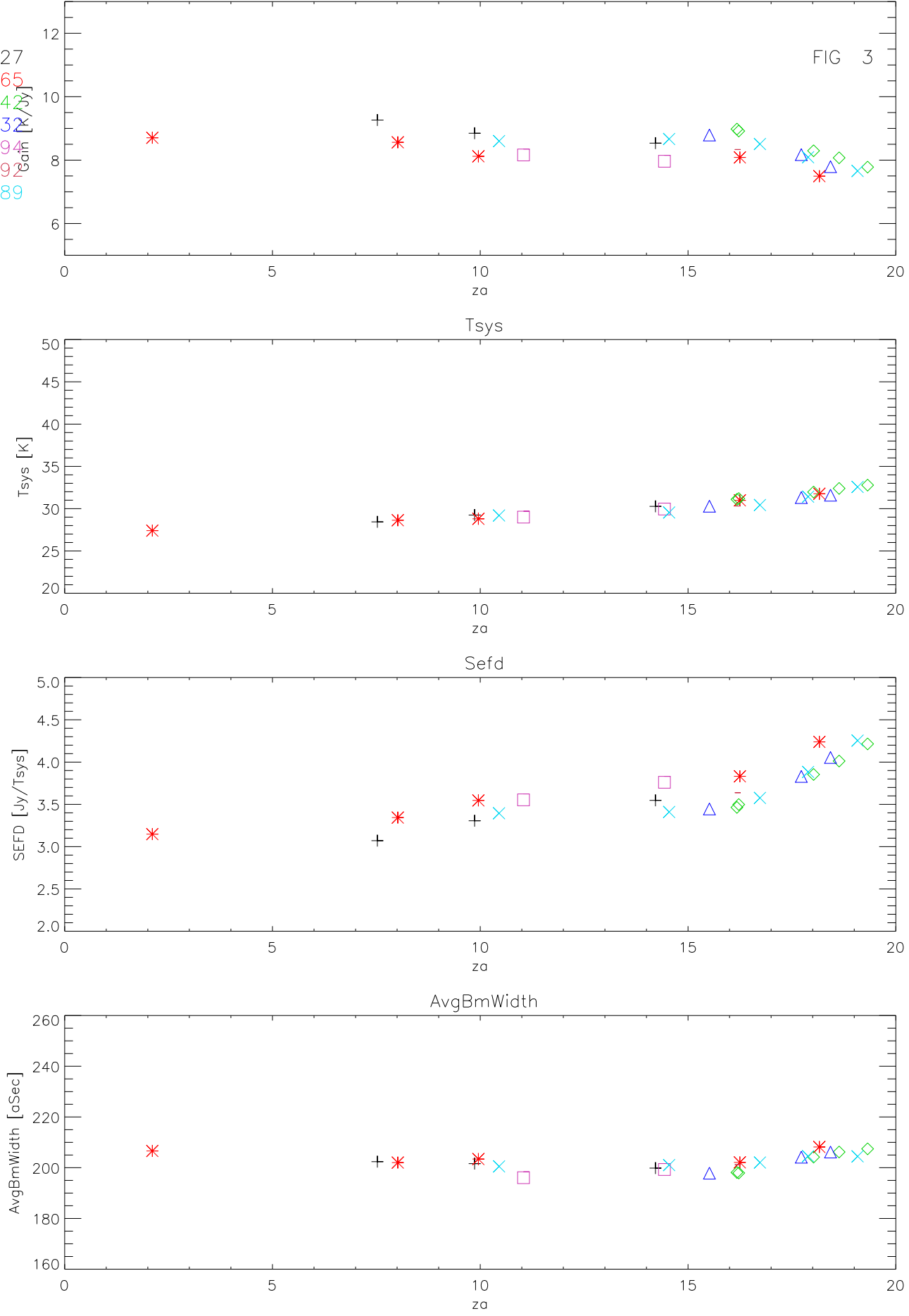
01oct11 to 31oct11 pixel 1 24 pnts. Gain K/Jy
