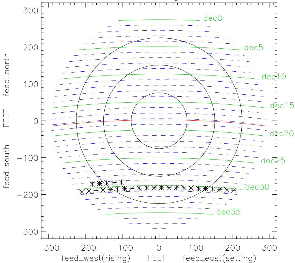
az,za coverage 327
