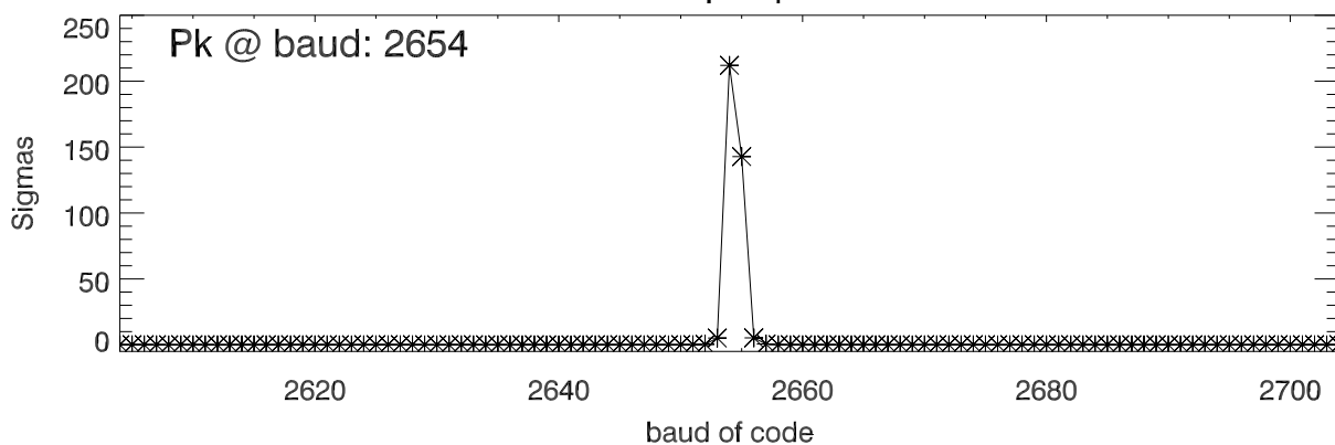
Blowup at peak
