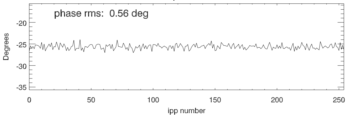
Phase of code peak vs code number
