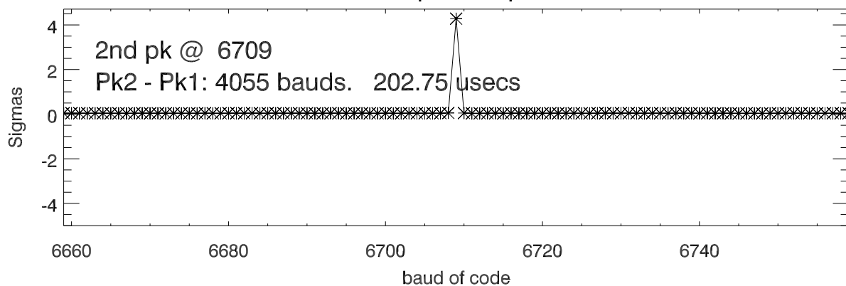
Blowup of 2nd peak
