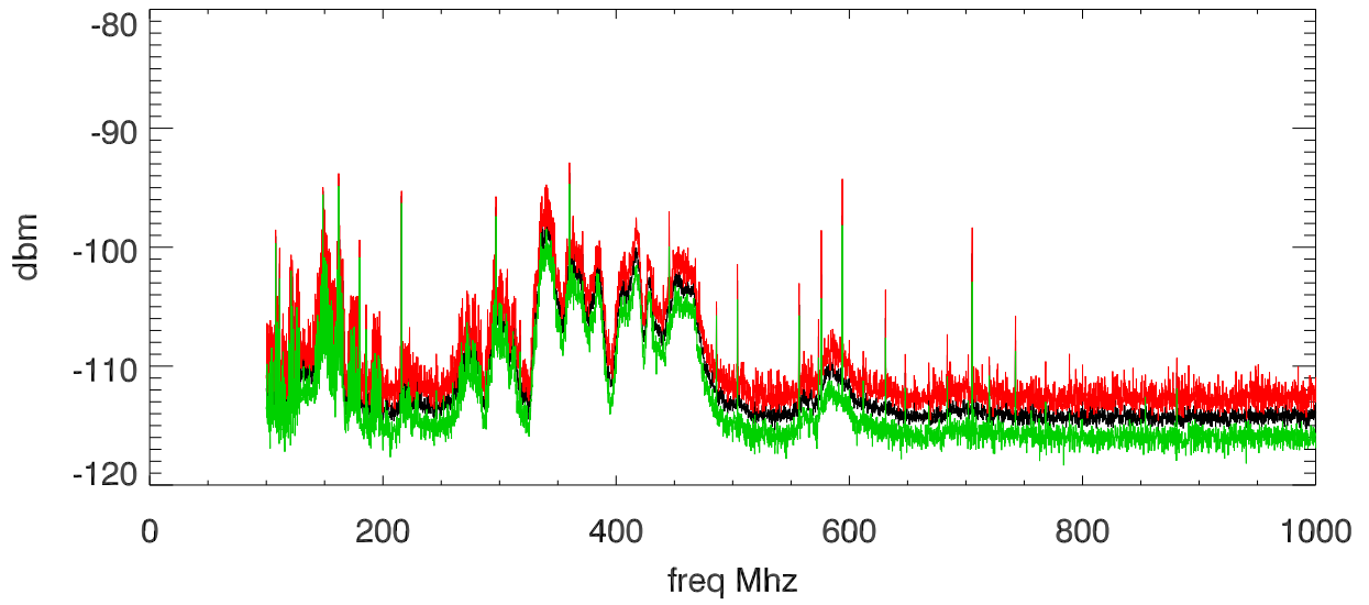
19Jan18 Site Cameras with Linear Supply (Eprobe)
