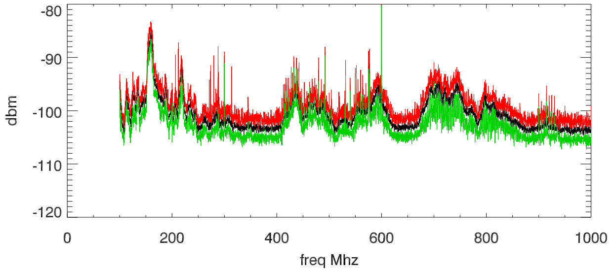
23May18 Site Cameras Model Axis P3227-LV (Eprobe)
