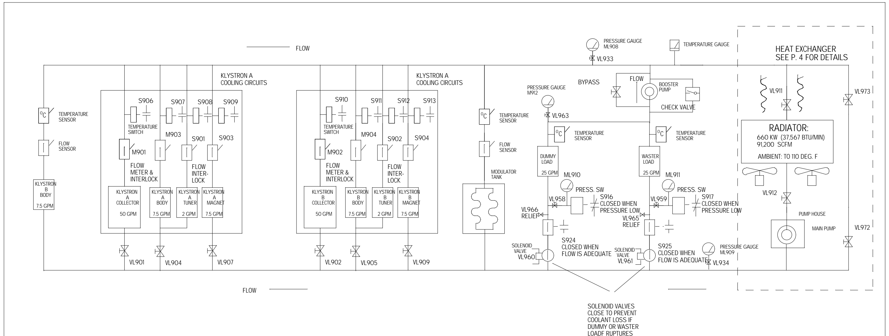
430 TRANSMITTER BLOCK DIAGRAM PAGE 3 OF 3: COOLING SYSTEM
