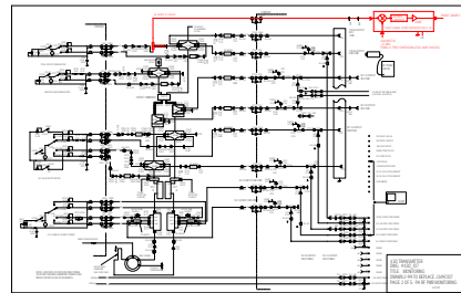
PA RF METERING
