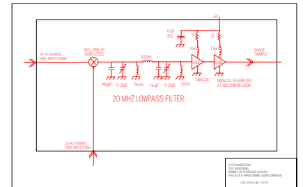
PHASE SAMPLE DOWN CONVERTER
