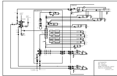
IPA AND CONSOLE METERING
