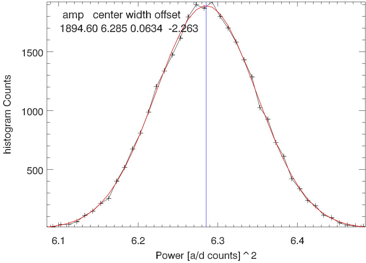
Gauss fit to histogram of multiBit simulated caloff power
