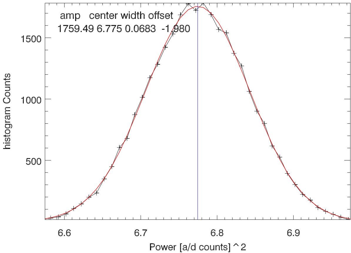
Gauss fit to histogram of simulated calon power
