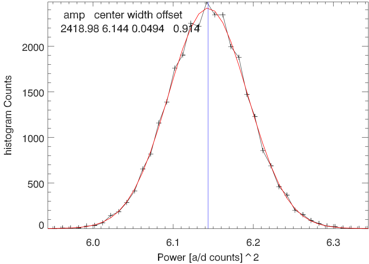
Gauss fit to histogram of 2bit simulated caloff power
