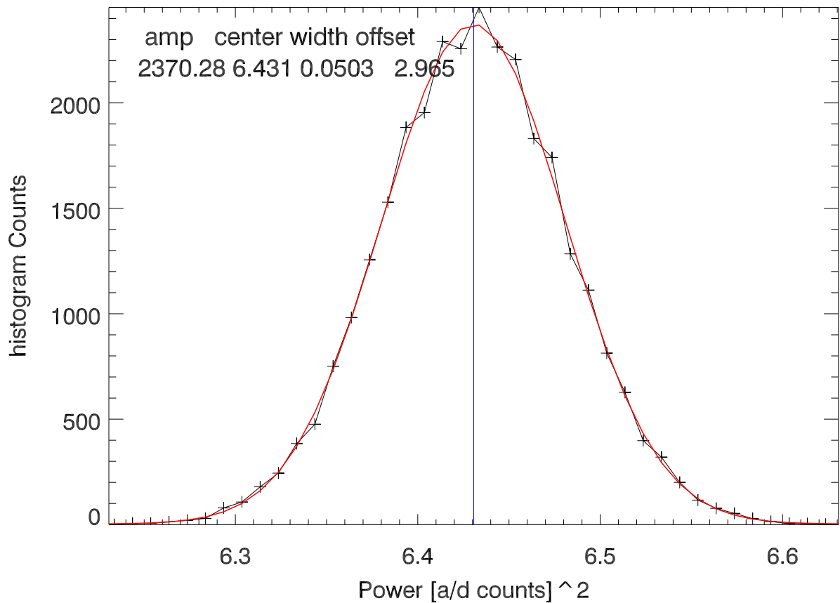
Gauss fit to histogram of 2bit simulated calon power
