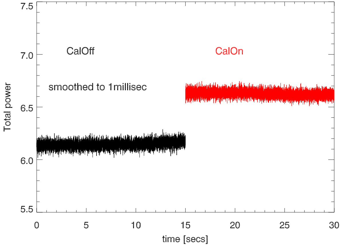
total power vs time (deviceUnits)
