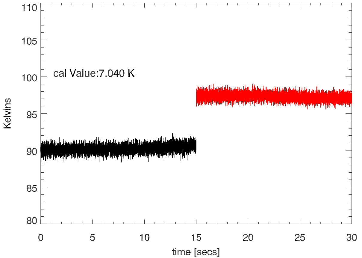
total power vs time (Kelvins)
