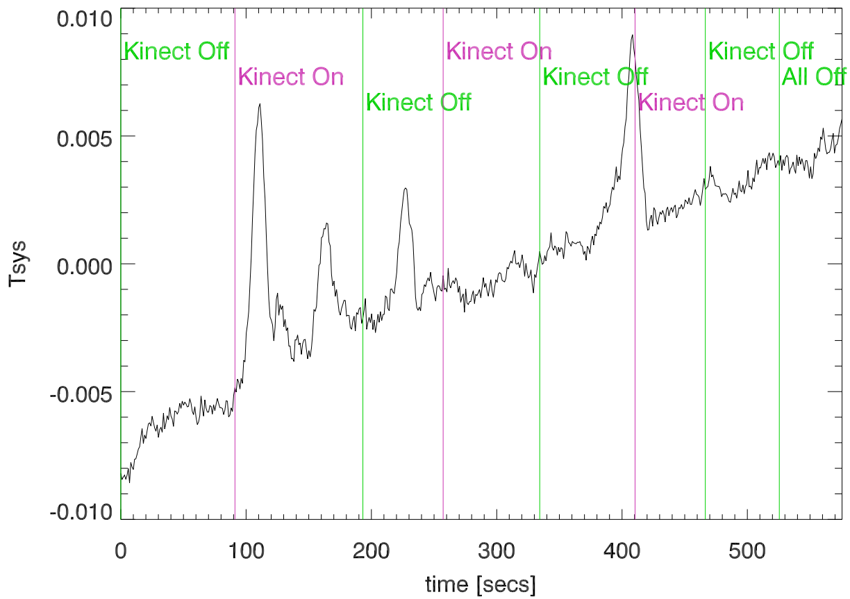
Total Pwr (1650.1 to 1670. Mhz) vs time
